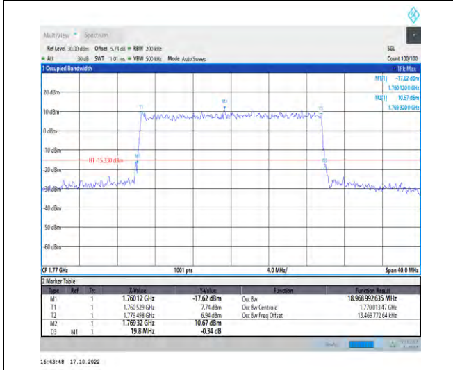
1-N66-PC3-15-20-H-8-CP-64QAM-Outer_Full-106@0 -Ant1-18.969-19.800-≤20-PASS
