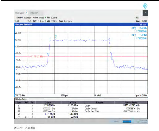
1-N66-PC3-15-10-H-4-DFT-64QAM-Outer_Full-50@0-Ant1-8.911-9.600-≤10-PASS
