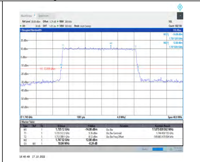
1-N66-PC3-15-20-M-3-DFT-16QAM-Outer_Full-100 @0-Ant1-17.876-18.840-≤20-PASS
