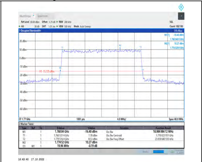
1-N66-PC3-15-20-H-7-CP-16QAM-Outer_Full-106@0 -Ant1-18.985-19.960-≤20-PASS
