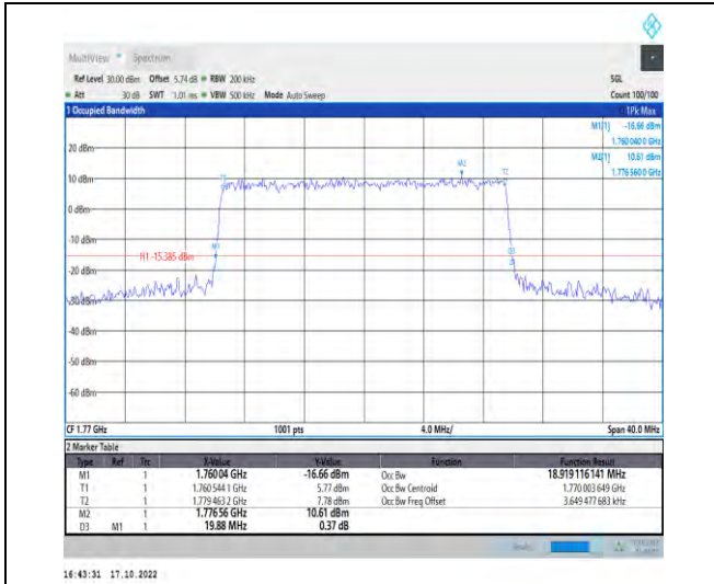
1-N66-PC3-15-20-H-6-CP-QPSK-Outer_Full-106@0 -Ant1-18.919-19.880-≤20-PASS
