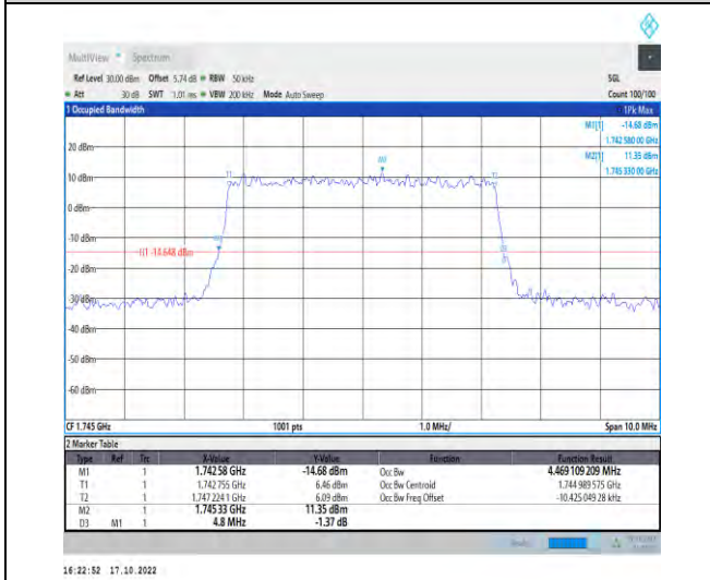
1-N66-PC3-15-5-M-4-DFT-64QAM-Outer_Full-25@0-Ant1-4.469-4.800-≤5-PASS
