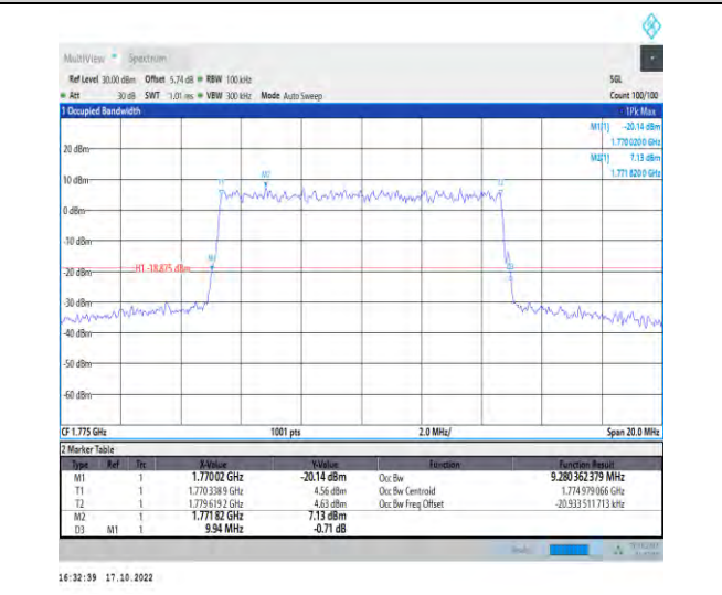
1-N66-PC3-15-10-H-9-CP-256QAM-Outer_Full-52@0-Ant1-9.28-9.940-≤10-PASS
