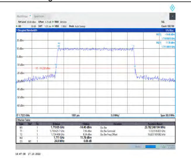
1-N66-PC3-15-25-L-7-CP-16QAM-Outer_Full-133@0 -Ant1-23.782-24.800-≤25-PASS
