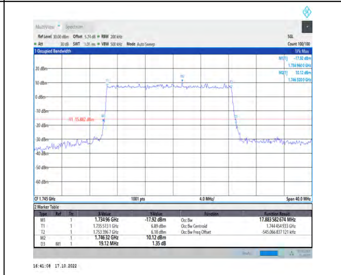
1-N66-PC3-15-20-M-5-DFT-256QAM-Outer_Full-100 @0-Ant1-17.884-19.120-≤20-PASS
