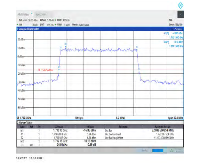
1-N66-PC3-15-25-L-5-DFT-256QAM-Outer_Full-128 @0-Ant1-22.839-24.000-≤25-PASS
