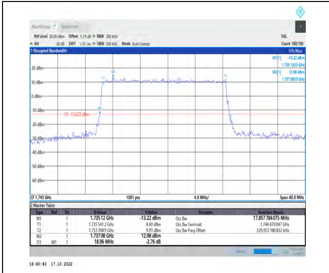
1-N66-PC3-15-20-M-1-DFT-QPSK-Outer_Full-100@ 0-Ant1-17.858-18.960-≤20-PASS
