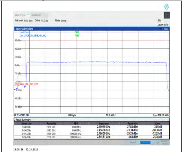
1-N41-PC2-30-100-L-3-DFT-PI2BPSK-Outer_Full-270@0-Ant1-1--PASS-see graph
