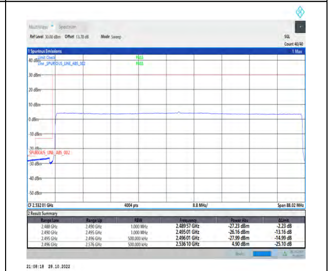
1-N41-PC2-30-80-L-6-CP-QPSK-Outer_Full-217@0-Ant1-1--PASS-see graph
