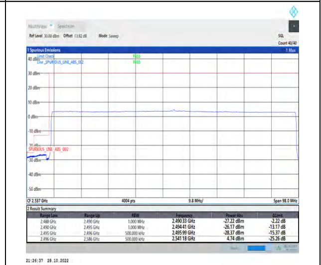
1-N41-PC2-30-90-L-6-CP-QPSK-Outer_Full-245@0-Ant1-1--PASS-see graph
