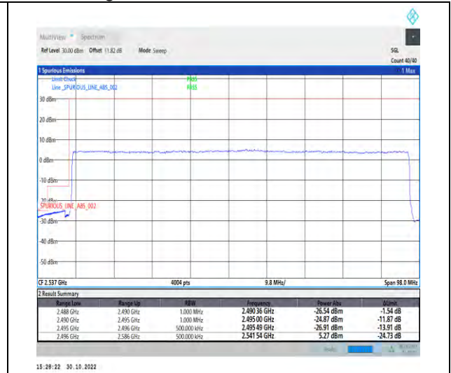
1-N41-PC2-30-90-L-3-DFT-PI2BPSK-Outer_Full-240@0-Ant1-1--PASS-see graph
