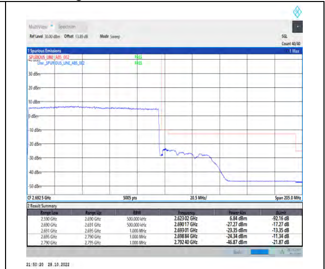
1-N41-PC2-30-100-H-3-DFT-PI2BPSK-Outer_Full-270@0-Ant1-1--PASS-see graph
