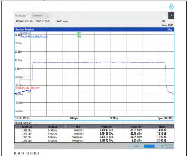
1-N41-PC2-30-70-L-3-DFT-PI2BPSK-Outer_Full-180@0-Ant1-1--PASS-see graph
