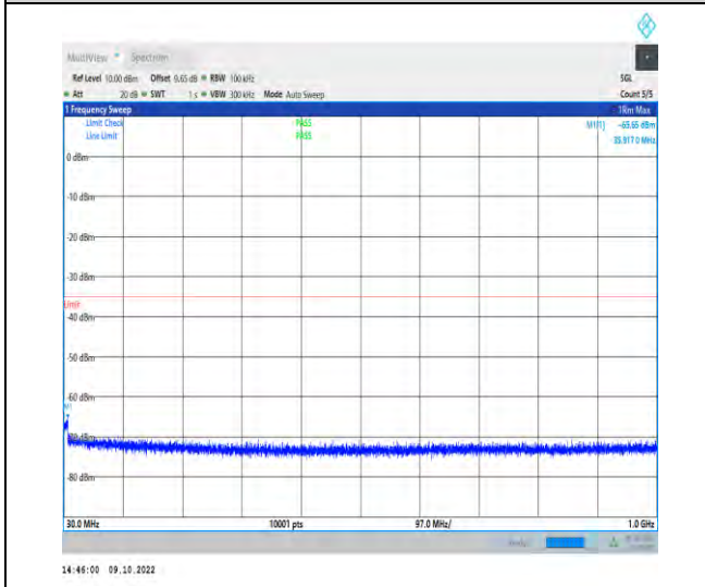
1-N41-PC2-30-100-H-1-DFT-QPSK-Edge_1RB_Left -1@0-30-1000-Ant1-35.92--65.65--35-PASS
