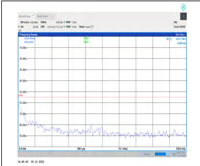
1-N41-PC2-30-100-H-1-DFT-QPSK-Edge_1RB_Left -1@0-0.009-0.15-Ant1-0.01--63.21--55-PASS
