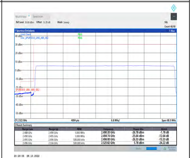
1-N41-PC2-30-60-L-6-CP-QPSK-Outer_Full-162@0-Ant1-1--PASS-see graph
