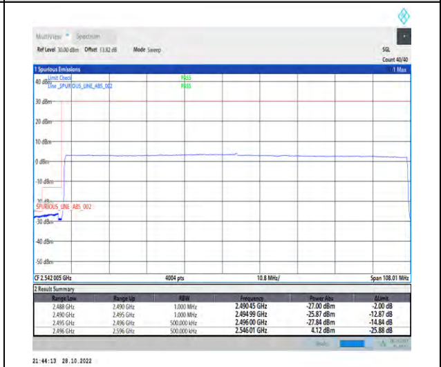
1-N41-PC2-30-100-L-6-CP-QPSK-Outer_Full-273@0-Ant1-1--PASS-see graph
