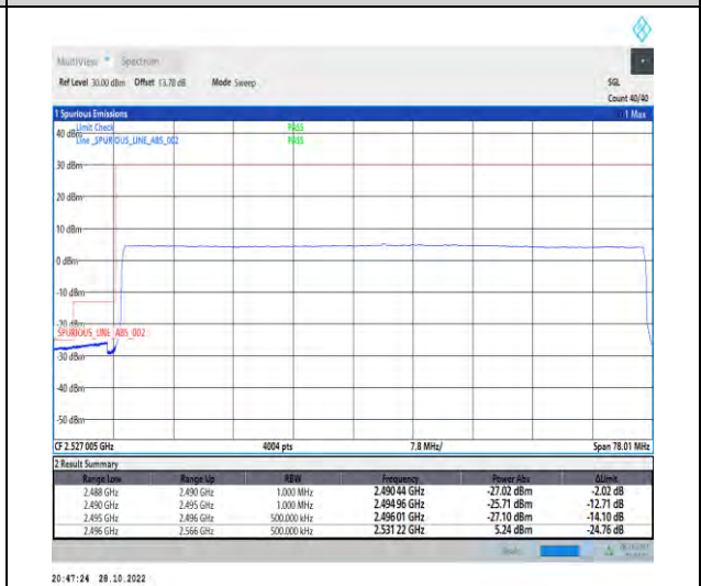
1-N41-PC2-30-70-L-6-CP-QPSK-Outer_Full-189@0-Ant1-1--PASS-see graph
