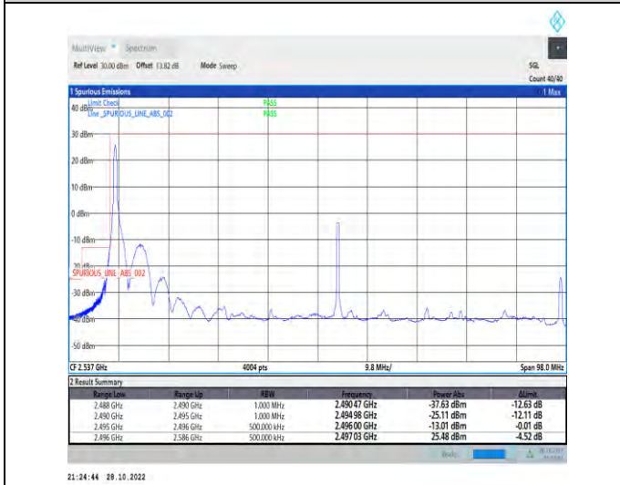
1-N41-PC2-30-90-L-4-CP-QPSK-Edge_1RB_Left-1@0-Ant1-1--PASS-see graph
