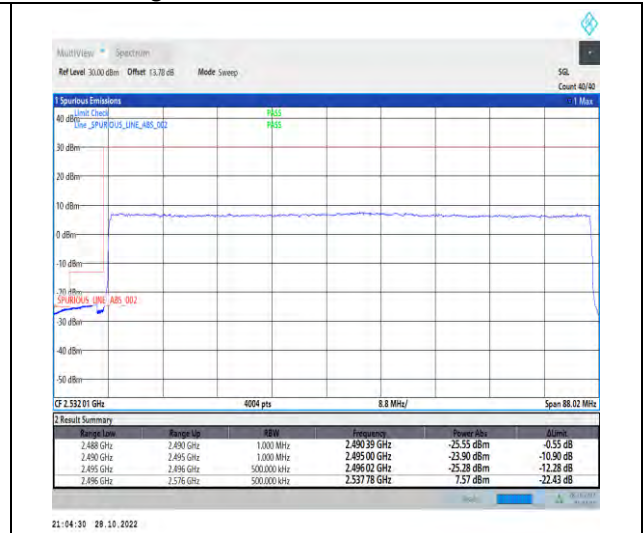
1-N41-PC2-30-80-L-3-DFT-PI2BPSK-Outer_Full-216@0-Ant1-1--PASS-see graph
