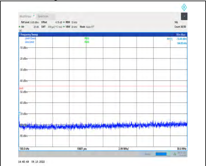
1-N41-PC2-30-100-H-1-DFT-QPSK-Edge_1RB_Left -1@0-0.15-30-Ant1-0.16--72.48--45-PASS
