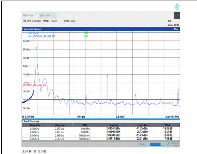
1-N41-PC2-30-90-L-1-DFT-PI2BPSK-Edge_1RB_Left-1@0-Ant1-1--PASS-see graph
