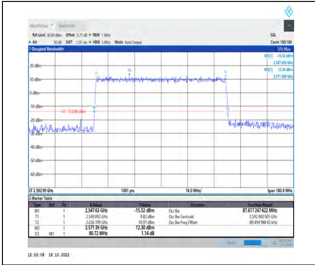
1-N41-PC2-30-90-M-6-CP-QPSK-Outer_Full-245@0-Ant1-87.617-90.720-≤90-PASS
