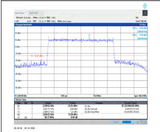
1-N41-PC2-30-90-H-8-CP-64QAM-Outer_Full-245@0 -Ant1-87.226-90.720-<=90-PASS
