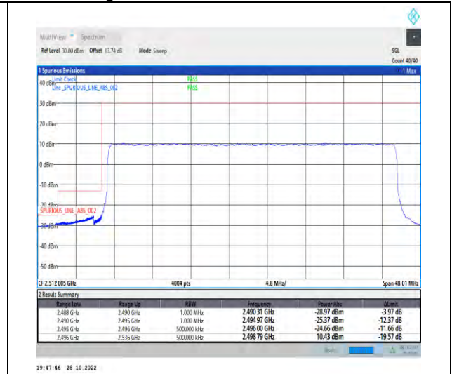
1-N41-PC2-30-40-L-3-DFT-PI2BPSK-Outer_Full-100@0-Ant1-1--PASS-see graph
