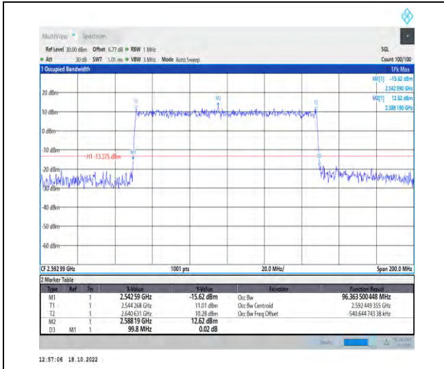
1-N41-PC2-30-100-M-1-DFT-QPSK-Outer_Full-270 @0-Ant1-96.364-99.800-≤100-PASS
