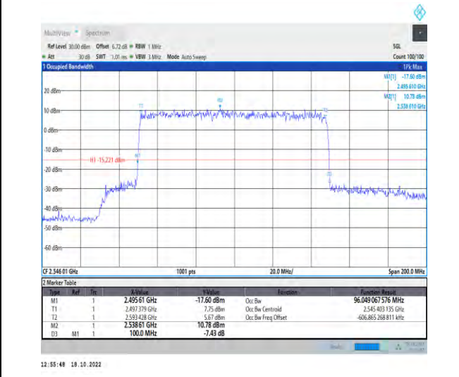
1-N41-PC2-30-100-L-5-DFT-256QAM-Outer_Full-270 @0-Ant1-96.049-100.000-≤100-PASS
