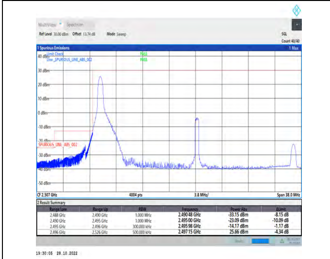
1-N41-PC2-30-30-L-4-CP-QPSK-Edge_1RB_Left-1@0-Ant1-1--PASS-see graph
