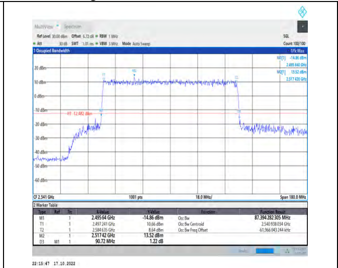
1-N41-PC2-30-90-L-7-CP-16QAM-Outer_Full-245@0 -Ant1-87.394-90.720-≤90-PASS
