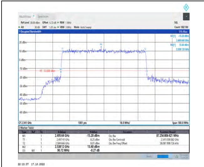
1-N41-PC2-30-90-L-6-CP-QPSK-Outer_Full-245@0 -Ant1-87.257-90.720-≤90-PASS
