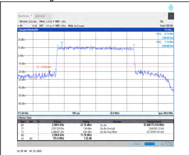
1-N41-PC2-30-100-H-7-CP-16QAM-Outer_Full-273 @0-Ant1-97.609-101.000-≤100-PASS
