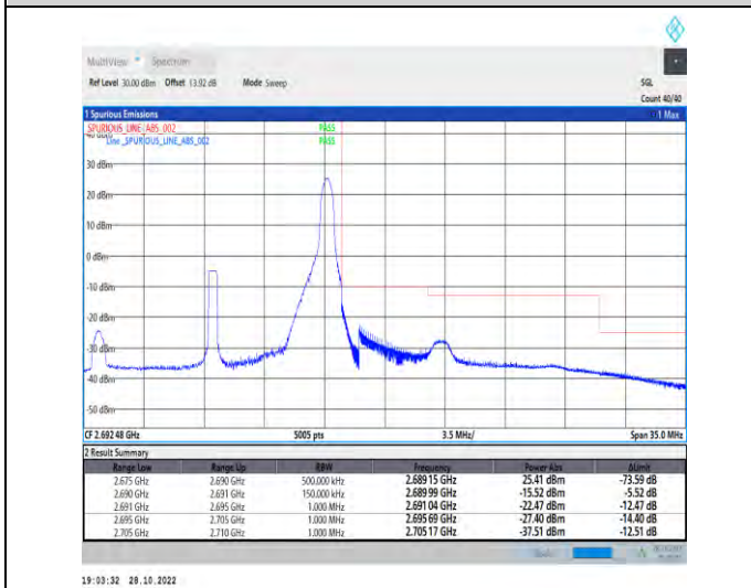
1-N41-PC2-30-15-H-5-CP-QPSK-Edge_1RB_Right-1@37-Ant1-1--PASS-see graph
