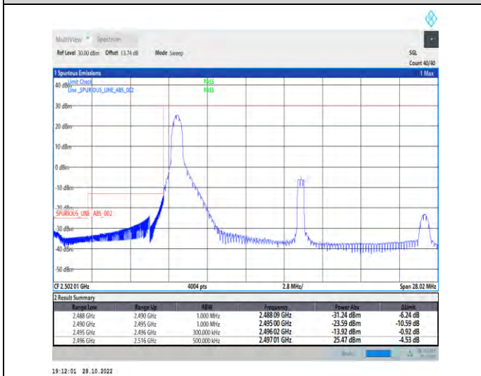
1-N41-PC2-30-20-L-4-CP-QPSK-Edge_1RB_Left-1@0-Ant1-1--PASS-see graph
