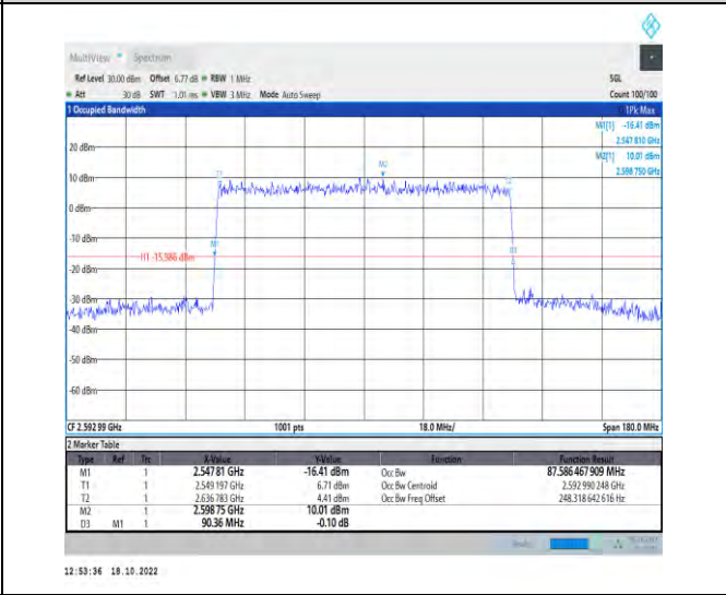
1-N41-PC2-30-90-M-9-CP-256QAM-Outer_Full-245@0-Ant1-87.586-90.360-≤90-PASS
