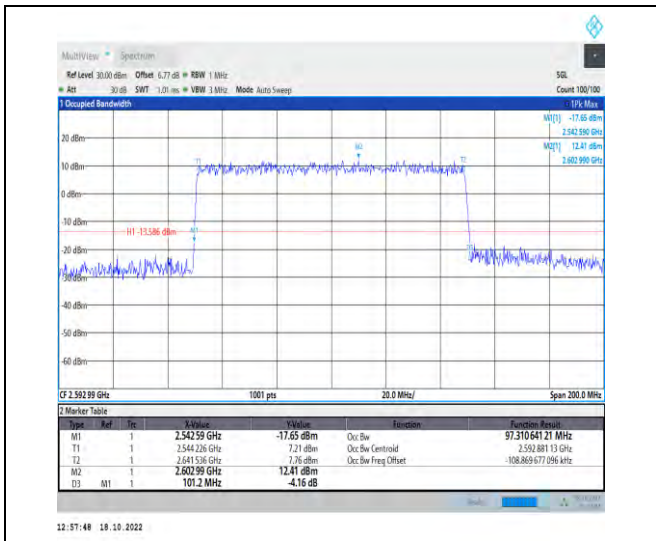
1-N41-PC2-30-100-M-6-CP-QPSK-Outer_Full-273 @0-Ant1-97.311-101.200-≤100-PASS
