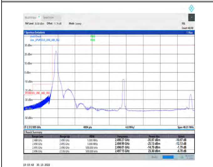
1-N41-PC2-30-40-L-4-CP-QPSK-Edge_1RB_Left-1@0-Ant1-1--PASS-see graph
