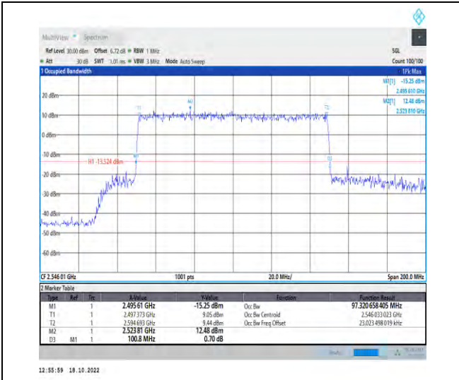
1-N41-PC2-30-100-L-6-CP-QPSK-Outer_Full-273@ 0-Ant1-97.321-100.800-≤100-PASS
