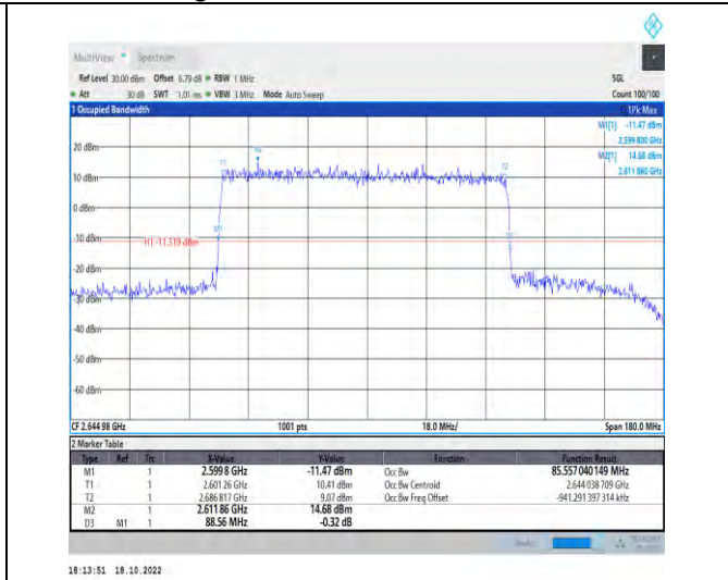
1-N41-PC2-30-90-H-3-DFT-16QAM-Outer_Full-240 @0-Ant1-85.557-88.560-≤90-PASS
