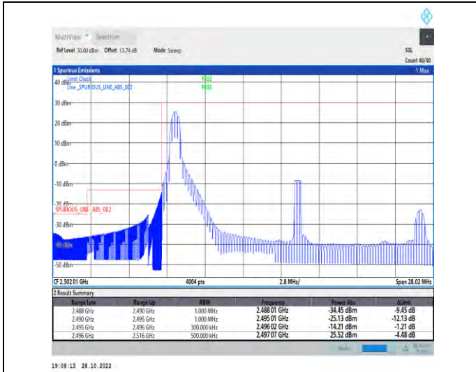
1-N41-PC2-30-20-L-1-DFT-PI2BPSK-Edge_1RB_Left-1@0-Ant1-1--PASS-see graph
