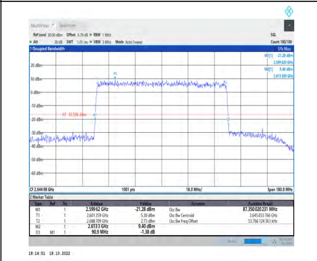
1-N41-PC2-30-90-H-9-CP-256QAM-Outer_Full-245@0 -Ant1-87.35-90.900-<=90-PASS
