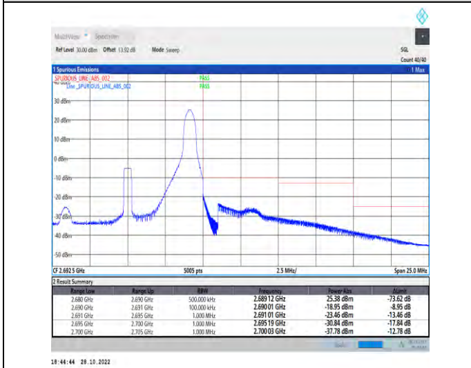
1-N41-PC2-30-10-H-5-CP-QPSK-Edge_1RB_Right-1@23-Ant1-1--PASS-see graph
