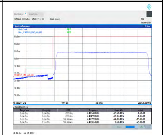
1-N41-PC2-30-20-L-6-CP-QPSK-Outer_Full-51@0-Ant1-1--PASS-see graph
