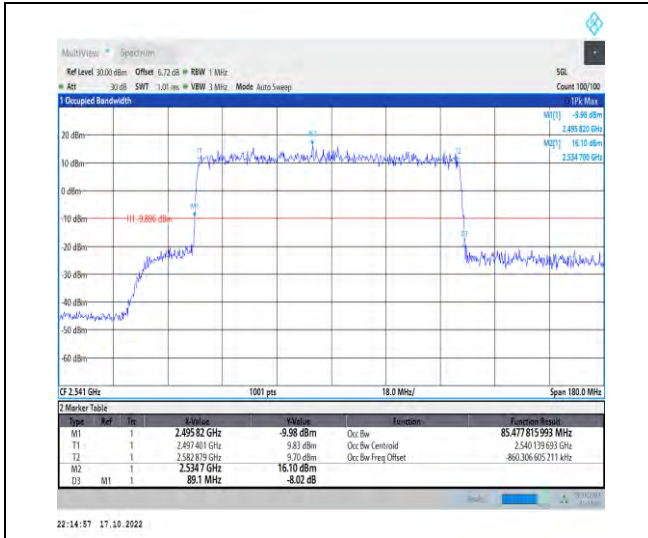
1-N41-PC2-30-90-L-1-DFT-QPSK-Outer_Full-240@ 0-Ant1-85.478-89.100-≤90-PASS
