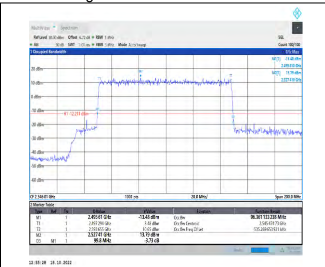
1-N41-PC2-30-100-L-3-DFT-16QAM-Outer_Full-270 @0-Ant1-96.361-99.800-≤100-PASS
