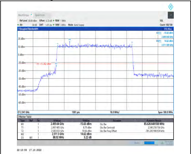
1-N41-PC2-30-90-L-3-DFT-16QAM-Outer_Full-240@ 0-Ant1-85.627-88.920-≤90-PASS
