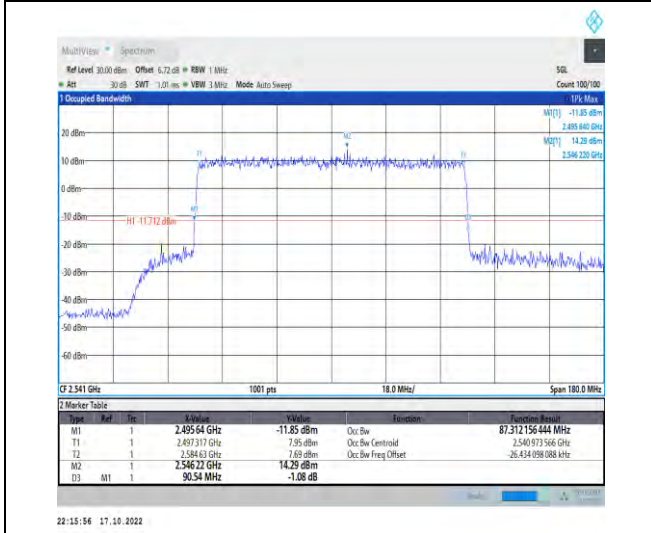
1-N41-PC2-30-90-L-8-CP-64QAM-Outer_Full-245@0 -Ant1-87.312-90.540-≤90-PASS
