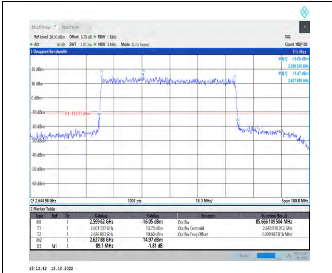
1-N41-PC2-30-90-H-1-DFT-QPSK-Outer_Full-240@ 0-Ant1-85.666-89.100-≤90-PASS
