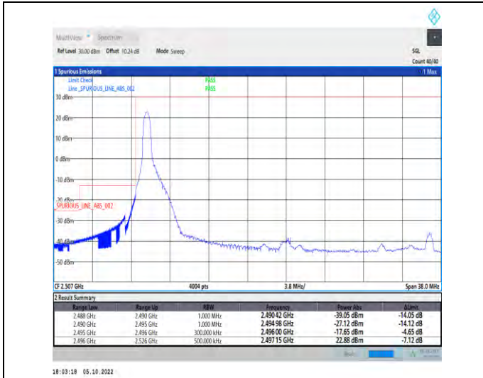
1-N41-PC2-30-30-L-1-DFT-PI2BPSK-Edge_1RB_Left-1@0-Ant1-1--PASS-see graph
