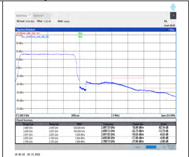
1-N41-PC2-30-10-H-3-DFT-PI2BPSK-Outer_Full-24@0-Ant1-1--PASS-see graph
