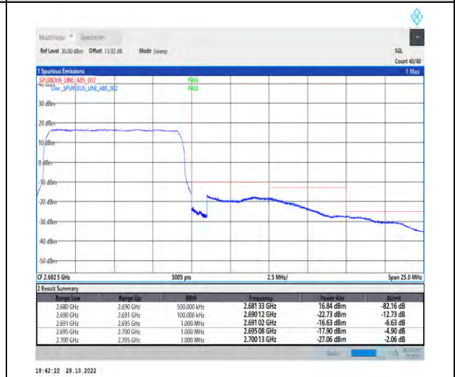
1-N41-PC2-30-10-H-6-CP-QPSK-Outer_Full-24@0-Ant1-1--PASS-see graph
