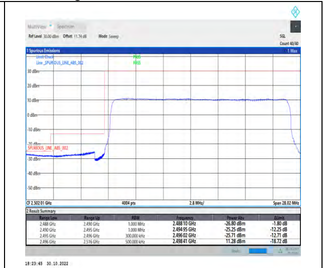
1-N41-PC2-30-20-L-3-DFT-PI2BPSK-Outer_Full-50@0-Ant1-1--PASS-see graph
