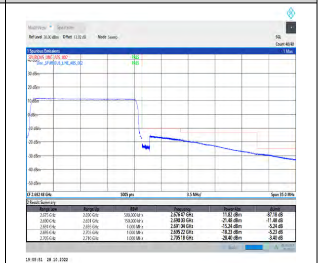
1-N41-PC2-30-15-H-6-CP-QPSK-Outer_Full-38@0-Ant1-1--PASS-see graph
