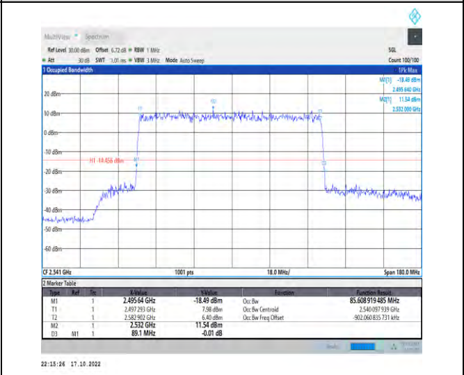
1-N41-PC2-30-90-L-5-DFT-256QAM-Outer_Full-240 @0-Ant1-85.609-89.100-≤90-PASS
