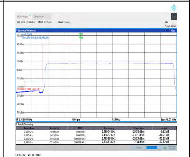
1-N41-PC2-30-40-L-6-CP-QPSK-Outer_Full-106@0-Ant1-1--PASS-see graph
