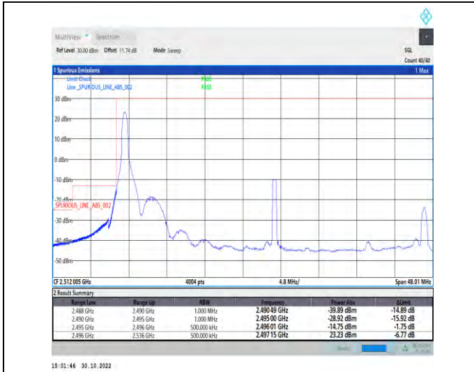
1-N41-PC2-30-40-L-1-DFT-PI2BPSK-Edge_1RB_Left-1@0-Ant1-1--PASS-see graph
