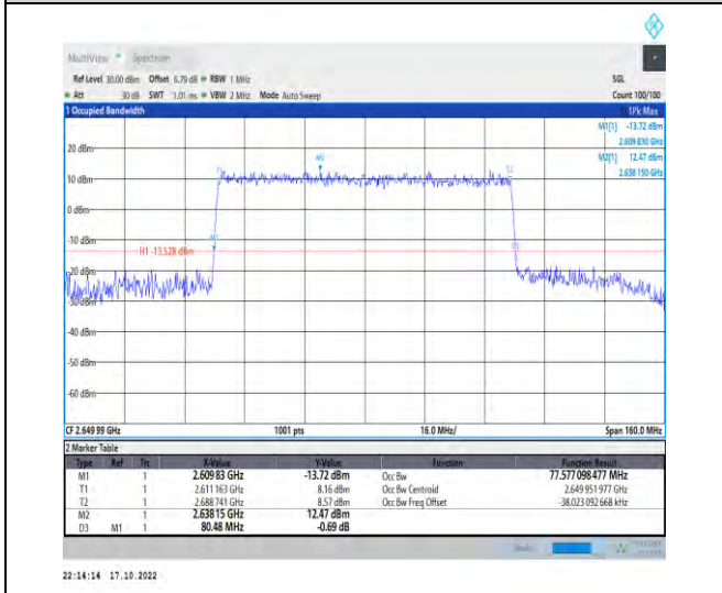
1-N41-PC2-30-80-H-8-CP-64QAM-Outer_Full-217@0 -Ant1-77.577-80.480-≤80-PASS
