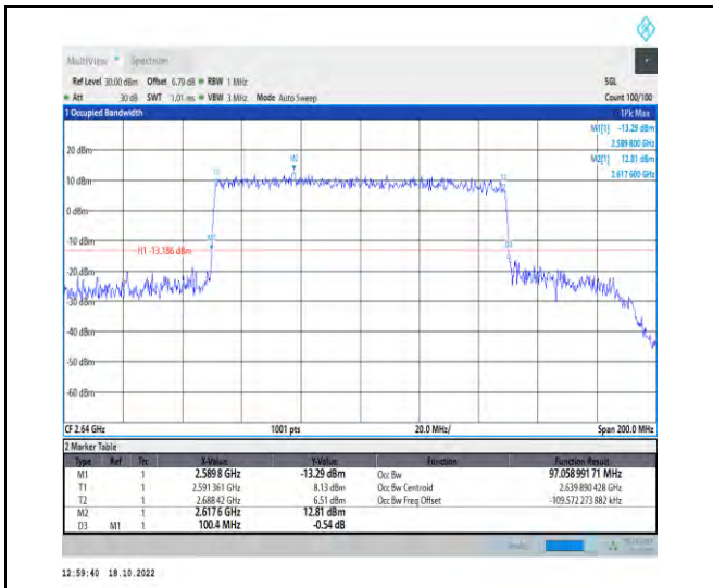
1-N41-PC2-30-100-H-6-CP-QPSK-Outer_Full-273@ 0-Ant1-97.059-100.400-≤100-PASS
