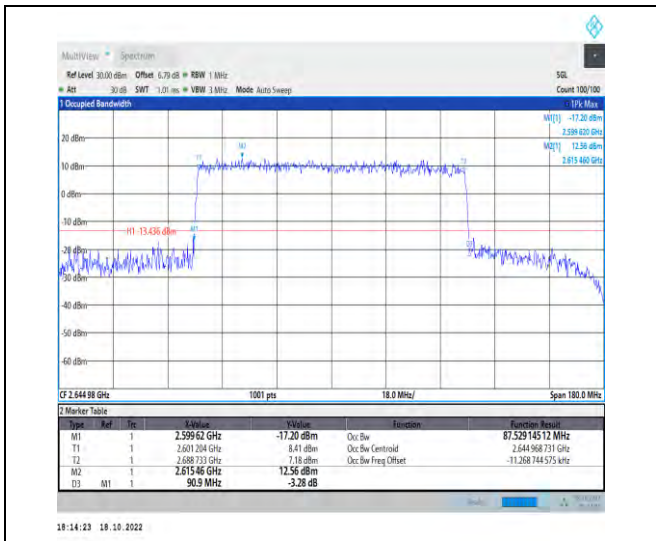
1-N41-PC2-30-90-H-6-CP-QPSK-Outer_Full-245@0 -Ant1-87.529-90.900-<=90-PASS
