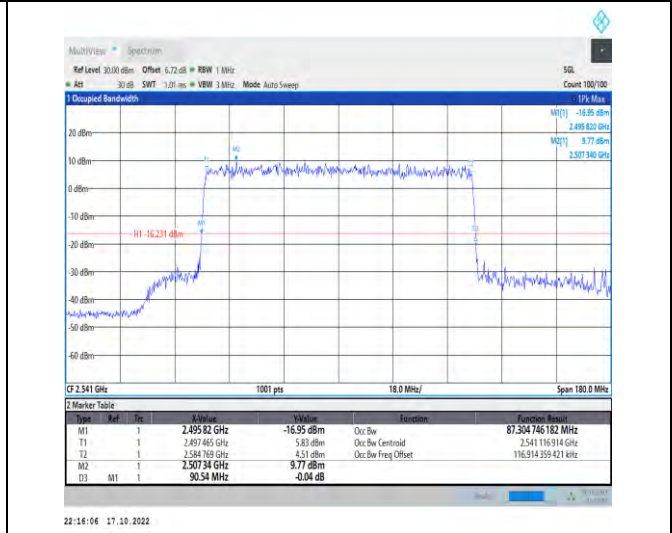
1-N41-PC2-30-90-L-9-CP-256QAM-Outer_Full-245@0 -Ant1-87.305-90.540-≤90-PASS
