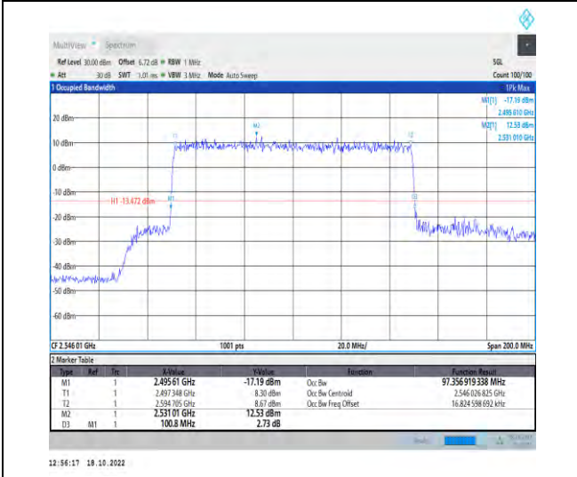
1-N41-PC2-30-100-L-8-CP-64QAM-Outer_Full-273 @0-Ant1-97.357-100.800-≤100-PASS
