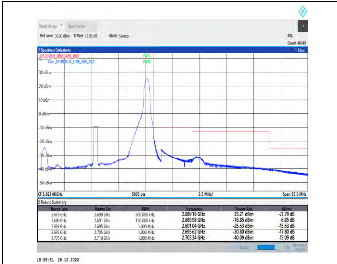
1-N41-PC2-30-15-H-2-DFT-PI2BPSK-Edge_1RB_Right-t-1@37-Ant1-1--PASS-see graph
