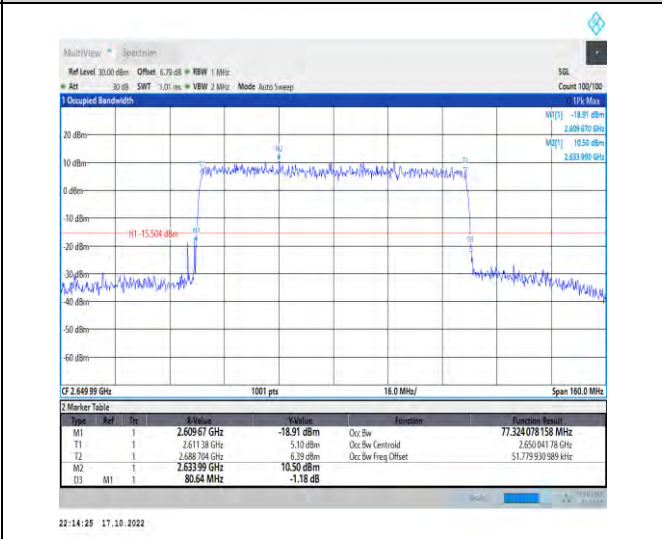
1-N41-PC2-30-80-H-9-CP-256QAM-Outer_Full-217@0 -Ant1-77.324-80.640-≤80-PASS
