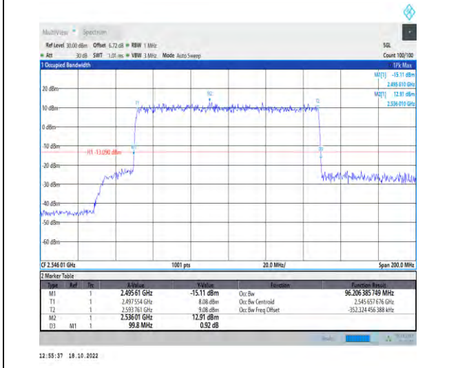
1-N41-PC2-30-100-L-4-DFT-64QAM-Outer_Full-270 @0-Ant1-96.206-99.800-≤100-PASS
