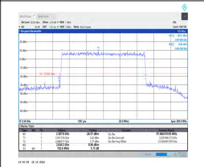
1-N41-PC2-30-100-H-9-CP-256QAM-Outer_Full-273 @0-Ant1-97.46-102.600-≤100-PASS
