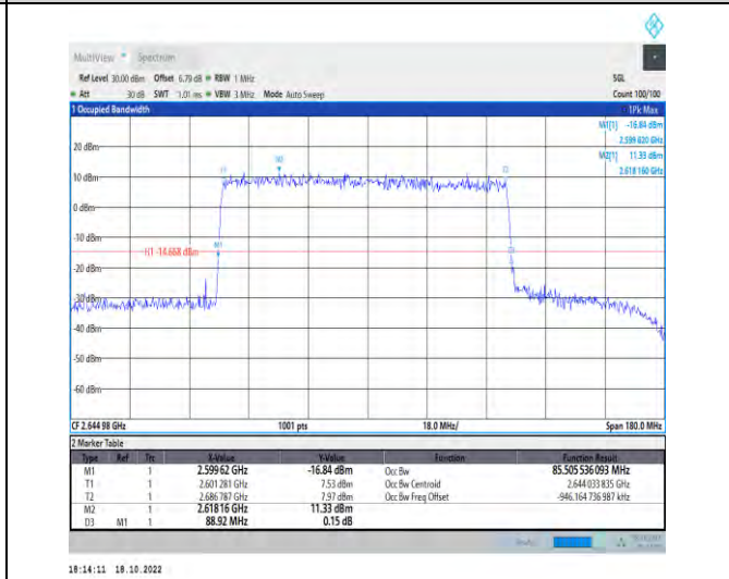
1-N41-PC2-30-90-H-5-DFT-256QAM-Outer_Full-240 @0-Ant1-85.506-88.920-≤90-PASS
