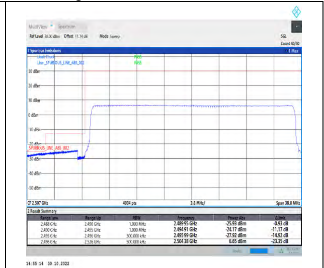
1-N41-PC2-30-30-L-3-DFT-PI2BPSK-Outer_Full-75@0-Ant1-1--PASS-see graph
