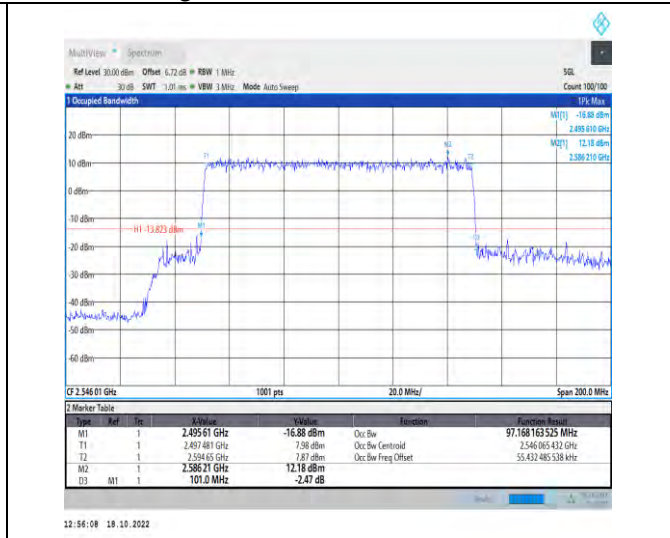
1-N41-PC2-30-100-L-7-CP-16QAM-Outer_Full-273@ 0-Ant1-97.168-101.000-≤100-PASS
