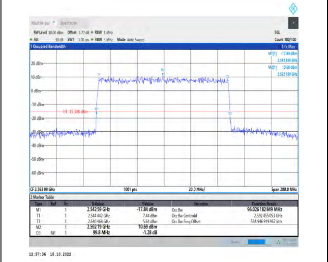
1-N41-PC2-30-100-M-5-DFT-256QAM-Outer_Full-27 @0-Ant1-96.026-99.800-≤100-PASS
