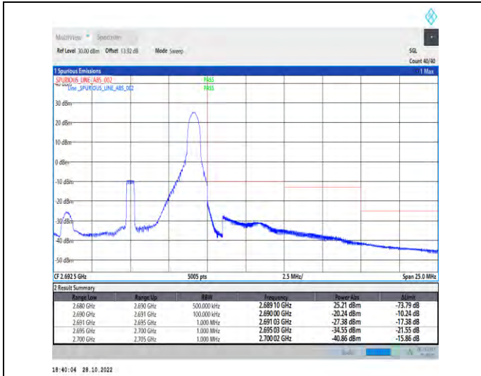
1-N41-PC2-30-10-H-2-DFT-PI2BPSK-Edge_1RB_Right-t-1@23-Ant1-1--PASS-see graph
