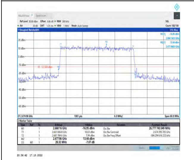
1-N41-PC2-30-30-H-4-DFT-64QAM-Outer_Full-75@0 -Ant1-26.778-28.320-≤30-PASS
