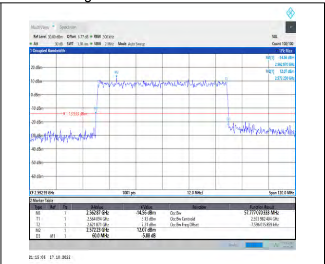
1-N41-PC2-30-60-M-7-CP-16QAM-Outer_Full-162@ 0-Ant1-57.777-60.000-≤60-PASS
