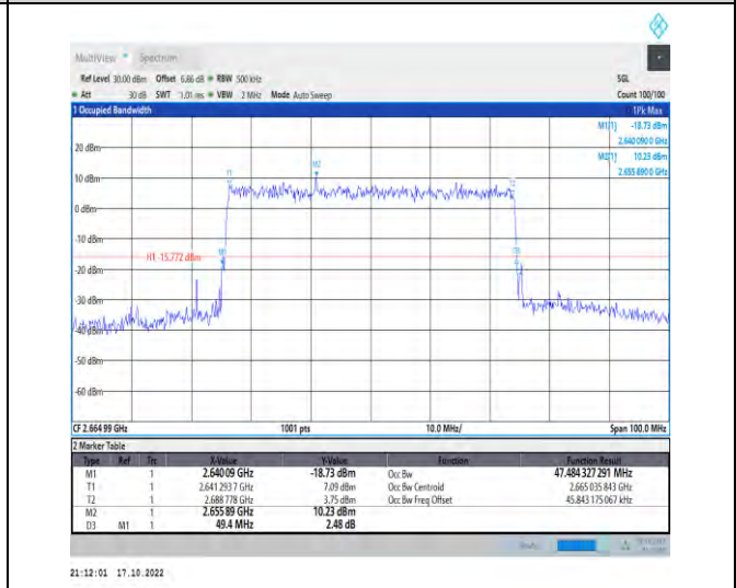
1-N41-PC2-30-50-H-9-CP-256QAM-Outer_Full-133@0 -Ant1-47.484-49.400-≤50-PASS
