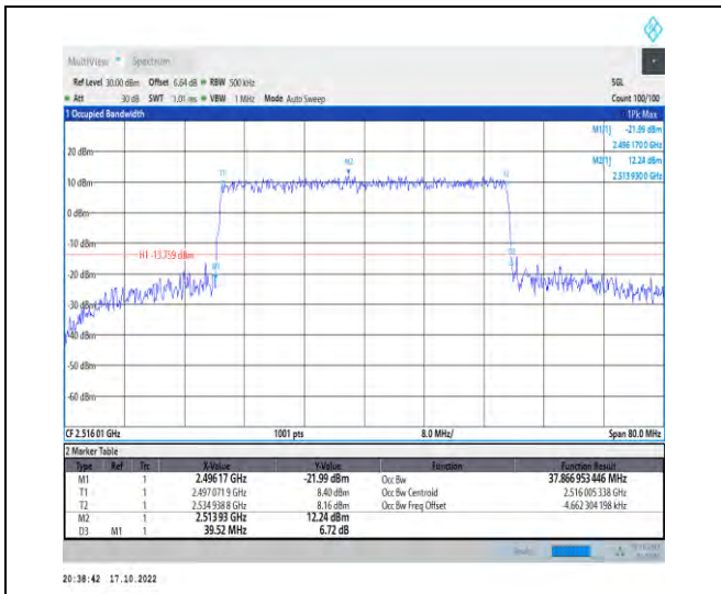
1-N41-PC2-30-40-L-6-CP-QPSK-Outer_Full-106@0 -Ant1-37.867-39.520-≤40-PASS
