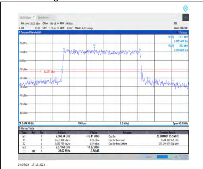
1-N41-PC2-30-30-H-3-DFT-16QAM-Outer_Full-75@0 -Ant1-26.809-28.020-≤30-PASS
