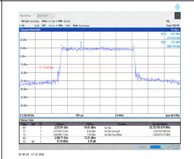
1-N41-PC2-30-40-M-5-DFT-256QAM-Outer_Full-100 @0-Ant1-35.754-37.760-≤40-PASS
