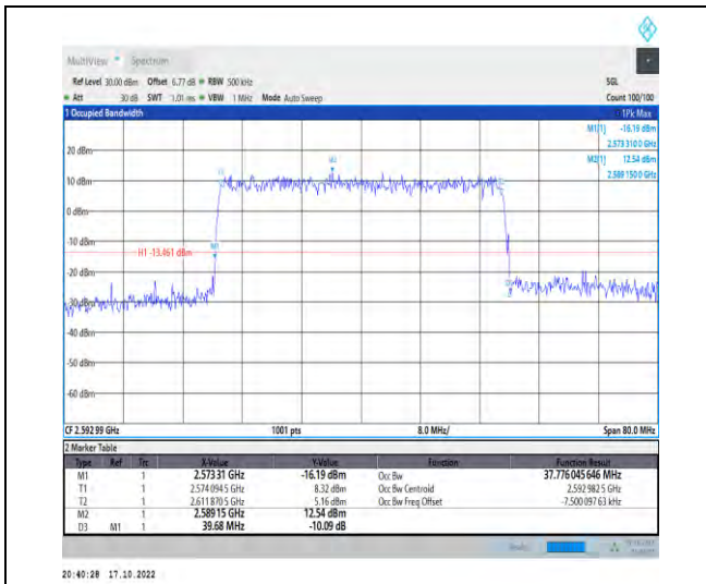
1-N41-PC2-30-40-M-6-CP-QPSK-Outer_Full-106@ 0-Ant1-37.776-39.680-≤40-PASS
