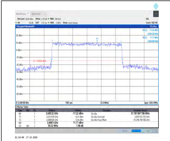
1-N41-PC2-30-60-H-6-CP-QPSK-Outer_Full-162@0 -Ant1-57.787-59.520-≤60-PASS
