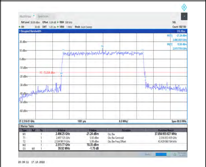
1-N41-PC2-30-40-L-9-CP-256QAM-Outer_Full-106@0 -Ant1-37.857-39.920-≤40-PASS
