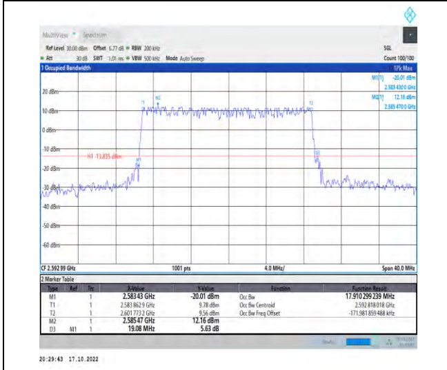
1-N41-PC2-30-20-M-4-DFT-64QAM-Outer_Full-50 @0-Ant1-17.91-19.080-<=20-PASS
