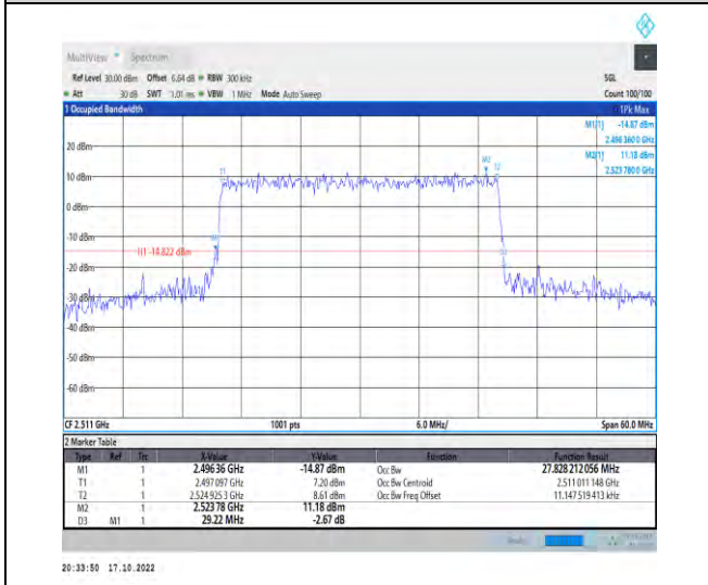
1-N41-PC2-30-30-L-8-CP-64QAM-Outer_Full-78@0-Ant1-27.828-29.220-≤30-PASS
