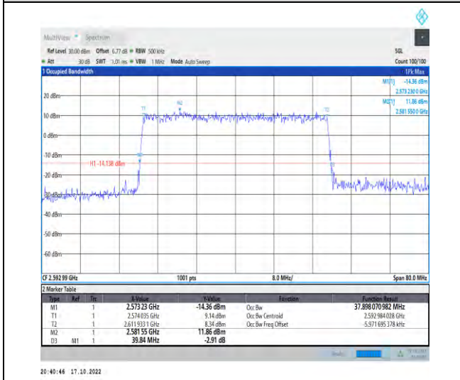
1-N41-PC2-30-40-M-8-CP-64QAM-Outer_Full-106 @0-Ant1-37.898-39.840-≤40-PASS
