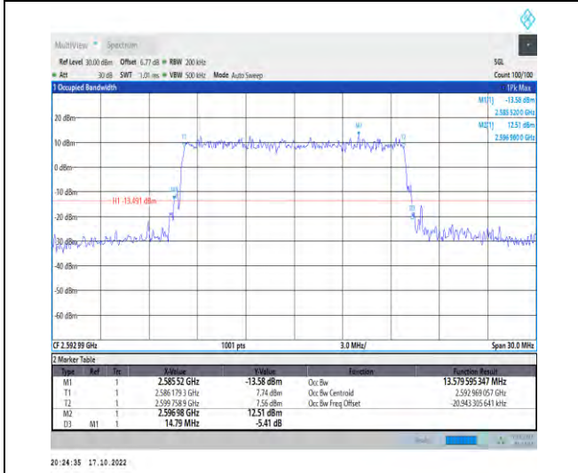
1-N41-PC2-30-15-M-8-CP-64QAM-Outer_Full-38@0-Ant1-13.58-14.790-≤15-PASS
