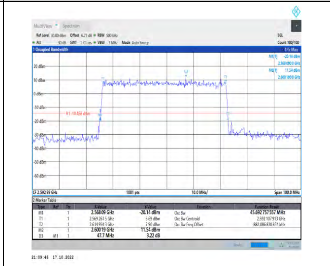
1-N41-PC2-30-50-M-5-DFT-256QAM-Outer_Full-128 @0-Ant1-45.693-47.700-≤50-PASS
