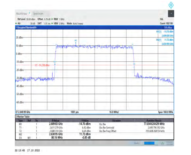
1-N41-PC2-30-80-H-5-DFT-256QAM-Outer_Full-216 @0-Ant1-77.035-80.160-≤80-PASS
