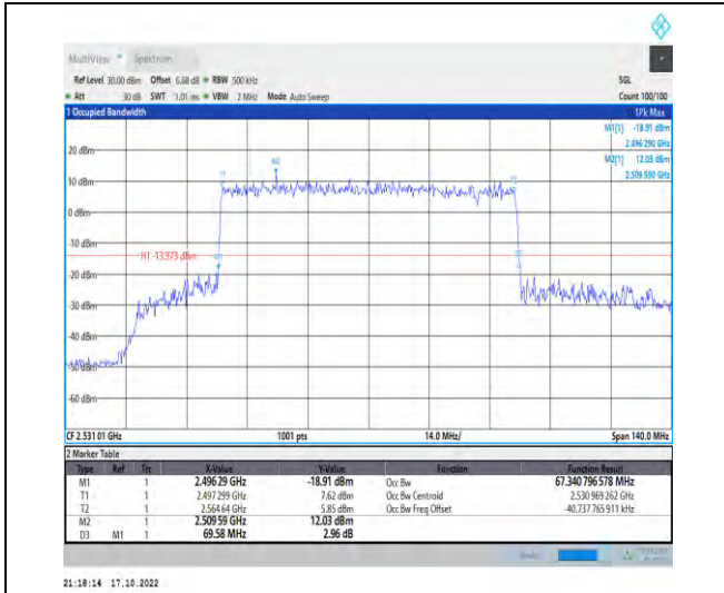
1-N41-PC2-30-70-L-6-CP-QPSK-Outer_Full-189@0 -Ant1-67.341-69.580-≤70-PASS
