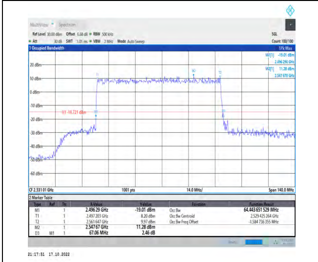
1-N41-PC2-30-70-L-4-DFT-64QAM-Outer_Full-180 @0-Ant1-64.444-67.060-≤70-PASS
