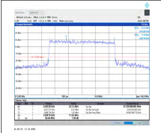
1-N41-PC2-30-70-H-8-CP-64QAM-Outer_Full-189@0 -Ant1-67.359-69.440-≤70-PASS
