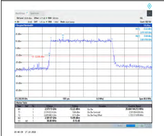
1-N41-PC2-30-40-M-4-DFT-64QAM-Outer_Full-100 @0-Ant1-35.664-38.080-≤40-PASS
