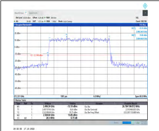
1-N41-PC2-30-30-L-1-DFT-QPSK-Outer_Full-75@0 -Ant1-26.784-28.500-≤30-PASS
