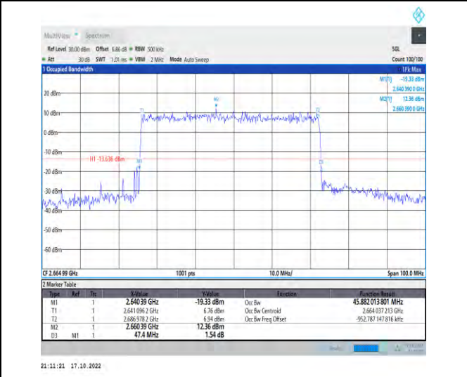
1-N41-PC2-30-50-H-5-DFT-256QAM-Outer_Full-128 @0-Ant1-45.882-47.400-≤50-PASS
