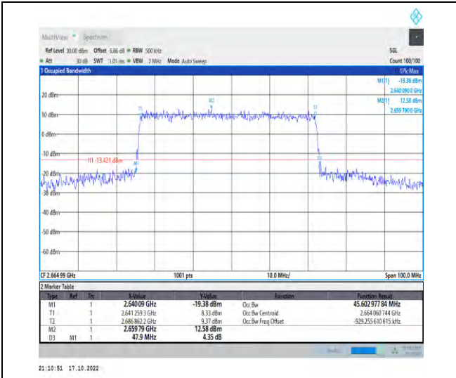
1-N41-PC2-30-50-H-1-DFT-QPSK-Outer_Full-128@ 0-Ant1-45.603-47.900-≤50-PASS
