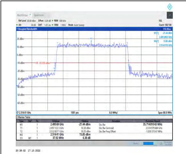
1-N41-PC2-30-40-L-1-DFT-QPSK-Outer_Full-100@ 0-Ant1-35.715-37.920-≤40-PASS
