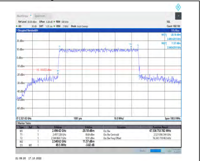
1-N41-PC2-30-50-L-7-CP-16QAM-Outer_Full-133@0 -Ant1-47.537-49.500-≤50-PASS
