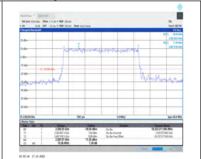
1-N41-PC2-30-20-M-7-CP-16QAM-Outer_Full-51@0-Ant1-18.253-19.360-≤20-PASS
