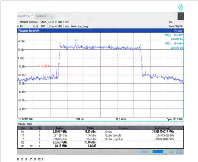
1-N41-PC2-30-80-H-1-DFT-QPSK-Outer_Full-216@ 0-Ant1-76.926-80.160-≤80-PASS
