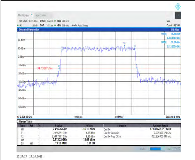
1-N41-PC2-30-20-L-4-DFT-64QAM-Outer_Full-50@0 -Ant1-17.833-19.120-≤20-PASS
