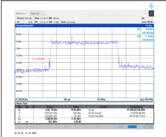
1-N41-PC2-30-50-M-8-CP-64QAM-Outer_Full-133@0-Ant1-47.43-50.200-≤50-PASS
