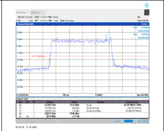
1-N41-PC2-30-30-M-5-DFT-256QAM-Outer_Full-75 @0-Ant1-26.788-28.140-≤30-PASS
