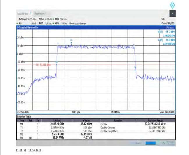
1-N41-PC2-30-60-L-4-DFT-64QAM-Outer_Full-162 @0-Ant1-57.748-59.640-≤60-PASS
