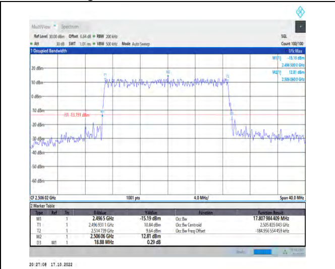
1-N41-PC2-30-20-L-3-DFT-16QAM-Outer_Full-50@0 -Ant1-17.808-18.880-≤20-PASS
