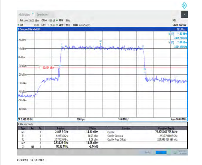
1-N41-PC2-30-80-L-4-DFT-64QAM-Outer_Full-216 @0-Ant1-76.875-80.320-≤80-PASS
