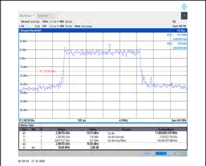
1-N41-PC2-30-20-M-5-DFT-256QAM-Outer_Full-50 @0-Ant1-17.851-18.640-<=20-PASS
