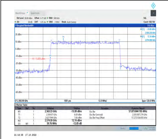
1-N41-PC2-30-60-M-4-DFT-64QAM-Outer_Full-162 @0-Ant1-57.874-59.760-≤60-PASS
