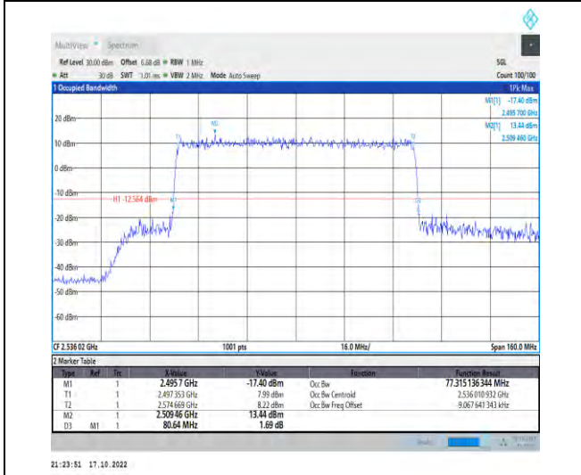
1-N41-PC2-30-80-L-8-CP-64QAM-Outer_Full-217@0 -Ant1-77.315-80.640-≤80-PASS
