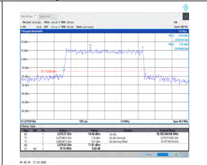
1-N41-PC2-30-20-H-7-CP-16QAM-Outer_Full-51@0-Ant1-18.183-19.160-<=20-PASS
