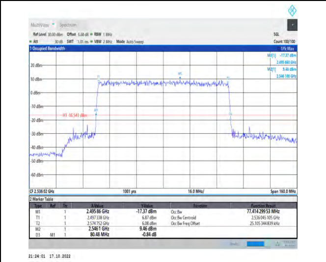
1-N41-PC2-30-80-L-9-CP-256QAM-Outer_Full-217@0 -Ant1-77.414-80.480-≤80-PASS
