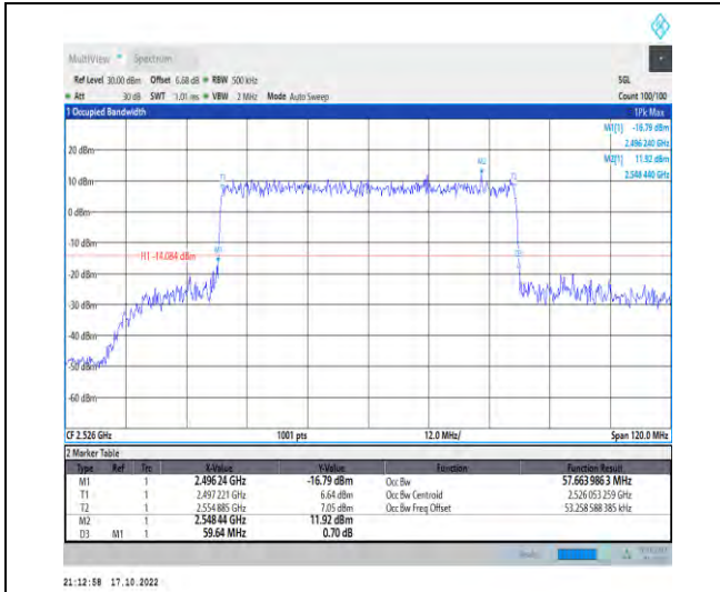
1-N41-PC2-30-60-L-6-CP-QPSK-Outer_Full-162@0 -Ant1-57.664-59.640-≤60-PASS
