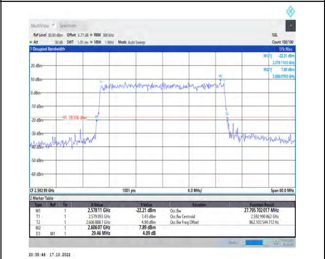
1-N41-PC2-30-30-M-9-CP-256QAM-Outer_Full-78@0-Ant1-27.796-29.460-≤30-PASS
