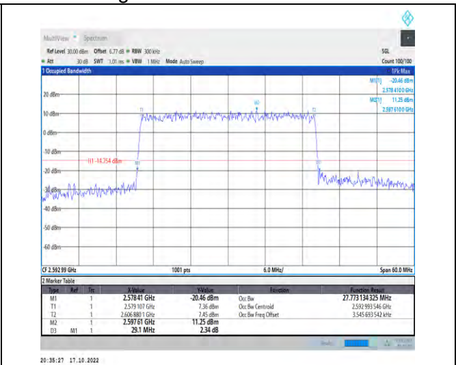
1-N41-PC2-30-30-M-7-CP-16QAM-Outer_Full-78@0-Ant1-27.773-29.100-≤30-PASS
