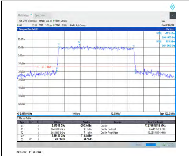
1-N41-PC2-30-50-H-6-CP-QPSK-Outer_Full-133@0 -Ant1-47.377-49.700-≤50-PASS
