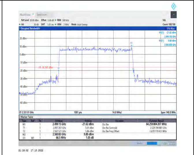
1-N41-PC2-30-70-L-5-DFT-256QAM-Outer_Full-180 @0-Ant1-64.26-66.500-≤70-PASS
