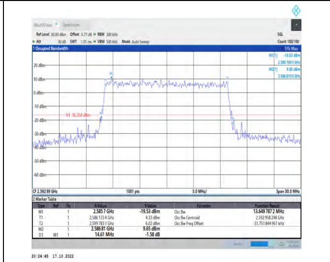
1-N41-PC2-30-15-M-9-CP-256QAM-Outer_Full-38@0-Ant1-13.65-14.610-≤15-PASS
