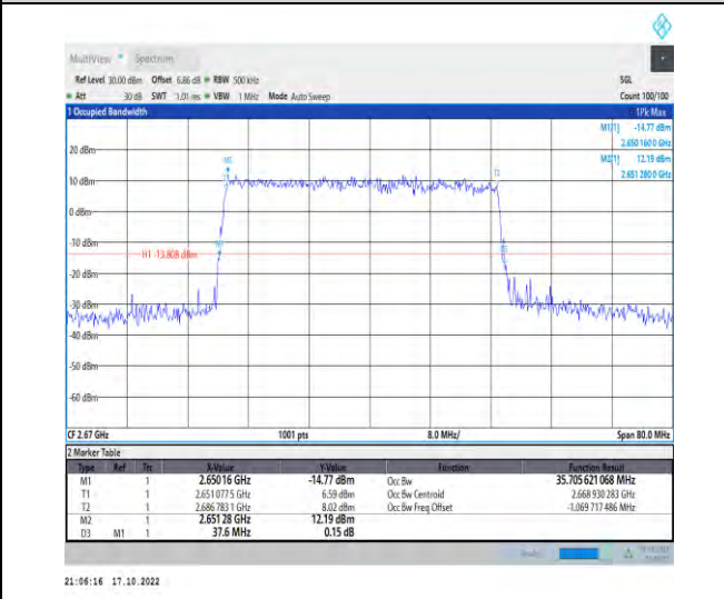
1-N41-PC2-30-40-H-5-DFT-256QAM-Outer_Full-100 @0-Ant1-35.706-37.600-≤40-PASS
