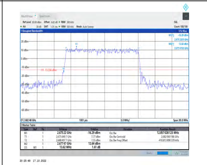
1-N41-PC2-30-15-H-5-DFT-256QAM-Outer_Full-36@0 -Ant1-12.857-13.620-≤15-PASS
