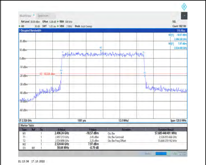
1-N41-PC2-30-60-L-9-CP-256QAM-Outer_Full-162@0 0-Ant1-57.685-59.640-≤60-PASS
