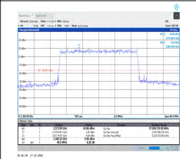
1-N41-PC2-30-40-M-9-CP-256QAM-Outer_Full-106 @0-Ant1-37.836-40.000-≤40-PASS
