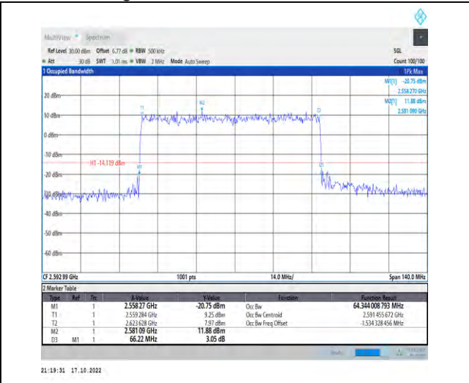
1-N41-PC2-30-70-M-3-DFT-16QAM-Outer_Full-180@0-Ant1-64.344-66.220-≤70-PASS
