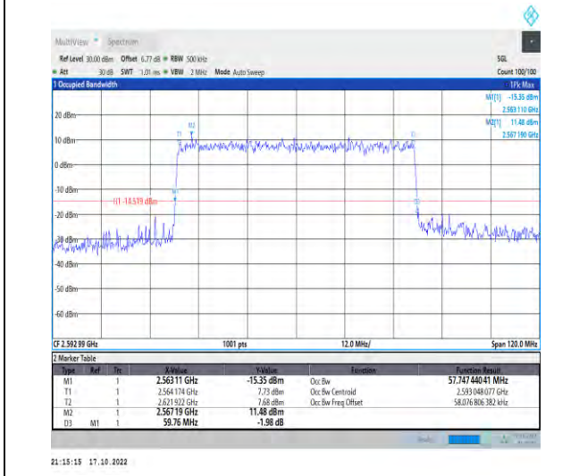
1-N41-PC2-30-60-M-8-CP-64QAM-Outer_Full-162 @0-Ant1-57.747-59.760-≤60-PASS
