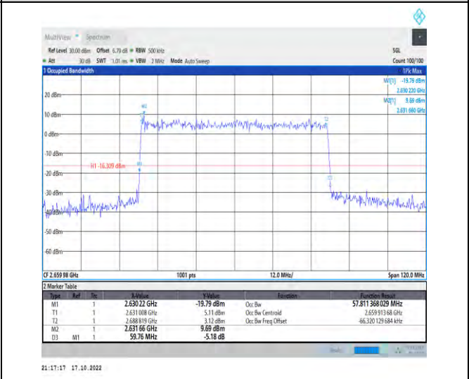
1-N41-PC2-30-60-H-9-CP-256QAM-Outer_Full-162@0-Ant1-57.811-59.760-≤60-PASS
