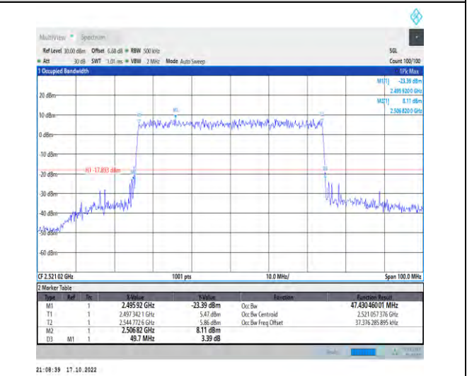
1-N41-PC2-30-50-L-9-CP-256QAM-Outer_Full-133@0 0-Ant1-47.43-49.700-≤50-PASS
