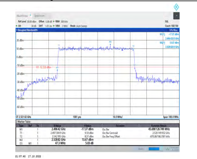
1-N41-PC2-30-50-L-3-DFT-16QAM-Outer_Full-128@0-Ant1-45.69-47.300-≤50-PASS
