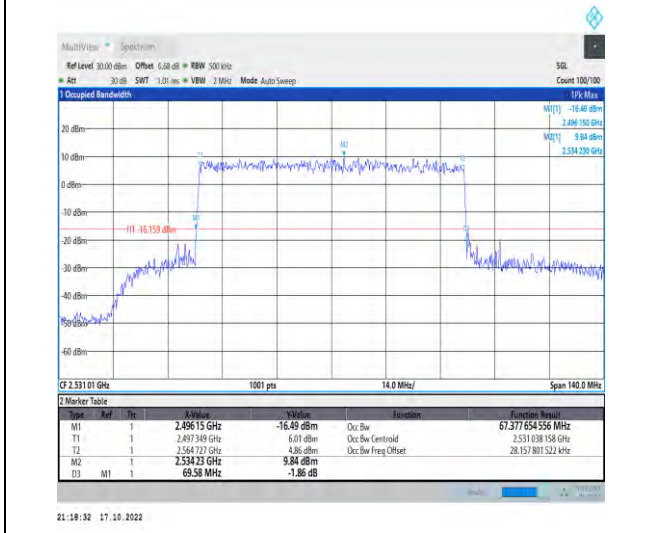
1-N41-PC2-30-70-L-8-CP-64QAM-Outer_Full-189@0 0-Ant1-67.378-69.580-≤70-PASS
