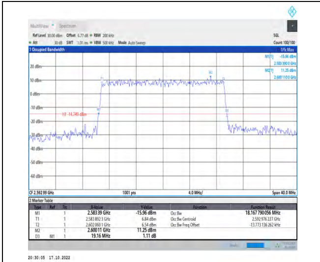
1-N41-PC2-30-20-M-6-CP-QPSK-Outer_Full-51@0-Ant1-18.168-19.160-≤20-PASS
