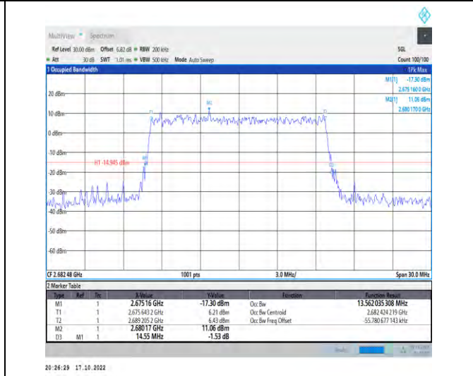
1-N41-PC2-30-15-H-9-CP-256QAM-Outer_Full-38@0-Ant1-13.562-14.550-≤15-PASS
