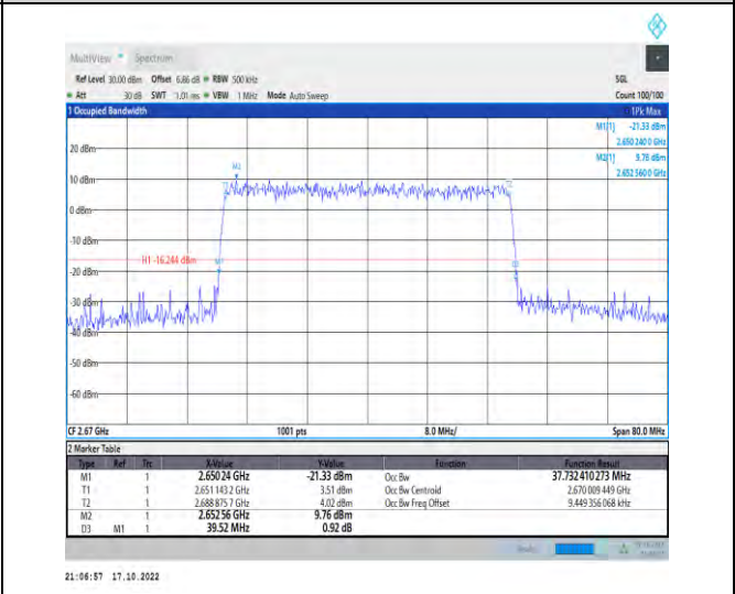
1-N41-PC2-30-40-H-9-CP-256QAM-Outer_Full-106@0 -Ant1-37.732-39.520-≤40-PASS
