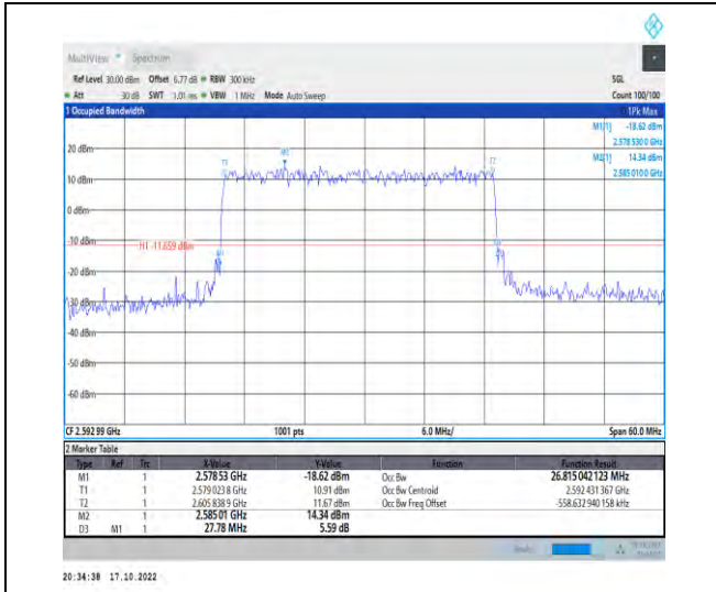
1-N41-PC2-30-30-M-1-DFT-QPSK-Outer_Full-75@0 -Ant1-26.815-27.780-≤30-PASS
