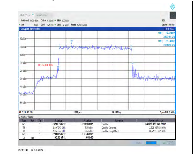
1-N41-PC2-30-70-L-3-DFT-16QAM-Outer_Full-180@ 0-Ant1-64.029-66.360-≤70-PASS
