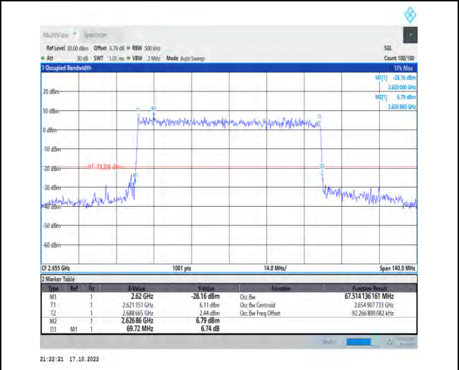
1-N41-PC2-30-70-H-9-CP-256QAM-Outer_Full-189@0 -Ant1-67.514-69.720-≤70-PASS
