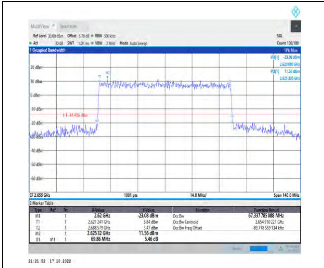
1-N41-PC2-30-70-H-6-CP-QPSK-Outer_Full-189@0 -Ant1-67.338-69.860-≤70-PASS
