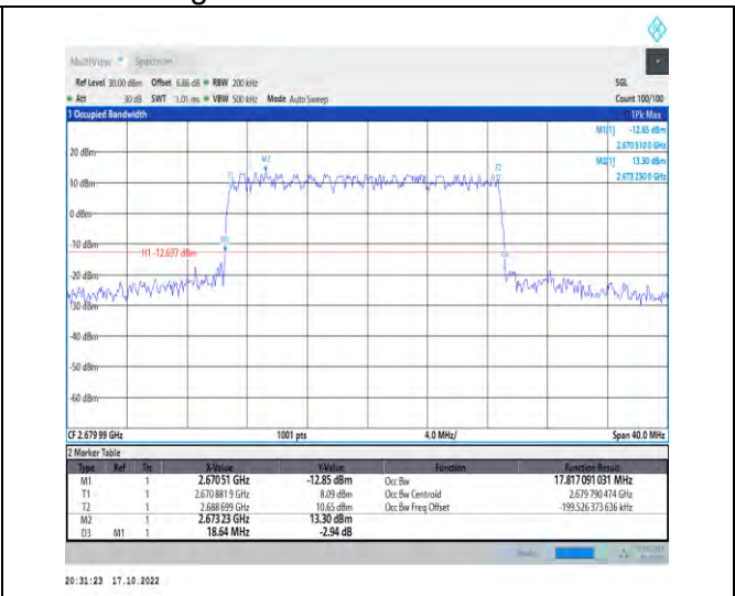
1-N41-PC2-30-20-H-3-DFT-16QAM-Outer_Full-50@0 0-Ant1-17.817-18.640-≤20-PASS
