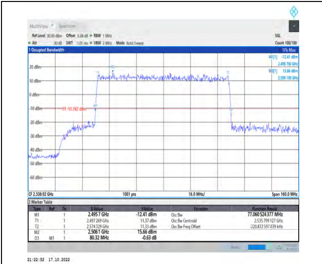
1-N41-PC2-30-80-L-1-DFT-QPSK-Outer_Full-216@ 0-Ant1-77.061-80.320-≤80-PASS
