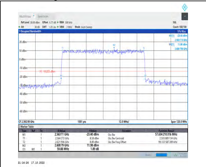
1-N41-PC2-30-60-M-3-DFT-16QAM-Outer_Full-162 @0-Ant1-57.634-59.880-≤60-PASS
