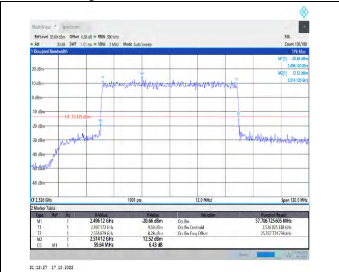
1-N41-PC2-30-60-L-3-DFT-16QAM-Outer_Full-162@ 0-Ant1-57.707-59.640-≤60-PASS
