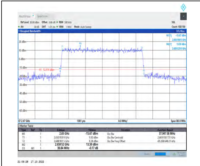
1-N41-PC2-30-40-H-6-CP-QPSK-Outer_Full-106@0 -Ant1-37.942-39.840-≤40-PASS
