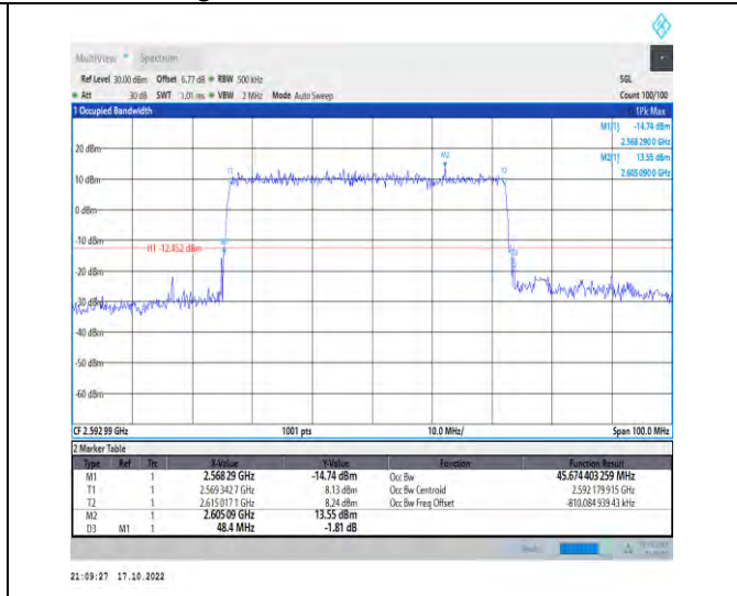
1-N41-PC2-30-50-M-3-DFT-16QAM-Outer_Full-128 @0-Ant1-45.674-48.400-≤50-PASS
