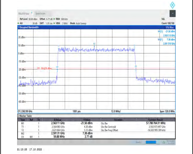
1-N41-PC2-30-60-M-9-CP-256QAM-Outer_Full-162 @0-Ant1-57.781-59.880-≤60-PASS
