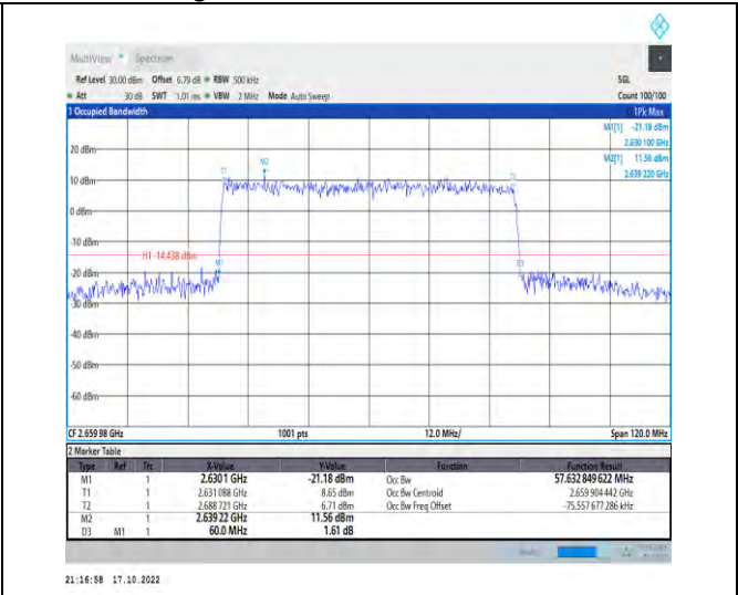
1-N41-PC2-30-60-H-7-CP-16QAM-Outer_Full-162@0-Ant1-57.633-60.000-≤60-PASS
