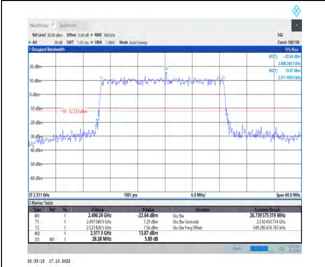
1-N41-PC2-30-30-L-4-DFT-64QAM-Outer_Full-75@0 -Ant1-26.74-28.380-≤30-PASS
