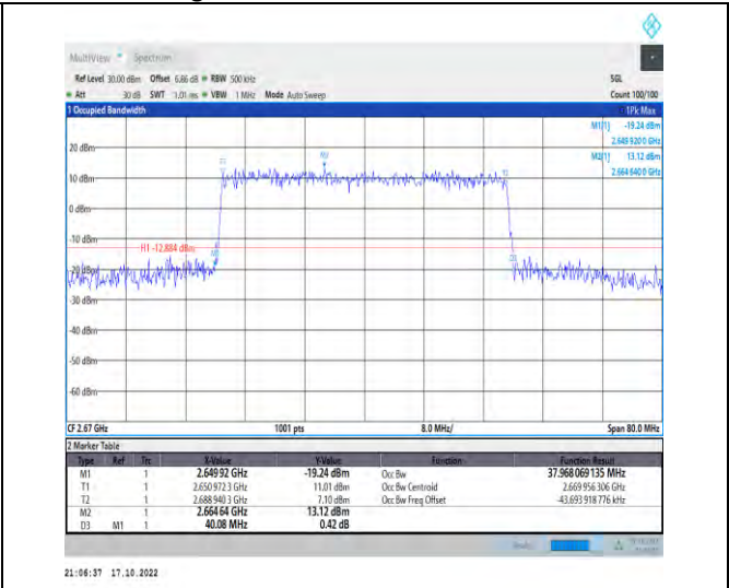
1-N41-PC2-30-40-H-7-CP-16QAM-Outer_Full-106@0 -Ant1-37.968-40.080-≤40-PASS
