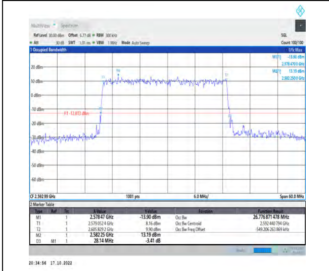
1-N41-PC2-30-30-M-4-DFT-64QAM-Outer_Full-75 @0-Ant1-26.777-28.140-≤30-PASS
