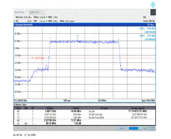
1-N41-PC2-30-80-L-5-DFT-256QAM-Outer_Full-216 @0-Ant1-77.115-80.160-≤80-PASS
