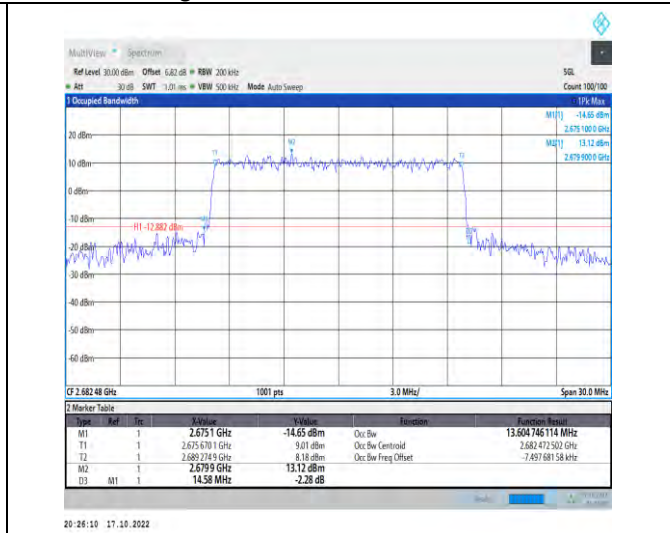
1-N41-PC2-30-15-H-7-CP-16QAM-Outer_Full-38@0-Ant1-13.605-14.580-≤15-PASS
