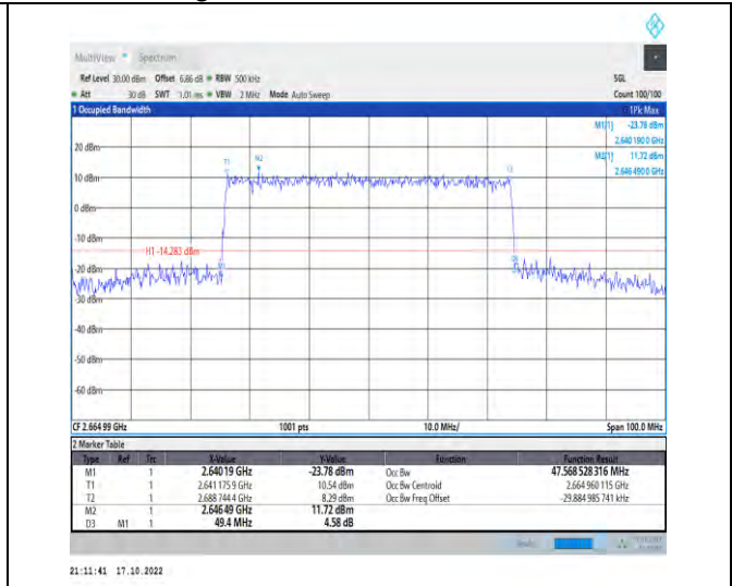
1-N41-PC2-30-50-H-7-CP-16QAM-Outer_Full-133@0 -Ant1-47.569-49.400-≤50-PASS
