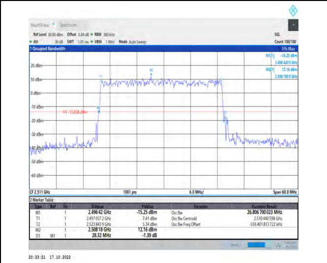
1-N41-PC2-30-30-L-5-DFT-256QAM-Outer_Full-75@0 -Ant1-26.807-28.320-≤30-PASS
