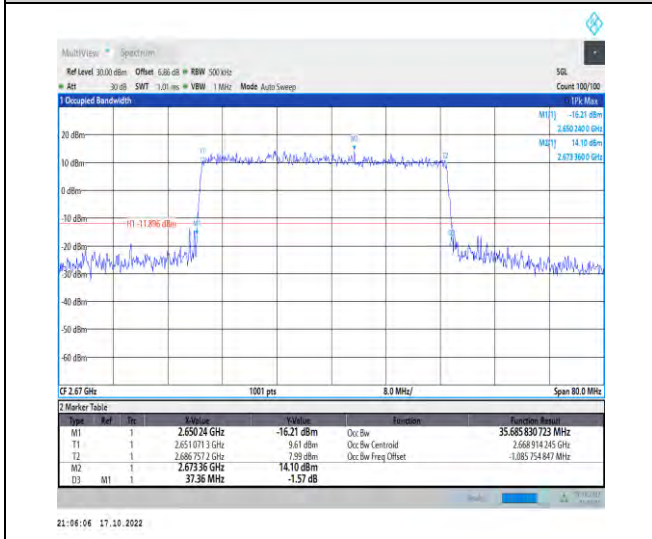
1-N41-PC2-30-40-H-4-DFT-64QAM-Outer_Full-100 @0-Ant1-35.686-37.360-≤40-PASS
