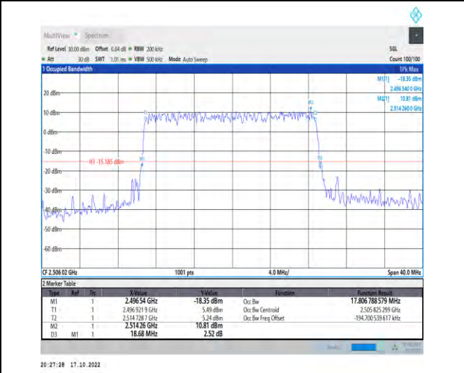
1-N41-PC2-30-20-L-5-DFT-256QAM-Outer_Full-50@0 -Ant1-17.807-18.680-≤20-PASS
