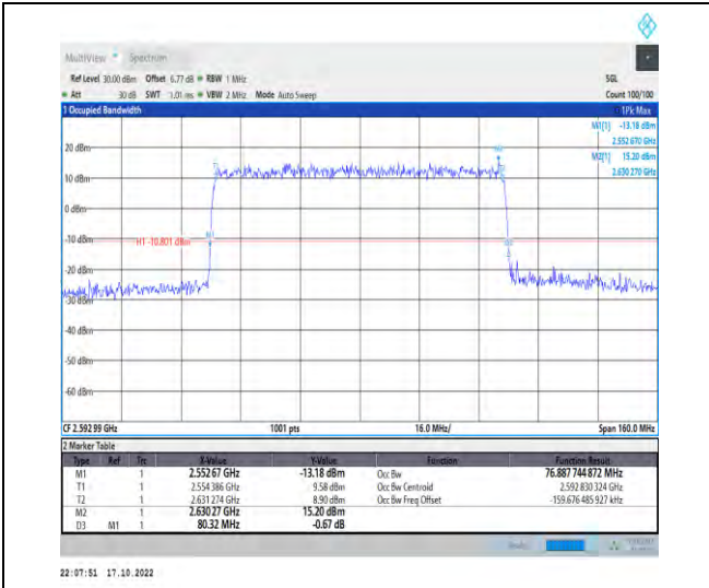
1-N41-PC2-30-80-M-1-DFT-QPSK-Outer_Full-216@ @0-Ant1-76.888-80.320-≤80-PASS
