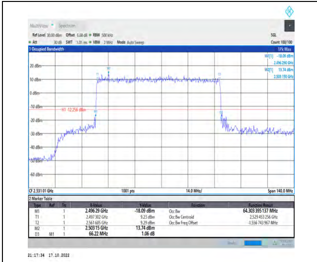
1-N41-PC2-30-70-L-1-DFT-QPSK-Outer_Full-180@ 0-Ant1-64.303-66.220-≤70-PASS
