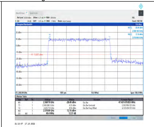
1-N41-PC2-30-50-M-7-CP-16QAM-Outer_Full-133@0-Ant1-47.432-49.400-≤50-PASS
