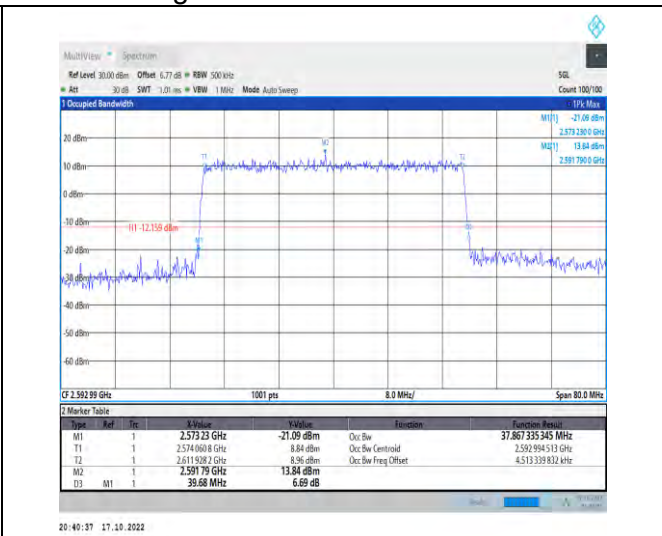
1-N41-PC2-30-40-M-7-CP-16QAM-Outer_Full-106@ 0-Ant1-37.867-39.680-≤40-PASS
