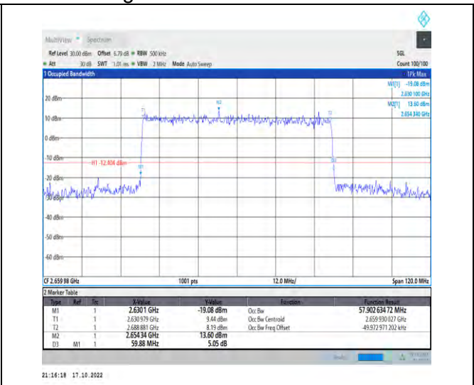
1-N41-PC2-30-60-H-3-DFT-16QAM-Outer_Full-162 @0-Ant1-57.903-59.880-≤60-PASS
