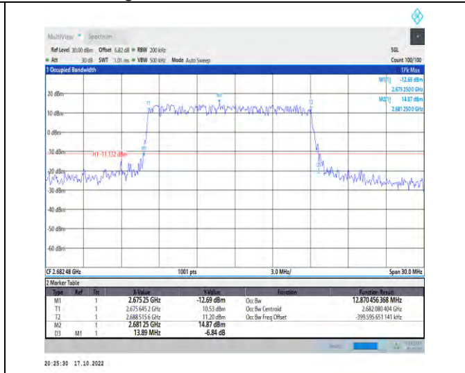
1-N41-PC2-30-15-H-3-DFT-16QAM-Outer_Full-36@0 -Ant1-12.87-13.890-≤15-PASS
