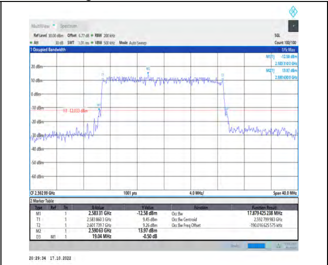
1-N41-PC2-30-20-M-3-DFT-16QAM-Outer_Full-50@0 0-Ant1-17.879-19.040-<=20-PASS
