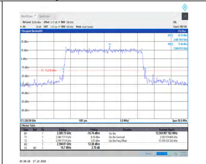
1-N41-PC2-30-15-M-7-CP-16QAM-Outer_Full-38@0-Ant1-13.594-14.700-≤15-PASS
