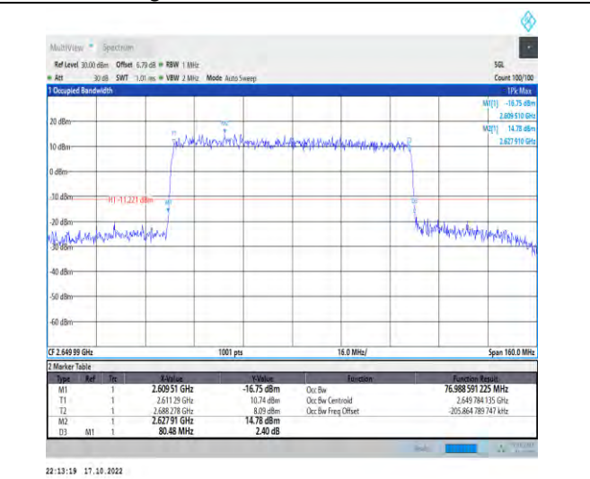
1-N41-PC2-30-80-H-3-DFT-16QAM-Outer_Full-216 @0-Ant1-76.989-80.480-≤80-PASS
