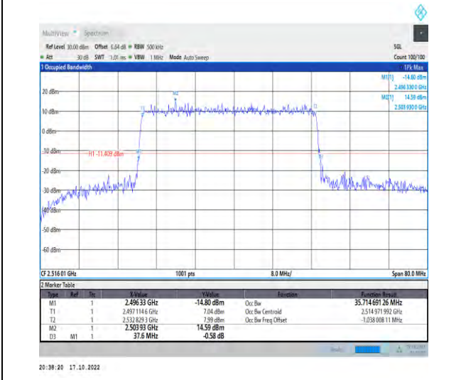
1-N41-PC2-30-40-L-4-DFT-64QAM-Outer_Full-100 @0-Ant1-35.715-37.600-≤40-PASS
