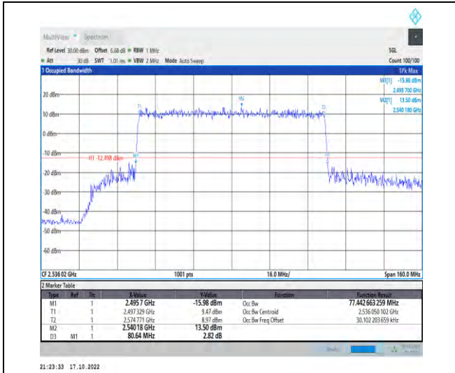
1-N41-PC2-30-80-L-6-CP-QPSK-Outer_Full-217@0 -Ant1-77.443-80.640-≤80-PASS
