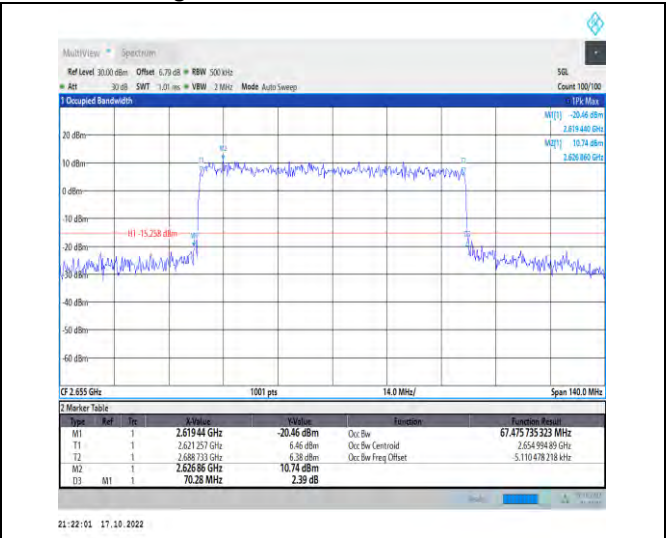
1-N41-PC2-30-70-H-7-CP-16QAM-Outer_Full-189@0 -Ant1-67.476-70.280-≤70-PASS
