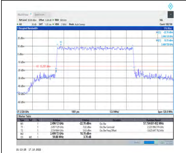
1-N41-PC2-30-60-L-8-CP-64QAM-Outer_Full-162@0 0-Ant1-57.735-59.880-≤60-PASS
