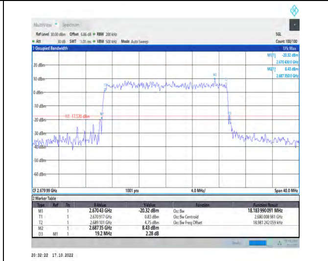
1-N41-PC2-30-20-H-9-CP-256QAM-Outer_Full-51@0-Ant1-18.184-19.200-<=20-PASS
