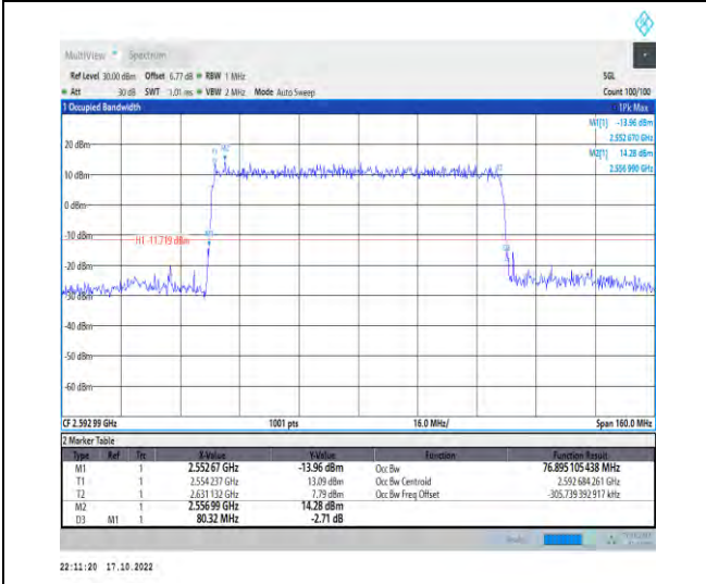
1-N41-PC2-30-80-M-4-DFT-64QAM-Outer_Full-216 @0-Ant1-76.895-80.320-≤80-PASS
