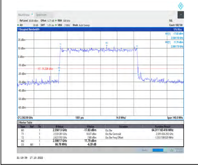
1-N41-PC2-30-70-M-4-DFT-64QAM-Outer_Full-180@0-Ant1-64.311-66.780-≤70-PASS
