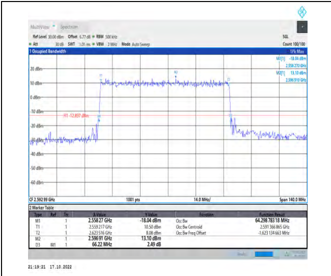
1-N41-PC2-30-70-M-1-DFT-QPSK-Outer_Full-180@0-Ant1-64.299-66.220-≤70-PASS
