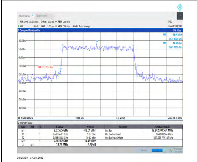
1-N41-PC2-30-15-H-4-DFT-64QAM-Outer_Full-36@0 -Ant1-12.843-13.770-≤15-PASS
