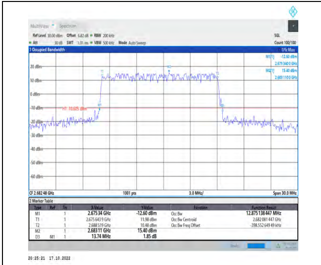
1-N41-PC2-30-15-H-1-DFT-QPSK-Outer_Full-36@0 -Ant1-12.875-13.740-≤15-PASS
