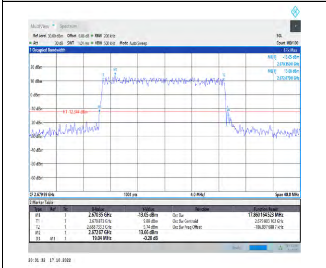
1-N41-PC2-30-20-H-4-DFT-64QAM-Outer_Full-50@0 0-Ant1-17.86-19.040-≤20-PASS
