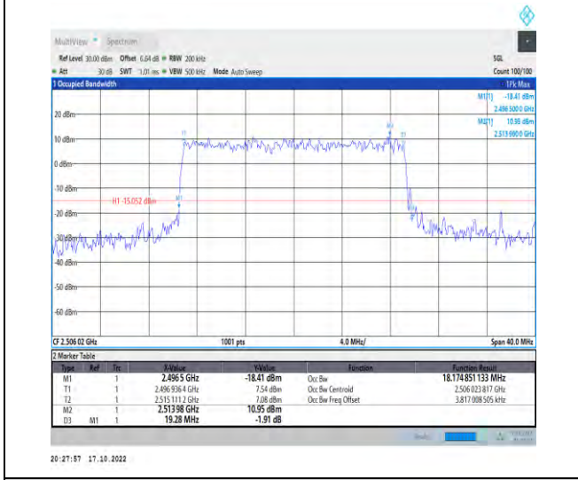
1-N41-PC2-30-20-L-8-CP-64QAM-Outer_Full-51@0-Ant1-18.175-19.280-≤20-PASS
