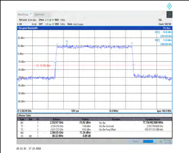
1-N41-PC2-30-80-M-5-DFT-256QAM-Outer_Full-216 @0-Ant1-77.156-80.320-≤80-PASS
