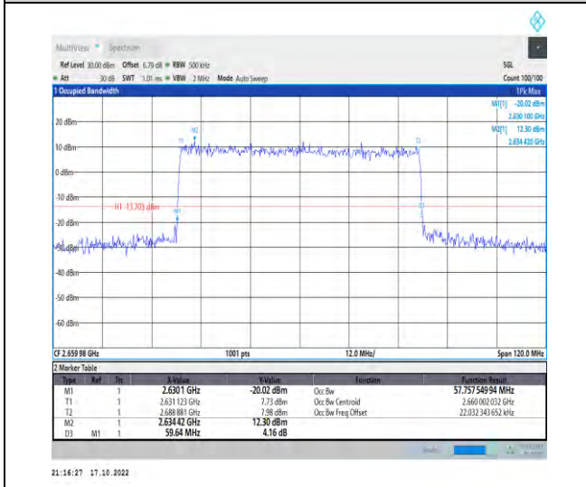
1-N41-PC2-30-60-H-4-DFT-64QAM-Outer_Full-162 @0-Ant1-57.758-59.640-≤60-PASS
