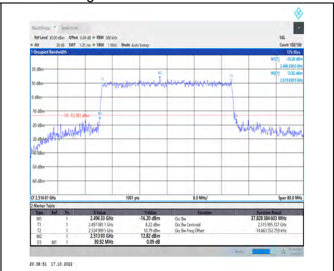
1-N41-PC2-30-40-L-7-CP-16QAM-Outer_Full-106@0 -Ant1-37.828-39.920-≤40-PASS
