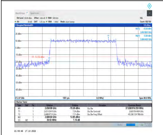
1-N41-PC2-30-40-H-8-CP-64QAM-Outer_Full-106@0 -Ant1-37.839-39.920-≤40-PASS
