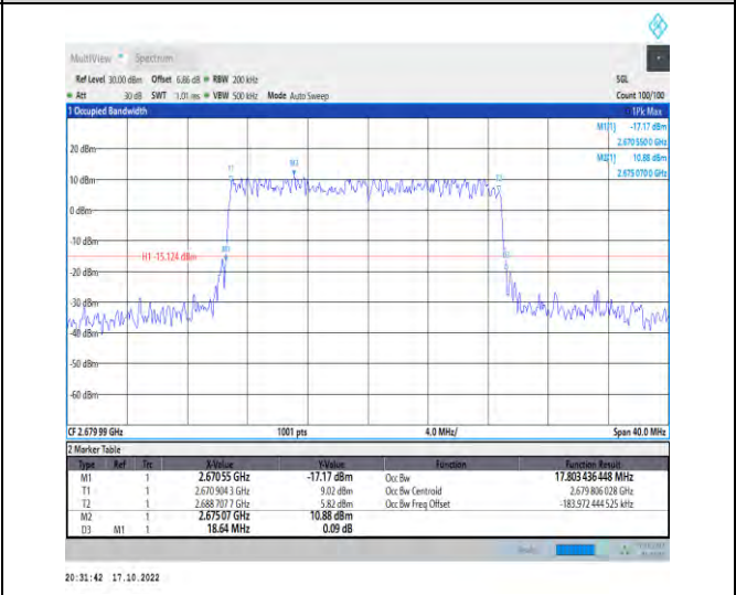
1-N41-PC2-30-20-H-5-DFT-256QAM-Outer_Full-50@0 0-Ant1-17.803-18.640-≤20-PASS
