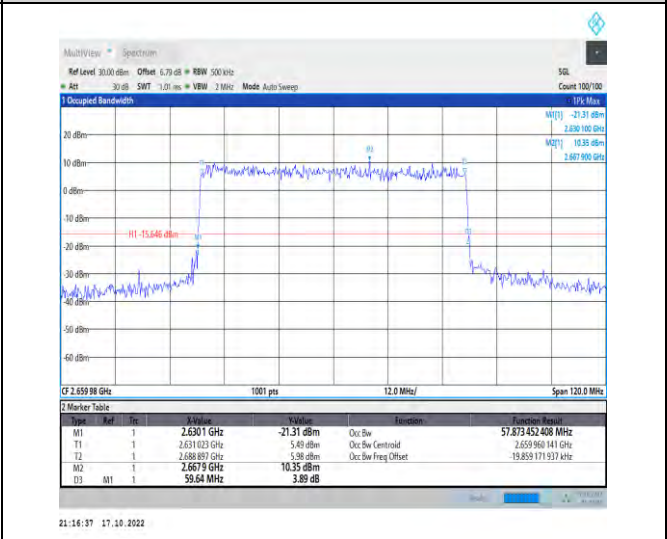
1-N41-PC2-30-60-H-5-DFT-256QAM-Outer_Full-162 @0-Ant1-57.873-59.640-≤60-PASS
