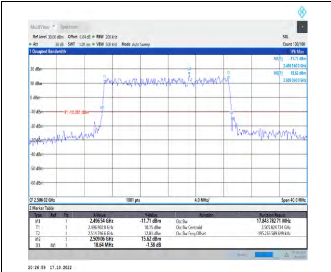
1-N41-PC2-30-20-L-1-DFT-QPSK-Outer_Full-50@0 -Ant1-17.844-18.640-≤20-PASS
