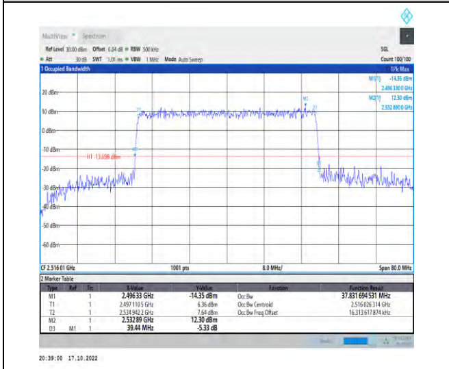
1-N41-PC2-30-40-L-8-CP-64QAM-Outer_Full-106@0 -Ant1-37.832-39.440-≤40-PASS
