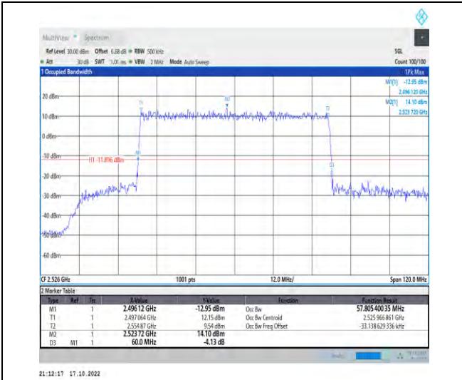
1-N41-PC2-30-60-L-1-DFT-QPSK-Outer_Full-162@ 0-Ant1-57.805-60.000-≤60-PASS
