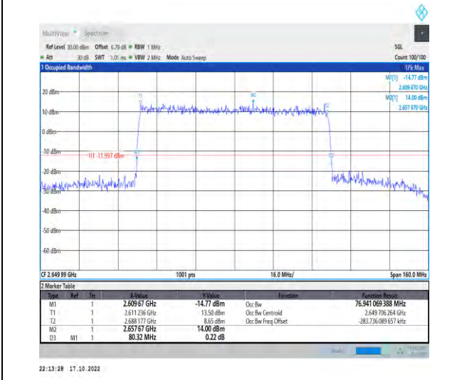
1-N41-PC2-30-80-H-4-DFT-64QAM-Outer_Full-216 @0-Ant1-76.941-80.320-≤80-PASS
