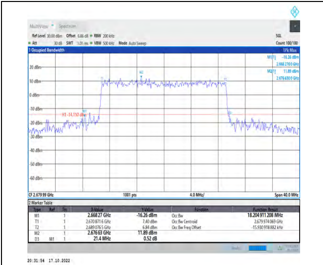
1-N41-PC2-30-20-H-6-CP-QPSK-Outer_Full-51@0-Ant1-18.205-21.400-<=20-PASS
