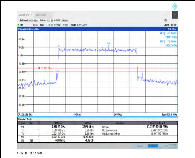
1-N41-PC2-30-60-M-5-DFT-256QAM-Outer_Full-162 @0-Ant1-57.784-60.000-≤60-PASS
