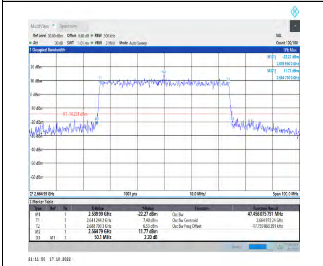
1-N41-PC2-30-50-H-8-CP-64QAM-Outer_Full-133@0 -Ant1-47.456-50.100-≤50-PASS
