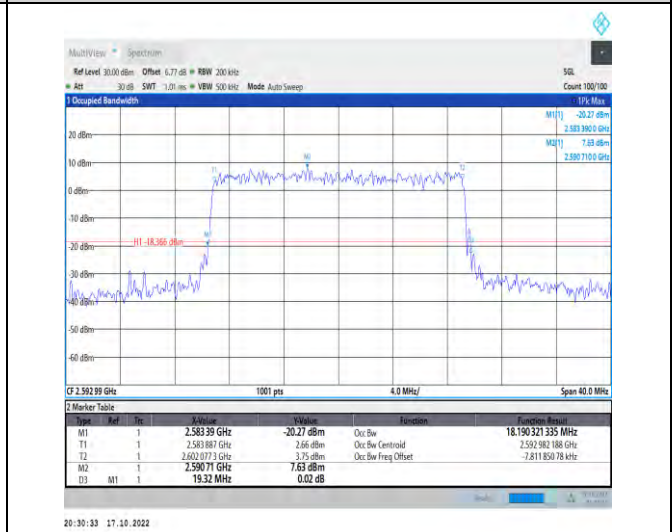
1-N41-PC2-30-20-M-9-CP-256QAM-Outer_Full-51@0-Ant1-18.19-19.320-≤20-PASS
