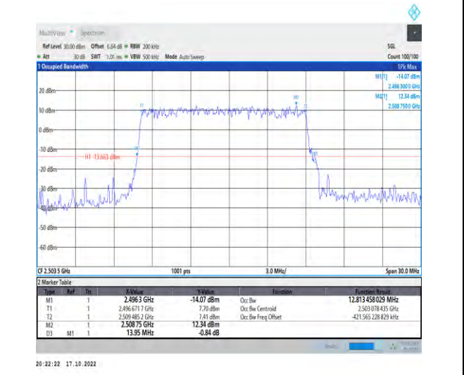
1-N41-PC2-30-15-L-5-DFT-256QAM-Outer_Full-36@0 -Ant1-12.813-13.950-≤15-PASS
