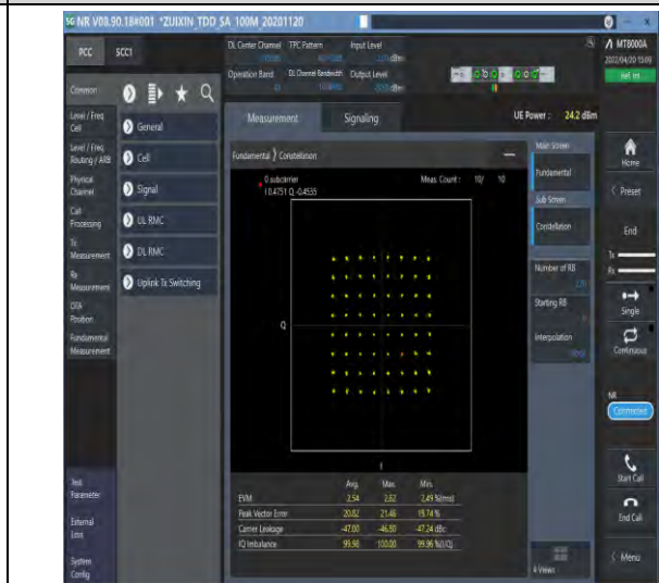
1-N41--30-100-M-4-DFT-64QAM-Outer_Full-270@0-Ant1-see graph-PASS
