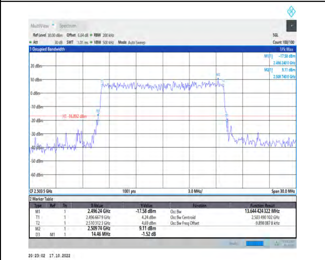
1-N41-PC2-30-15-L-9-CP-256QAM-Outer_Full-38@0-Ant1-13.644-14.460-≤15-PASS
