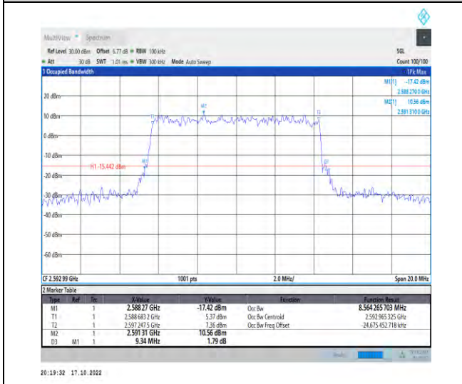
1-N41-PC2-30-10-M-8-CP-64QAM-Outer_Full-24@0-Ant1-8.564-9.340-≤10-PASS
