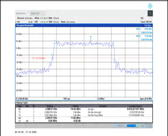
1-N41-PC2-30-10-M-5-DFT-256QAM-Outer_Full-24 @0-Ant1-8.616-9.060-≤10-PASS
