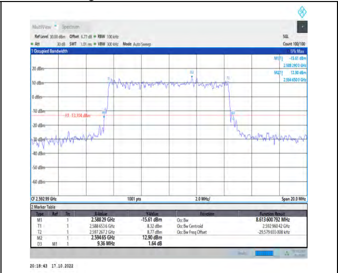
1-N41-PC2-30-10-M-3-DFT-16QAM-Outer_Full-24@0 -Ant1-8.614-9.360-≤10-PASS
