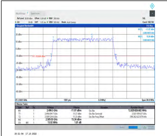
1-N41-PC2-30-15-L-1-DFT-QPSK-Outer_Full-36@0 -Ant1-12.83-13.920-≤15-PASS
