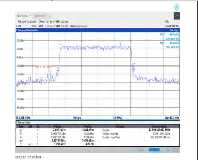
1-N41-PC2-30-15-L-3-DFT-16QAM-Outer_Full-36@0 -Ant1-12.899-13.980-≤15-PASS
