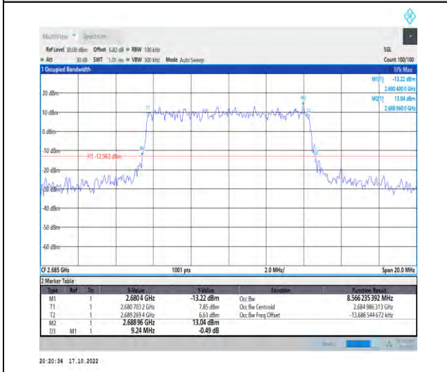
1-N41-PC2-30-10-H-4-DFT-64QAM-Outer_Full-24@ 0-Ant1-8.566-9.240-≤10-PASS
