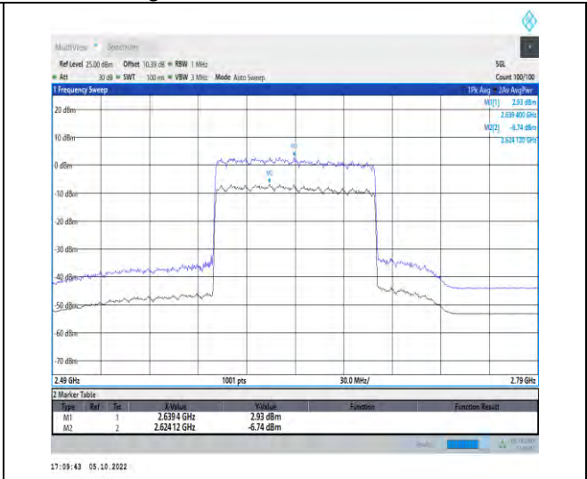
1-N41-PC2-30-100-H-2-CP-256QAM-Outer_Full-273 0@0-Ant1-9.67-100%-0.00-9.67-PASS-≤13
