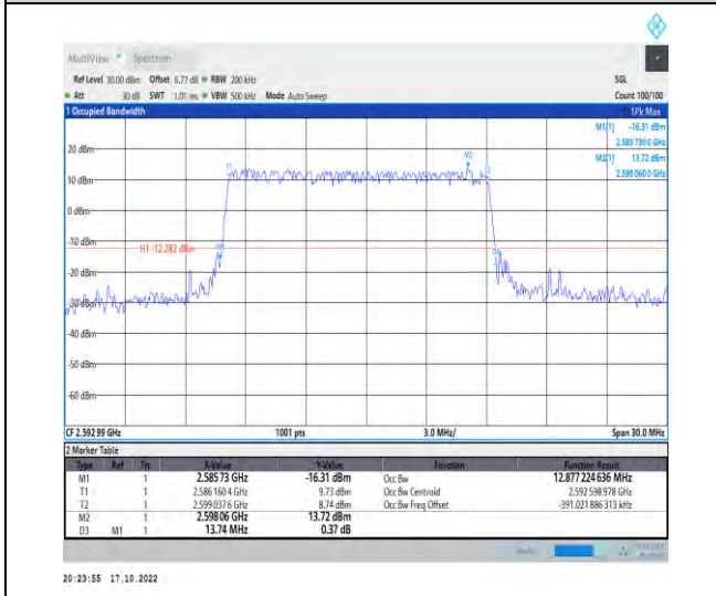
1-N41-PC2-30-15-M-4-DFT-64QAM-Outer_Full-36 @0-Ant1-12.877-13.740-≤15-PASS
