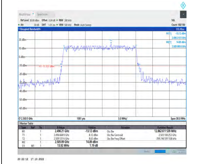
1-N41-PC2-30-15-L-4-DFT-64QAM-Outer_Full-36@0 -Ant1-12.863-13.920-≤15-PASS
