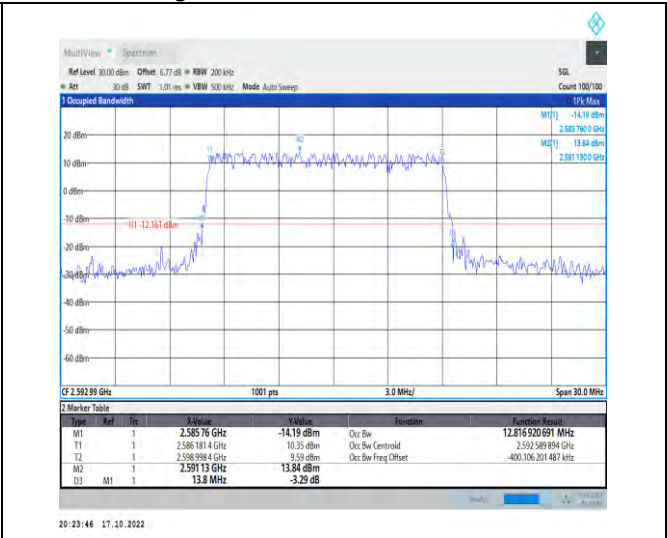
1-N41-PC2-30-15-M-3-DFT-16QAM-Outer_Full-36@0-Ant1-12.817-13.800-≤15-PASS
