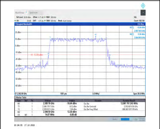
1-N41-PC2-30-15-M-5-DFT-256QAM-Outer_Full-36 @0-Ant1-12.862-14.070-≤15-PASS
