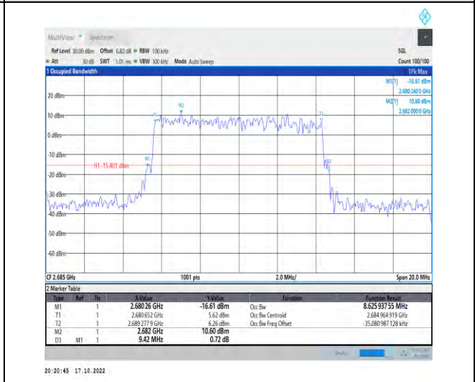
1-N41-PC2-30-10-H-5-DFT-256QAM-Outer_Full-24@ 0-Ant1-8.626-9.420-≤10-PASS
