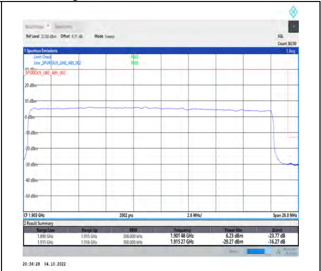
1-N25-PC3-15-25-H-3-DFT-QPSK-Outer_Full-128 @0-Ant1-1-seegraph-PASS-see graph
