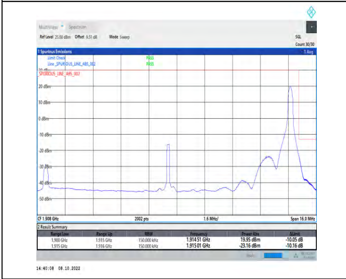
1-N25-PC3-15-15-H-5-CP-QPSK-Edge_1RB_Right-1 @78-Ant1-1-seegraph-PASS-see graph
