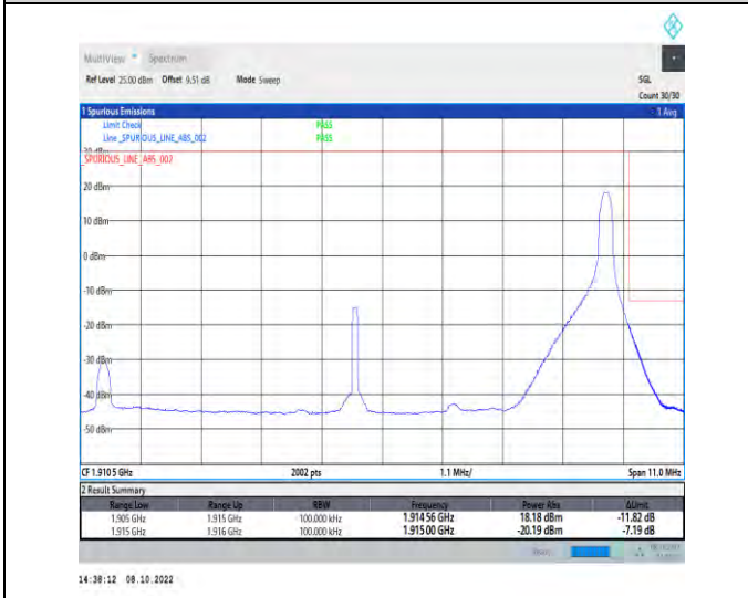
1-N25-PC3-15-10-H-5-CP-QPSK-Edge_1RB_Right-1 @51-Ant1-1-seegraph-PASS-see graph
