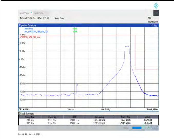
1-N25-PC3-15-5-H-2-DFT-QPSK-Edge_1RB_Right-1 @24-Ant1-1-seegraph-PASS-see graph
