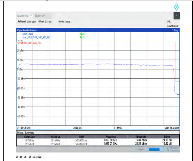
1-N25-PC3-15-40-H-3-DFT-QPSK-Outer_Full-216 @0-Ant1-1-seegraph-PASS-see graph
