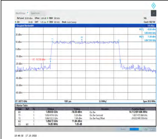
1-N25-PC3-15-15-L-8-CP-64QAM-Outer_Full-79@0-Ant1-14.113-14.850-≤15-PASS
