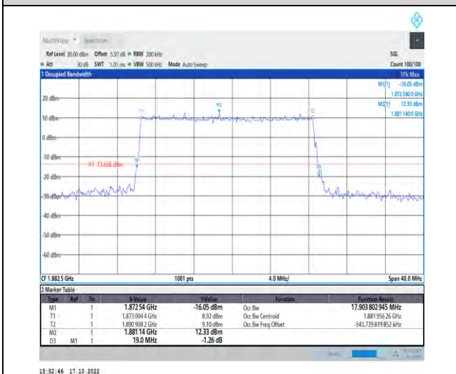
1-N25-PC3-15-20-M-4-DFT-64QAM-Outer_Full-100 @0-Ant1-17.904-19.000-≤20-PASS
