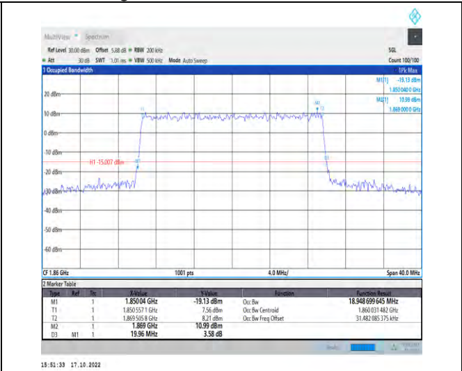
1-N25-PC3-15-20-L-7-CP-16QAM-Outer_Full-106@0 -Ant1-18.949-19.960-≤20-PASS
