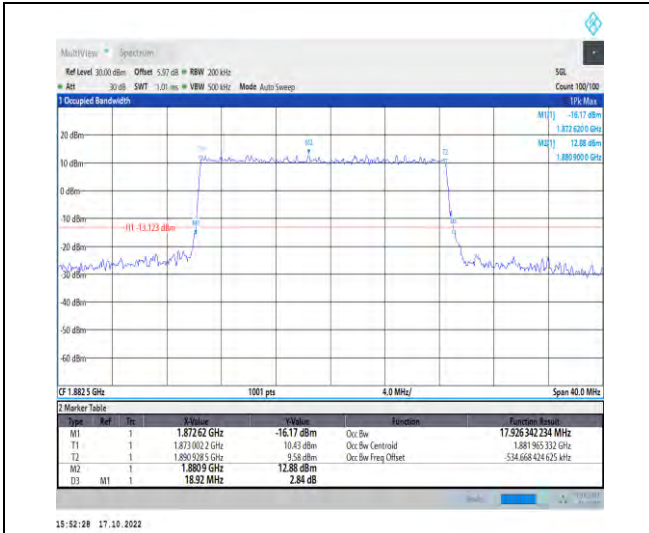
1-N25-PC3-15-20-M-1-DFT-QPSK-Outer_Full-100@ 0-Ant1-17.926-18.920-≤20-PASS
