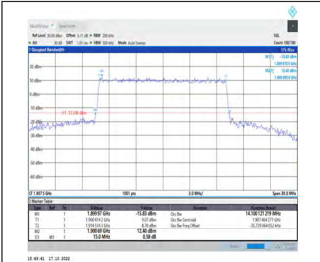
1-N25-PC3-15-15-H-6-CP-QPSK-Outer_Full-79@0-Ant1-14.1-15.000-≤15-PASS
