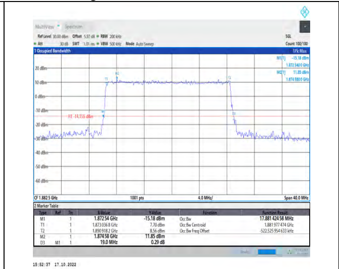
1-N25-PC3-15-20-M-3-DFT-16QAM-Outer_Full-100 @0-Ant1-17.881-19.000-≤20-PASS
