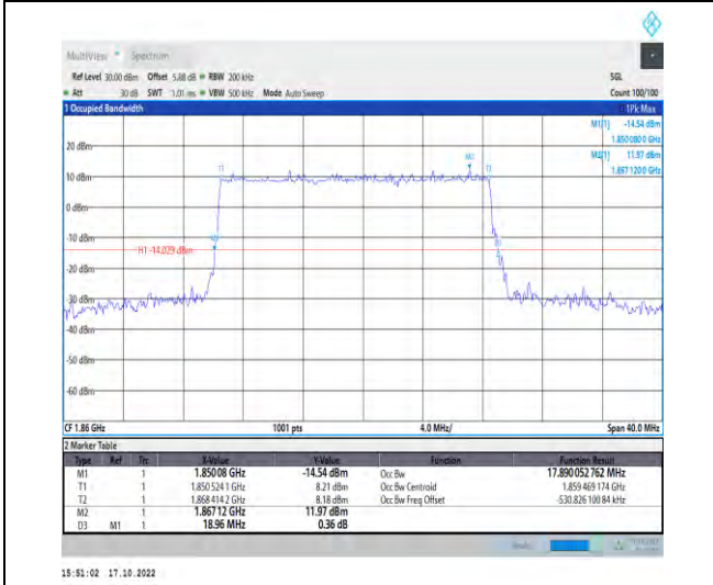
1-N25-PC3-15-20-L-4-DFT-64QAM-Outer_Full-100 @0-Ant1-17.89-18.960-≤20-PASS
