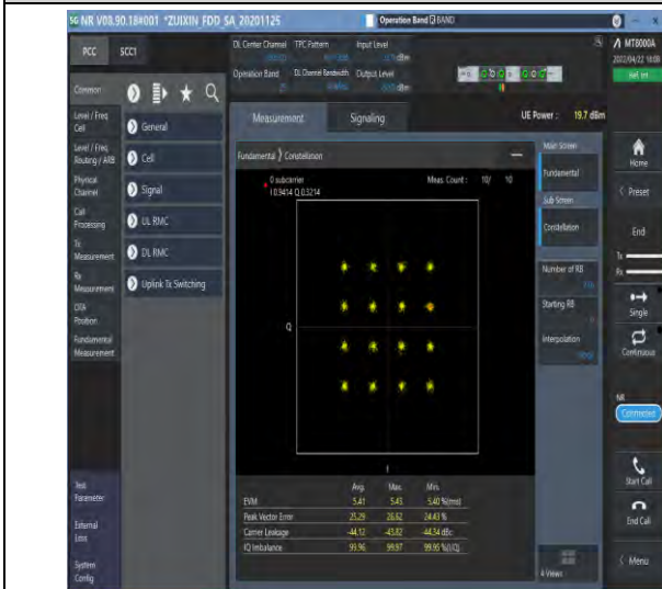
1-N25--15-40-M-7-CP-16QAM-Outer_Full-216@0-Ant1-see graph-PASS
