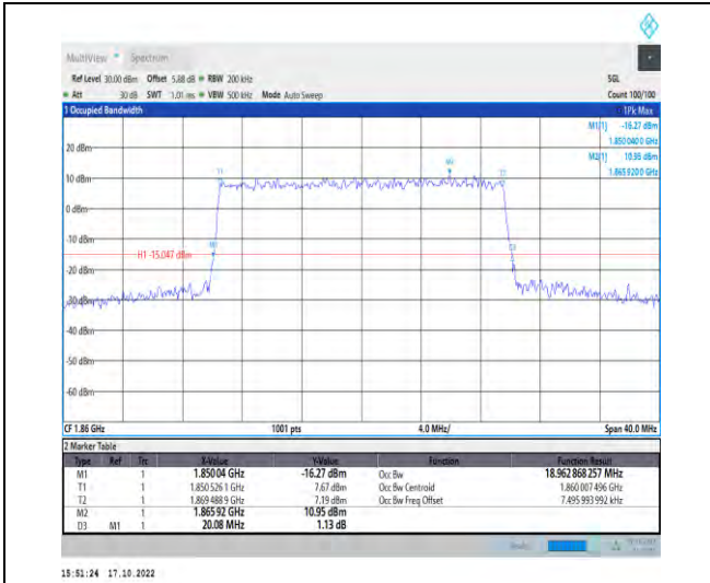
1-N25-PC3-15-20-L-6-CP-QPSK-Outer_Full-106@0 -Ant1-18.963-20.080-≤20-PASS
