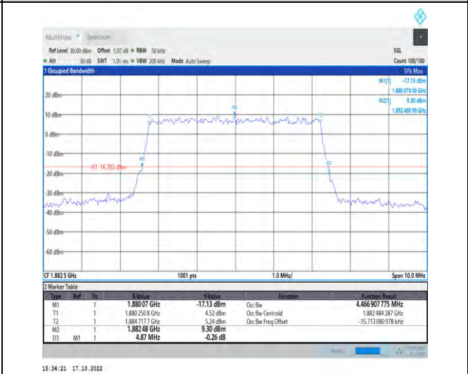
1-N25-PC3-15-5-M-5-DFT-256QAM-Outer_Full-25@0-Ant1-4.467-4.870-≤5-PASS
