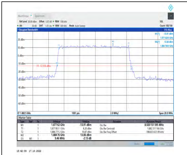
1-N25-PC3-15-10-M-1-DFT-QPSK-Outer_Full-50@0-Ant1-8.92-9.460-≤10-PASS
