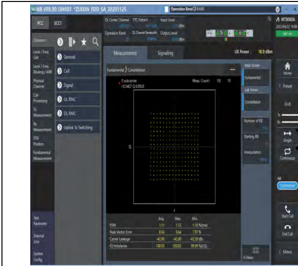
1-N25--15-40-M-5-DFT-256QAM-Outer_Full-216@0-Ant1-see graph-PASS
