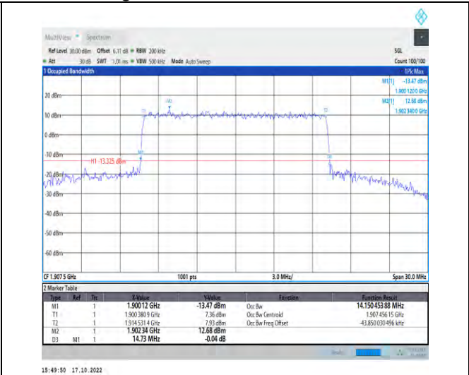
1-N25-PC3-15-15-H-7-CP-16QAM-Outer_Full-79@0-Ant1-14.15-14.730-≤15-PASS
