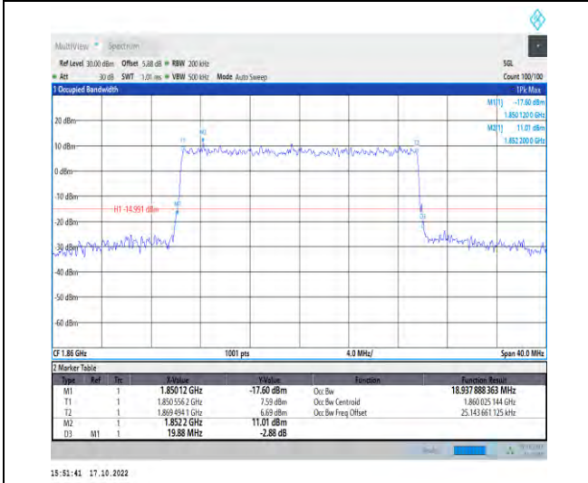
1-N25-PC3-15-20-L-8-CP-64QAM-Outer_Full-106@0 -Ant1-18.938-19.880-≤20-PASS
