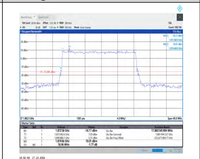
1-N25-PC3-15-20-M-5-DFT-256QAM-Outer_Full-100 @0-Ant1-17.884-18.960-≤20-PASS
