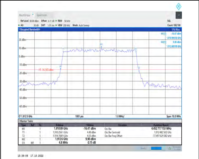
1-N25-PC3-15-5-H-5-DFT-256QAM-Outer_Full-25@0-Ant1-4.453-4.800-≤5-PASS
