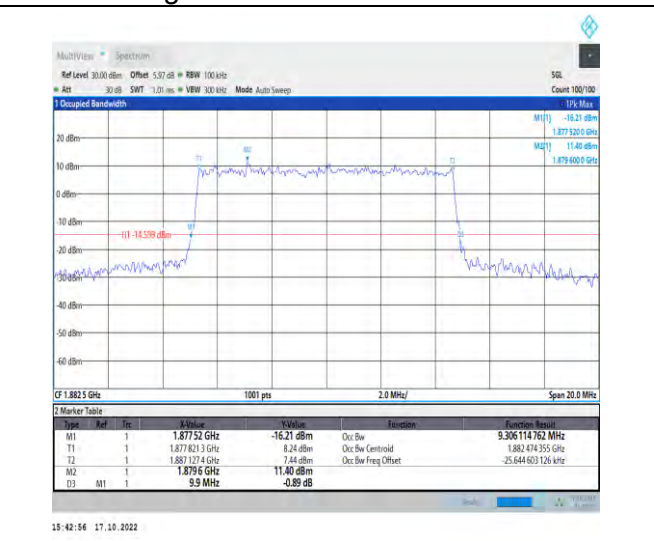
1-N25-PC3-15-10-M-7-CP-16QAM-Outer_Full-52@0-Ant1-9.306-9.900-≤10-PASS
