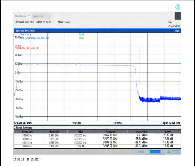
1-N77-3700-3980-PC2-30-30-H-6-CP-QPSK-Outer_Full-78@0-Ant1-1--PASS-see graph
