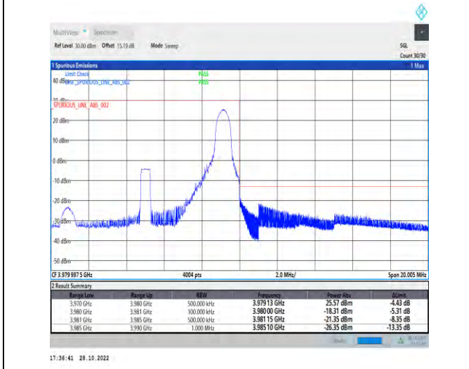
1-N77-3700-3980-PC2-30-10-H-5-CP-QPSK-Edge_1RB_Right-1@23-Ant1-1--PASS-see graph
