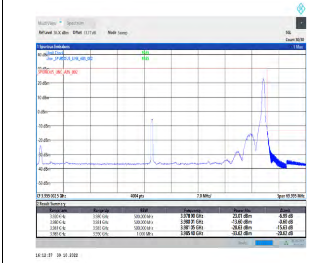
1-N77-3700-3980-PC2-30-60-H-5-CP-QPSK-Edge_1RB_Right-1@161-Ant1-1--PASS-see graph
