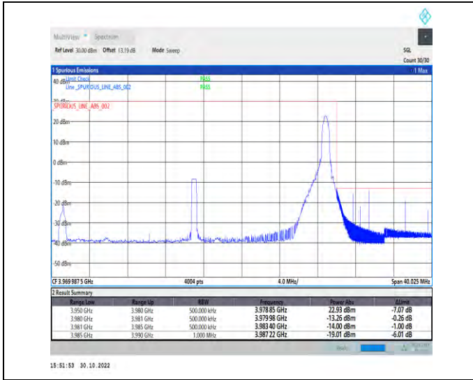
1-N77-3700-3980-PC2-30-30-H-2-DFT-PI2BPSK-Edge_1RB_Right-1@77-Ant1-1--PASS-see graph
