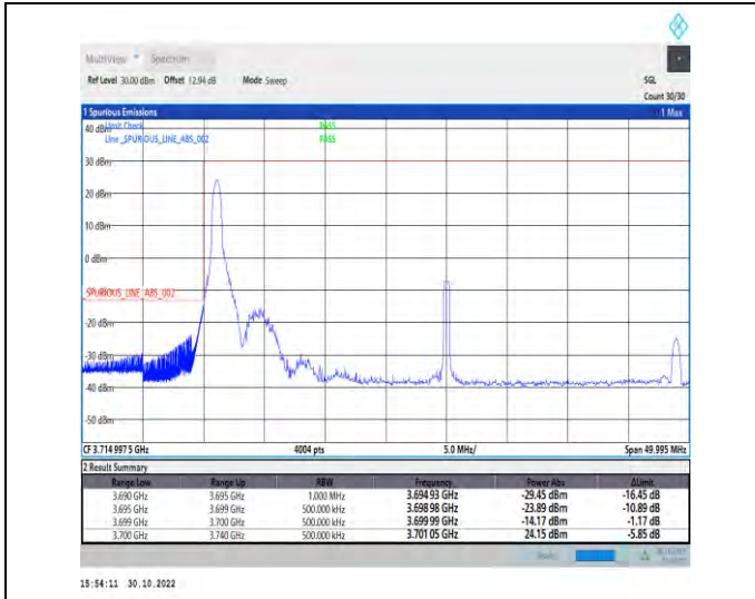
1-N77-3700-3980-PC2-30-40-L-1-DFT-PI2BPSK-Edge_1RB_Left-1@0-Ant1-1--PASS-see graph
