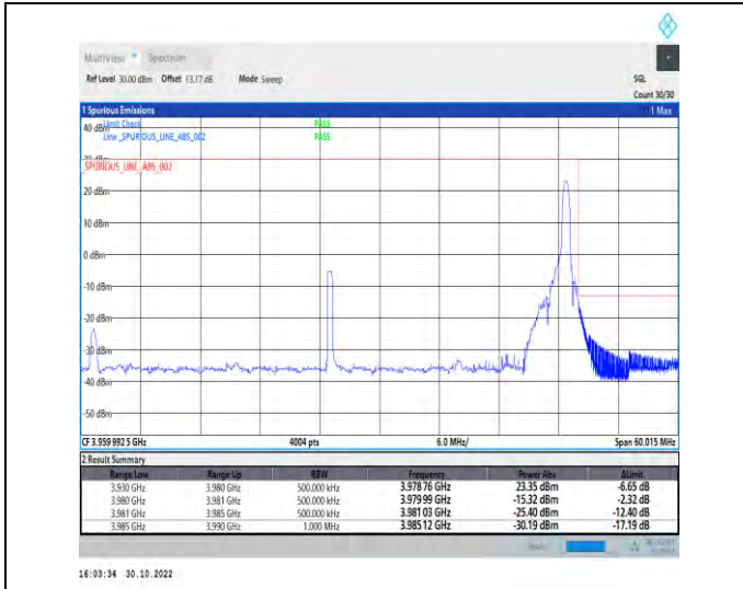
1-N77-3700-3980-PC2-30-50-H-2-DFT-PI2BPSK-Edge_1RB_Right-1@132-Ant1-1--PASS-see graph
