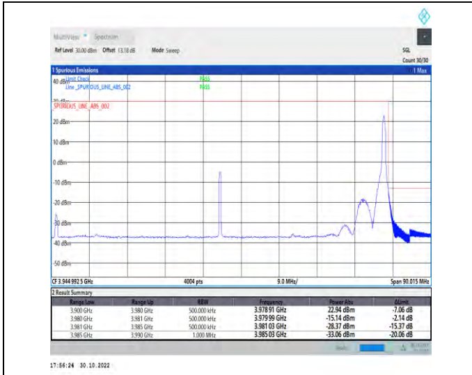
1-N77-3700-3980-PC2-30-80-H-2-DFT-PI2BPSK-Edge_1RB_Right-1@216-Ant1-1--PASS-see graph
