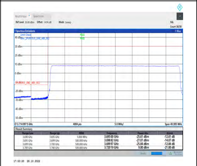
1-N77-3700-3980-PC2-30-40-L-6-CP-QPSK-Outer_Full-106@0-Ant1-1--PASS-see graph
