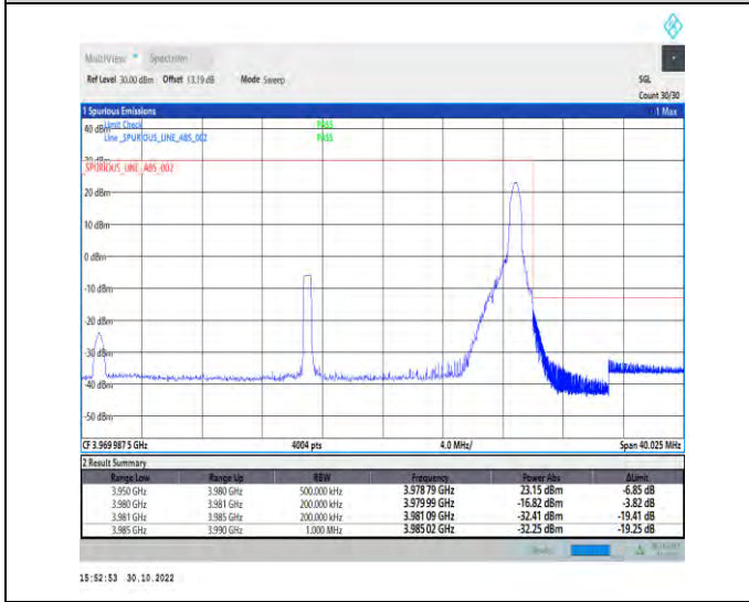
1-N77-3700-3980-PC2-30-30-H-5-CP-QPSK-Edge_1RB_Right-1@77-Ant1-1--PASS-see graph
