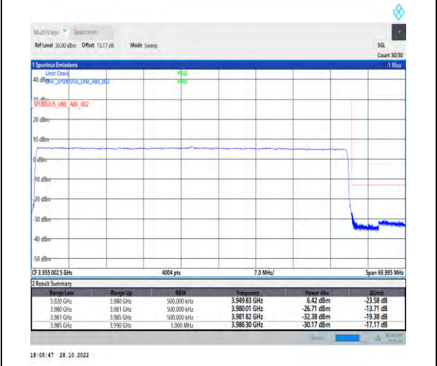
1-N77-3700-3980-PC2-30-60-H-6-CP-QPSK-Outer_Full-162@0-Ant1-1--PASS-see graph
