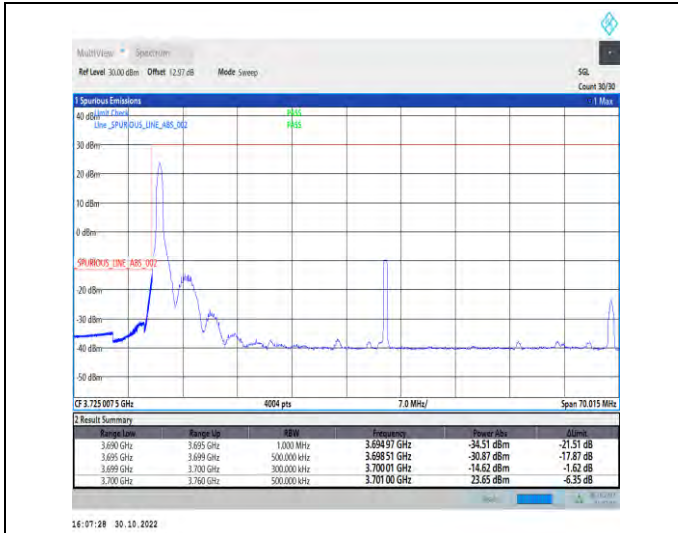
1-N77-3700-3980-PC2-30-60-L-1-DFT-PI2BPSK-Edge_1RB_Left-1@0-Ant1-1--PASS-see graph
