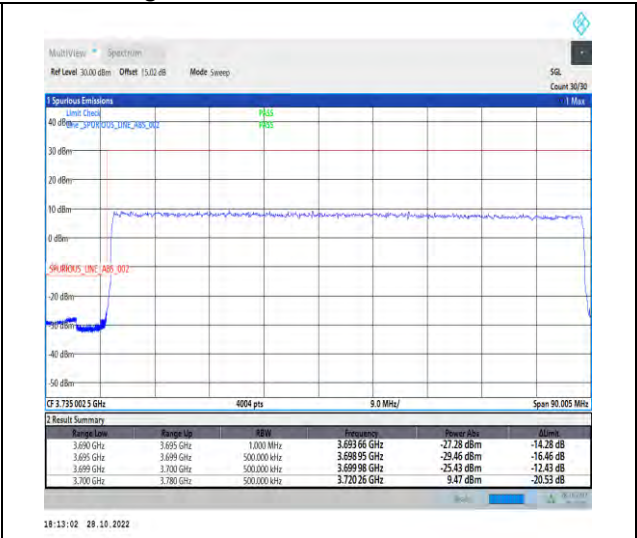
1-N77-3700-3980-PC2-30-80-L-3-DFT-PI2BPSK-Outer_Full-216@0-Ant1-1--PASS-see graph
