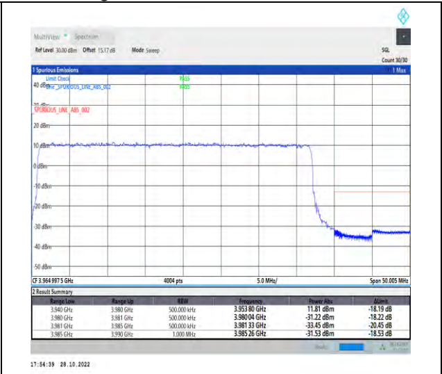
1-N77-3700-3980-PC2-30-40-H-3-DFT-PI2BPSK-Outer_Full-100@0-Ant1-1--PASS-see graph
