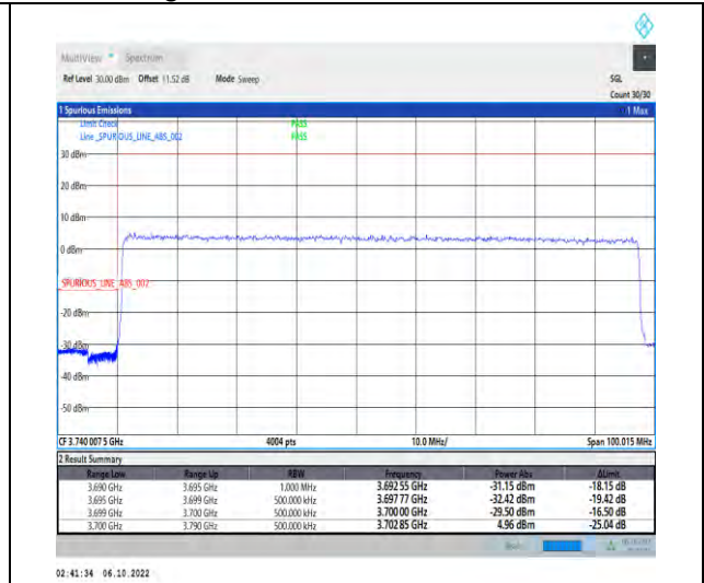
1-N77-3700-3980-PC2-30-90-L-3-DFT-QPSK-Outer_Full-240@0-Ant1-1--PASS-see graph
