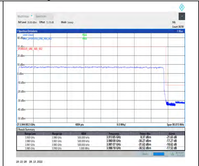
1-N77-3700-3980-PC2-30-80-H-3-DFT-PI2BPSK-Outer_Full-216@0-Ant1-1--PASS-see graph
