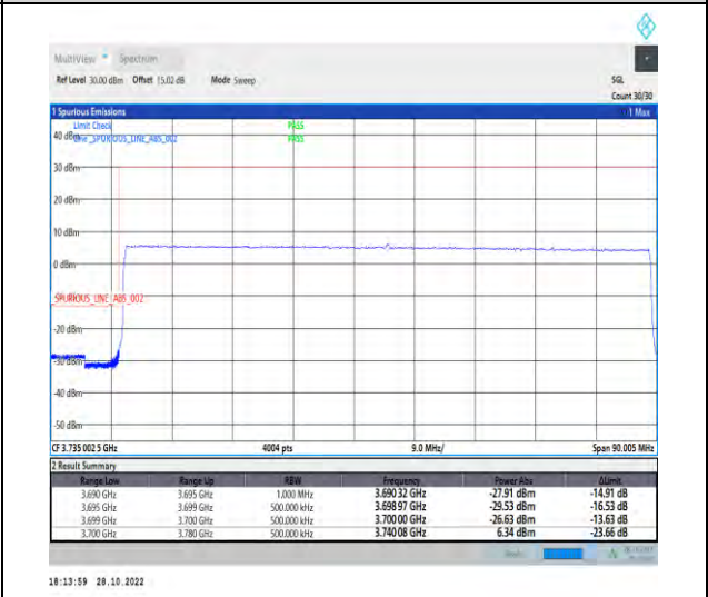
1-N77-3700-3980-PC2-30-80-L-6-CP-QPSK-Outer_Full-217@0-Ant1-1--PASS-see graph
