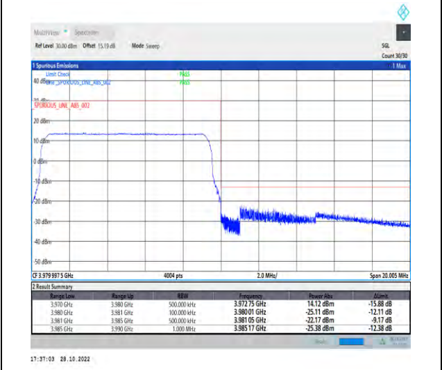
1-N77-3700-3980-PC2-30-10-H-6-CP-QPSK-Outer_Full-24@0-Ant1-1--PASS-see graph
