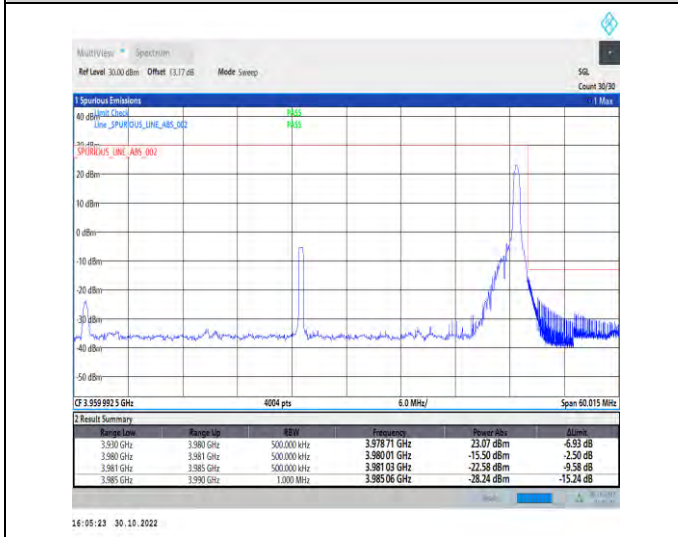
1-N77-3700-3980-PC2-30-50-H-5-CP-QPSK-Edge_1RB_Right-1@132-Ant1-1--PASS-see graph
