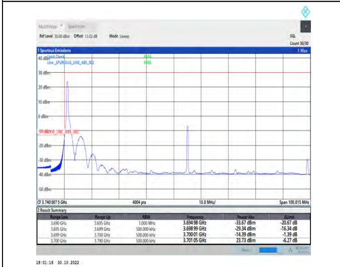
1-N77-3700-3980-PC2-30-90-L-4-CP-QPSK-Edge_1RB_Left-1@0-Ant1-1--PASS-see graph
