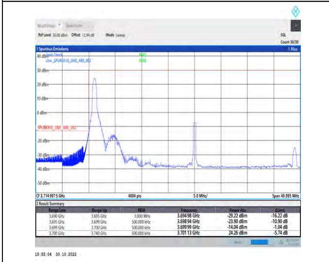
1-N77-3700-3980-PC2-30-40-L-4-CP-QPSK-Edge_1RB_Left-1@0-Ant1-1--PASS-see graph
