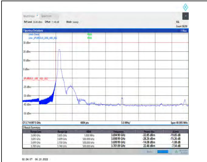
1-N77-3700-3980-PC2-30-40-L-1-DFT-QPSK-Edge_1 RB_Left-1@0-Ant1-1--PASS-see graph
