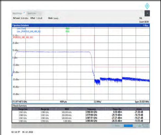
1-N77-3700-3980-PC2-30-15-H-6-CP-QPSK-Outer _Full-38@0-Ant1-1--PASS-see graph
