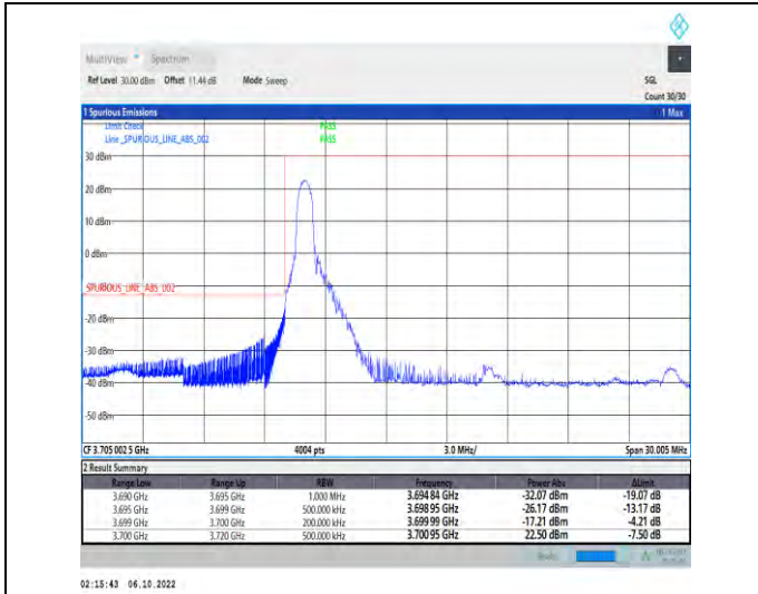
1-N77-3700-3980-PC2-30-20-L-1-DFT-QPSK-Edge_1 RB_Left-1@0-Ant1-1--PASS-see graph
