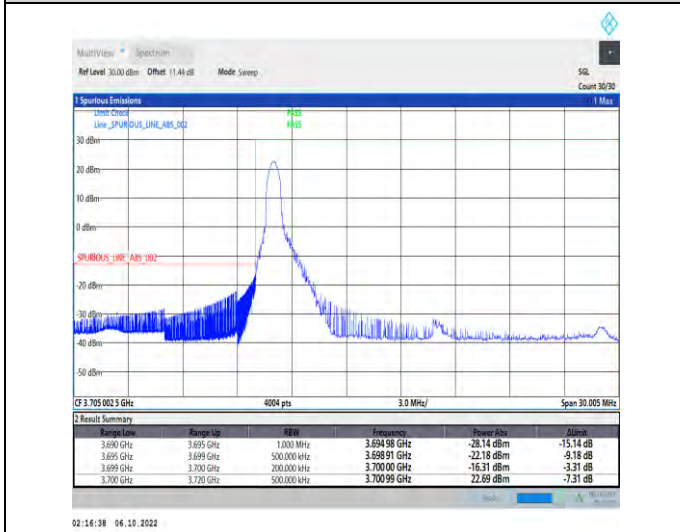
1-N77-3700-3980-PC2-30-20-L-4-CP-QPSK-Edge_1R B_Left-1@0-Ant1-1--PASS-see graph
