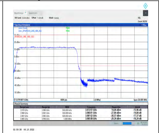
1-N77-3700-3980-PC2-30-10-H-3-DFT-QPSK-Out er_Full-24@0-Ant1-1--PASS-see graph
