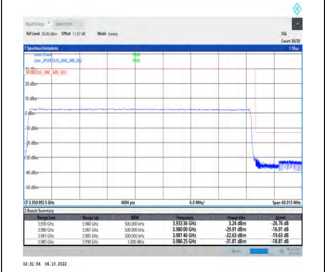
1-N77-3700-3980-PC2-30-50-H-6-CP-QPSK-Outer _Full-133@0-Ant1-1--PASS-see graph
