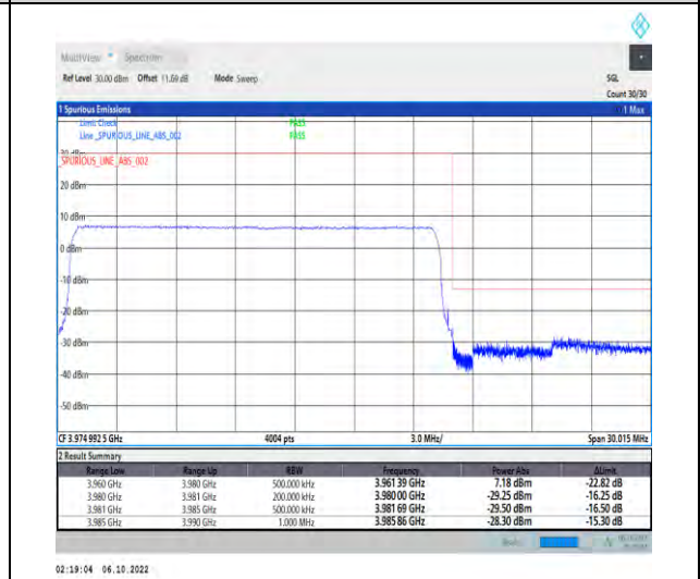
1-N77-3700-3980-PC2-30-20-H-6-CP-QPSK-Outer _Full-51@0-Ant1-1--PASS-see graph
