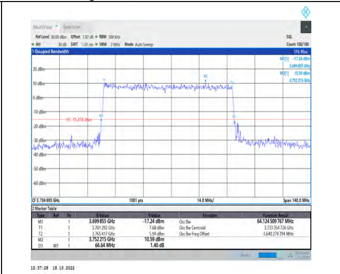
1-N77-3700-3980-PC2-30-70-L-3-DFT-16QAM-Outer_Full-180@0-Ant1-64.125-66.640-≤70-PASS
