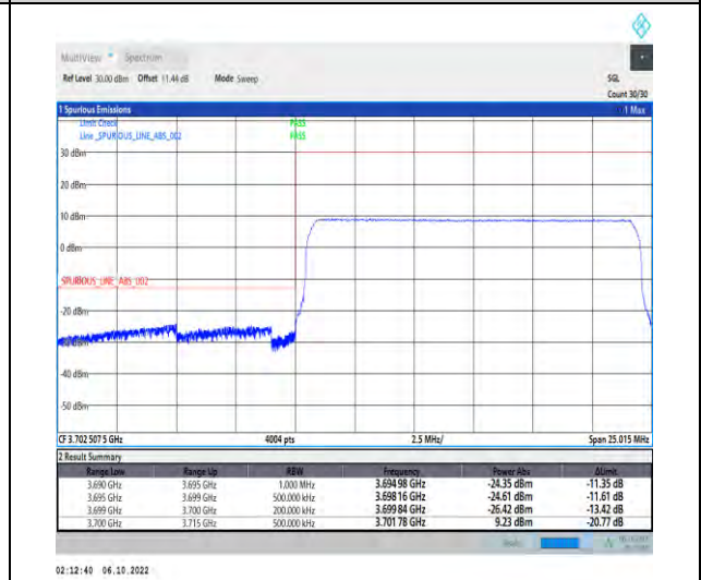
1-N77-3700-3980-PC2-30-15-L-6-CP-QPSK-Outer_Full-38@0-Ant1-1--PASS-see graph
