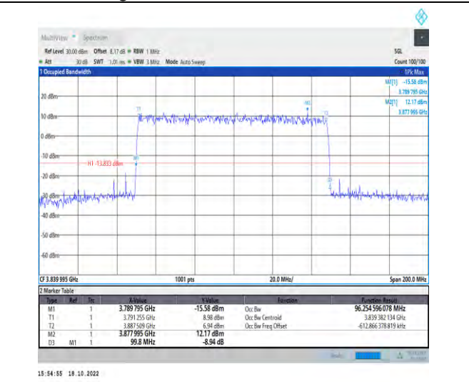
1-N77-3700-3980-PC2-30-100-M-3-DFT-16QAM-Out er_Full-270@0-Ant1-96.255-99.800-≤100-PASS
