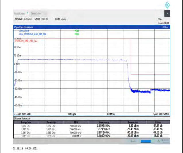
1-N77-3700-3980-PC2-30-30-H-6-CP-QPSK-Out er_Full-78@0-Ant1-1--PASS-see graph
