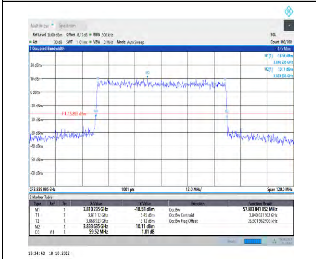
1-N77-3700-3980-PC2-30-60-M-8-CP-64QAM-Outer_Full-162@0-Ant1-57.804-59.520-≤60-PASS
