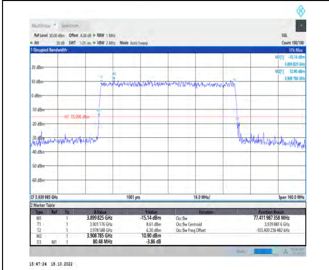
1-N77-3700-3980-PC2-30-80-H-8-CP-64QAM-Outer_Full-217@0-Ant1-77.412-80.480-≤80-PASS
