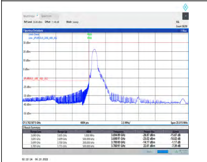
1-N77-3700-3980-PC2-30-15-L-4-CP-QPSK-Edge_1R B_Left-1@0-Ant1-1--PASS-see graph
