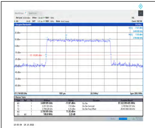
1-N77-3700-3980-PC2-30-100-L-6-CP-QPSK-Outer_Full-273@0-Ant1-97.322-100.800-≤100-PASS
