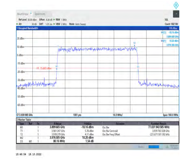
1-N77-3700-3980-PC2-30-80-H-5-DFT-256QAM-Outer_Full-216@0-Ant1-77.032-80.160-≤80-PASS
