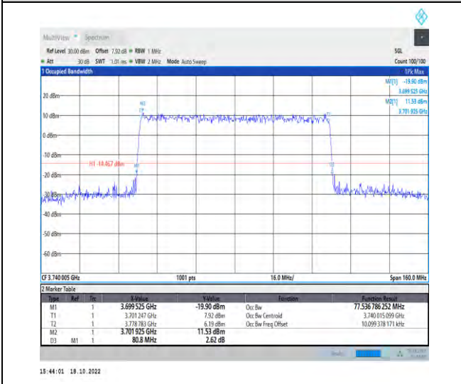
1-N77-3700-3980-PC2-30-80-L-8-CP-64QAM-Outer_Full-217@0-Ant1-77.537-80.800-<math>\leq 80</math>-PASS
