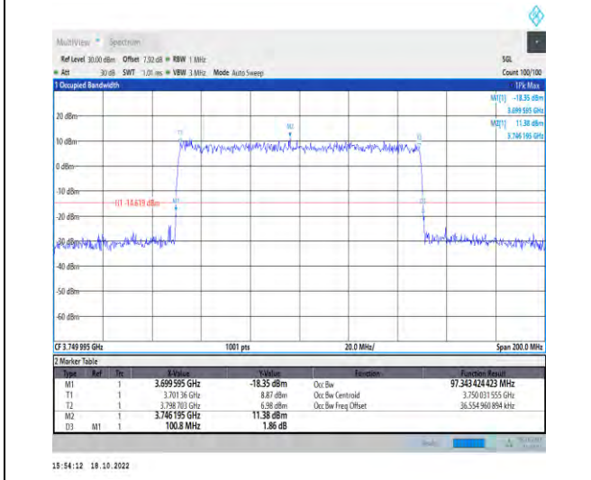
1-N77-3700-3980-PC2-30-100-L-8-CP-64QAM-Outer_Full-273@0-Ant1-97.343-100.800-≤100-PASS
