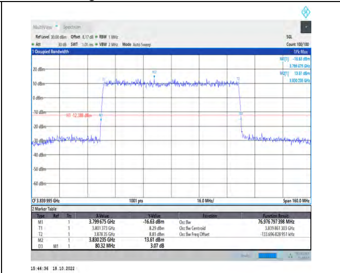
1-N77-3700-3980-PC2-30-80-M-3-DFT-16QAM-Outer_Full-216@0-Ant1-76.977-80.320-≤80-PASS
