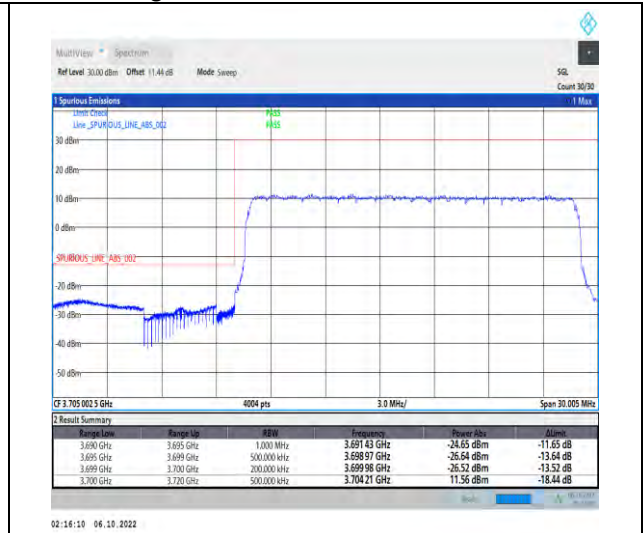
1-N77-3700-3980-PC2-30-20-L-3-DFT-QPSK-Outer_Full-50@0-Ant1-1--PASS-see graph
