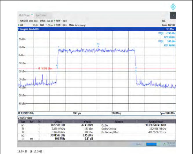
1-N77-3700-3980-PC2-30-100-H-5-DFT-256QAM-Outer_Full-270@0-Ant1-95.999-99.800-≤100-PASS
