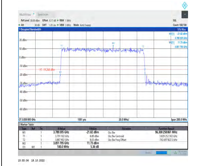
1-N77-3700-3980-PC2-30-100-M-4-DFT-64QAM-Out er_Full-270@0-Ant1-96.3-100.000-≤100-PASS
