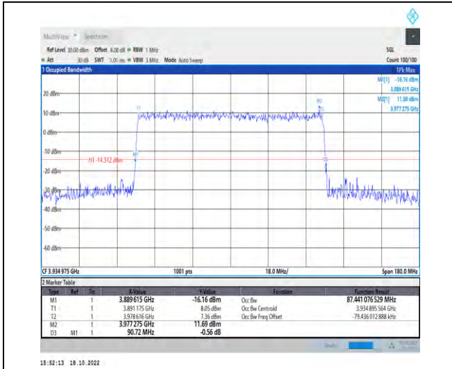
1-N77-3700-3980-PC2-30-90-H-6-CP-QPSK-Outer_Full-245@0-Ant1-87.441-90.720-≤90-PASS
