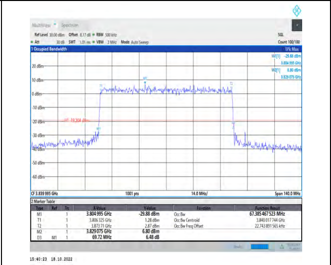
1-N77-3700-3980-PC2-30-70-M-9-CP-256QAM-Outer_Full-189@0-Ant1-67.385-69.720-≤70-PASS
