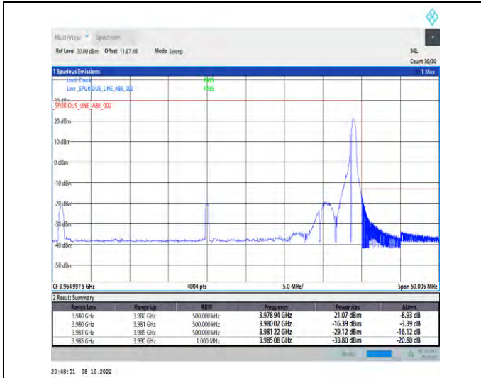
1-N77-3700-3980-PC2-30-40-H-2-DFT-QPSK-Edge_1 RB_Right-1@105-Ant1-1--PASS-see graph
