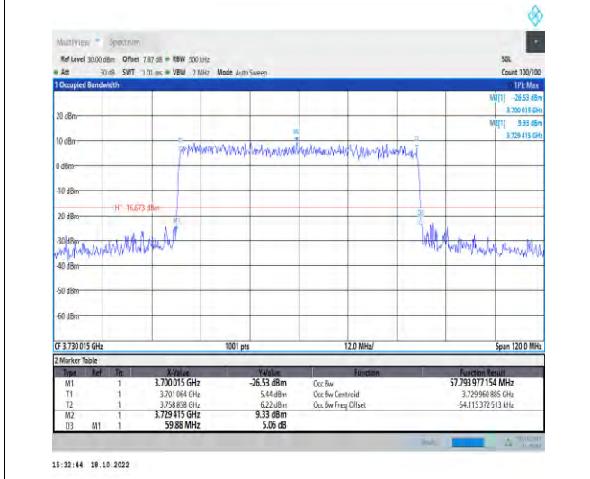
1-N77-3700-3980-PC2-30-60-L-8-CP-64QAM-Outer_Full-162@0-Ant1-57.794-59.880-≤60-PASS
