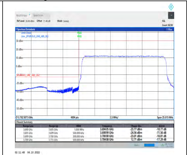
1-N77-3700-3980-PC2-30-15-L-3-DFT-QPSK-Outer_Full-36@0-Ant1-1--PASS-see graph
