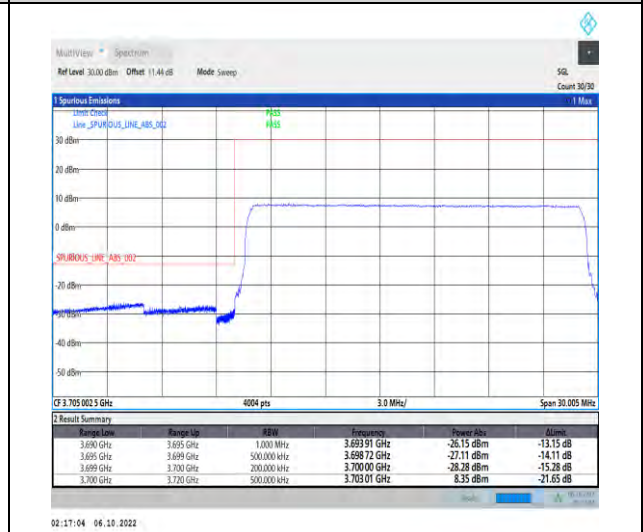
1-N77-3700-3980-PC2-30-20-L-6-CP-QPSK-Outer_Full-51@0-Ant1-1--PASS-see graph
