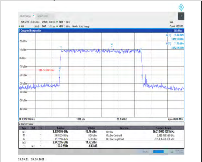
1-N77-3700-3980-PC2-30-100-H-3-DFT-16QAM-Outer_Full-270@0-Ant1-96.212-100.000-≤100-PASS
