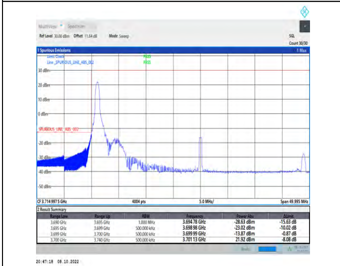
1-N77-3700-3980-PC2-30-40-L-4-CP-QPSK-Edge_1R B_Left-1@0-Ant1-1--PASS-see graph
