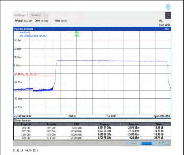
1-N77-3700-3980-PC2-30-30-L-6-CP-QPSK-Outer_Full-78@0-Ant1-1--PASS-see graph
