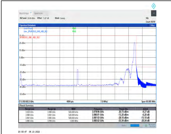
1-N77-3700-3980-PC2-30-60-H-2-DFT-QPSK-Edge_1 RB_Right-1@161-Ant1-1--PASS-see graph
