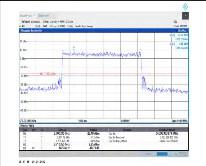
1-N77-3700-3980-PC2-30-70-L-5-DFT-256QAM-Outer_Full-180@0-Ant1-64.296-66.500-≤70-PASS
