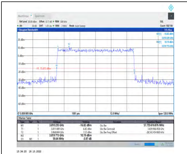
1-N77-3700-3980-PC2-30-60-M-6-CP-QPSK-Outer_Full-162@0-Ant1-57.756-59.640-≤60-PASS
