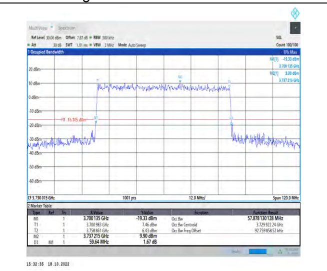
1-N77-3700-3980-PC2-30-60-L-7-CP-16QAM-Outer_Full-162@0-Ant1-57.878-59.640-≤60-PASS
