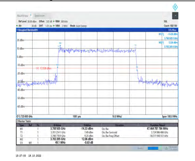
1-N77-3700-3980-PC2-30-50-L-7-CP-16QAM-Outer _Full-133@0-Ant1-47.465-49.100-≤50-PASS
