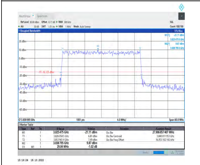
1-N77-3700-3980-PC2-30-30-M-8-CP-64QAM-Outer_Full-78@0-Ant1-27.907-29.040-≤30-PASS
