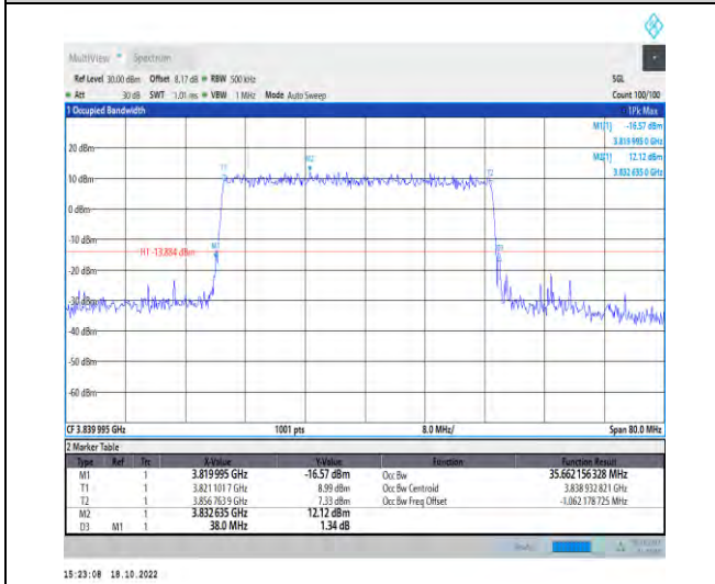
1-N77-3700-3980-PC2-30-40-M-4-DFT-64QAM-Outer_Full-100@0-Ant1-35.662-38.000-≤40-PASS
