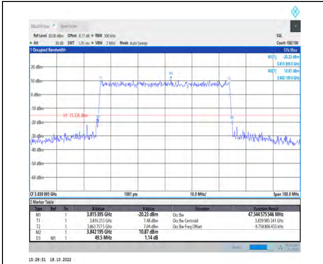
1-N77-3700-3980-PC2-30-50-M-6-CP-QPSK-Outer_Full-133@0-Ant1-47.545-49.500-≤50-PASS
