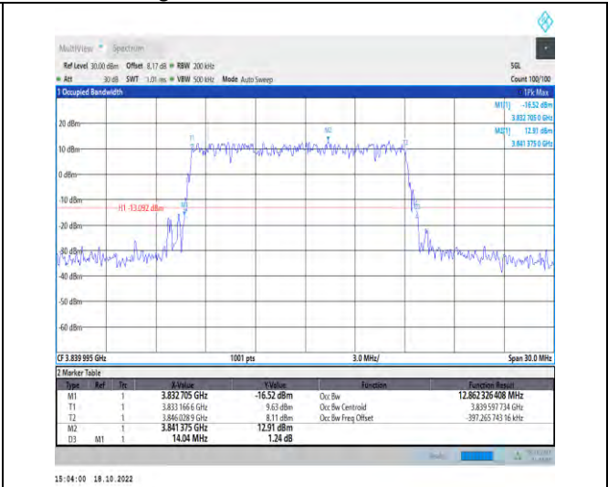
1-N77-3700-3980-PC2-30-15-M-3-DFT-16QAM-Outer_Full-36@0-Ant1-12.862-14.040-≤15-PASS
