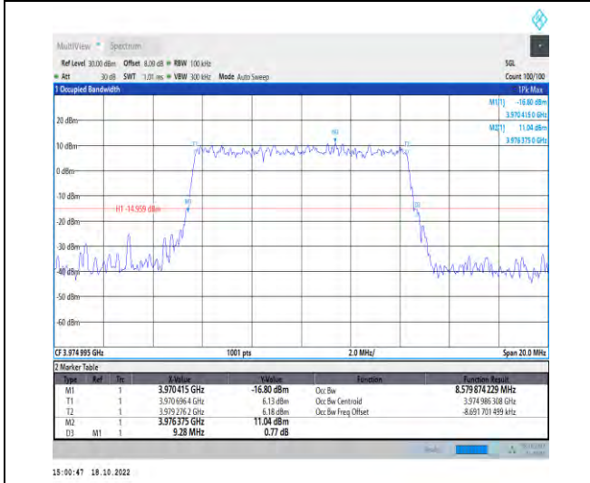
1-N77-3700-3980-PC2-30-10-H-4-DFT-64QAM-Outer_Full-24@0-Ant1-8.58-9.280-≤10-PASS
