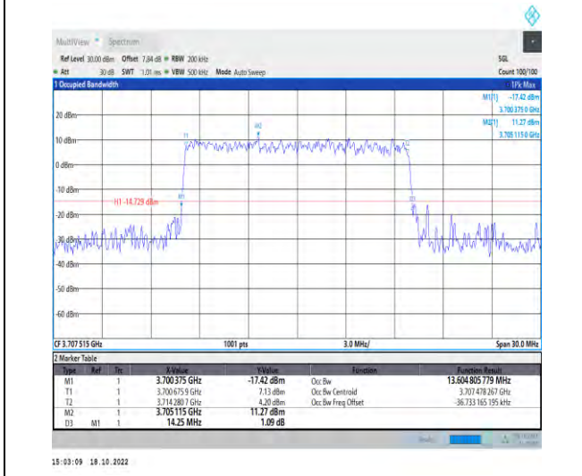
1-N77-3700-3980-PC2-30-15-L-8-CP-64QAM-Outer_Full-38@0-Ant1-13.605-14.250-≤15-PASS
