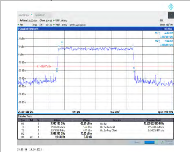
1-N77-3700-3980-PC2-30-50-H-7-CP-16QAM-Outer_Full-133@0-Ant1-47.56-49.400-≤50-PASS
