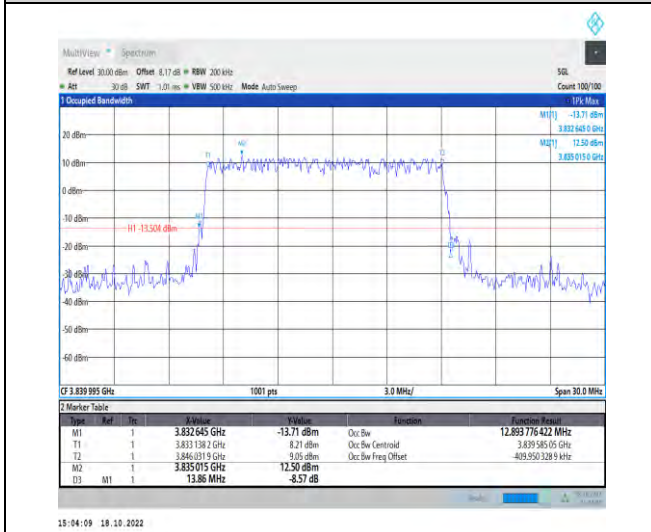
1-N77-3700-3980-PC2-30-15-M-4-DFT-64QAM-Outer_Full-36@0-Ant1-12.894-13.860-≤15-PASS
