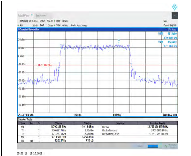
1-N77-3700-3980-PC2-30-15-L-1-DFT-QPSK-Outer_Full-36@0-Ant1-12.8-13.620-≤15-PASS
