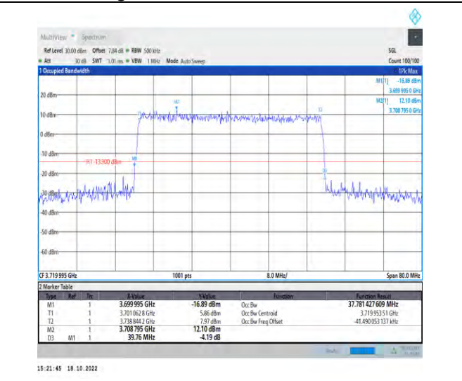
1-N77-3700-3980-PC2-30-40-L-7-CP-16QAM-Outer_Full-106@0-Ant1-37.781-39.760-≤40-PASS
