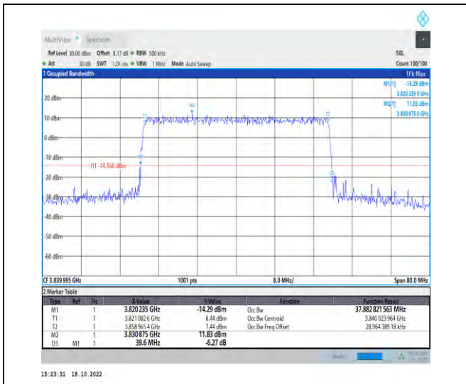
1-N77-3700-3980-PC2-30-40-M-6-CP-QPSK-Outer_Full-106@0-Ant1-37.883-39.600-≤40-PASS
