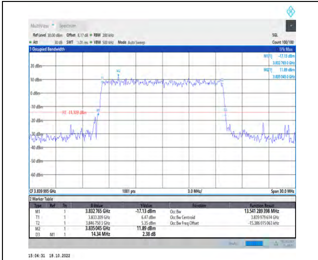
1-N77-3700-3980-PC2-30-15-M-6-CP-QPSK-Outer_Full-38@0-Ant1-13.541-14.340-≤15-PASS
