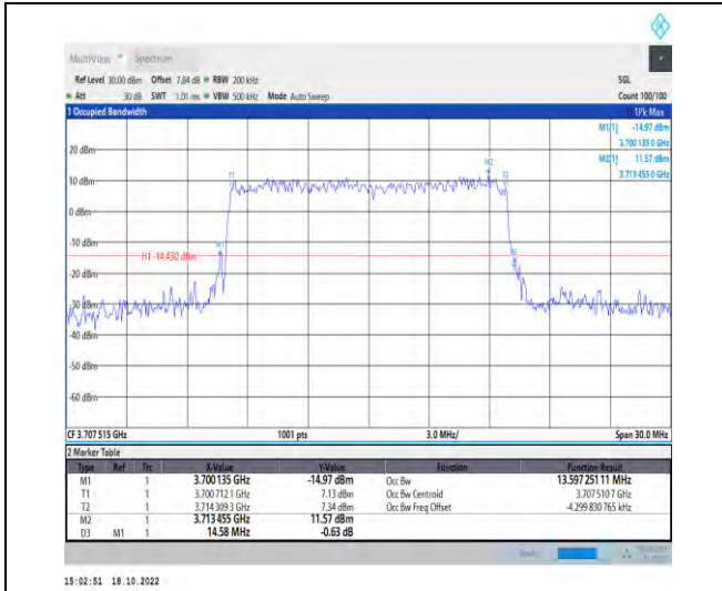
1-N77-3700-3980-PC2-30-15-L-6-CP-QPSK-Outer_Full-38@0-Ant1-13.597-14.580-≤15-PASS
