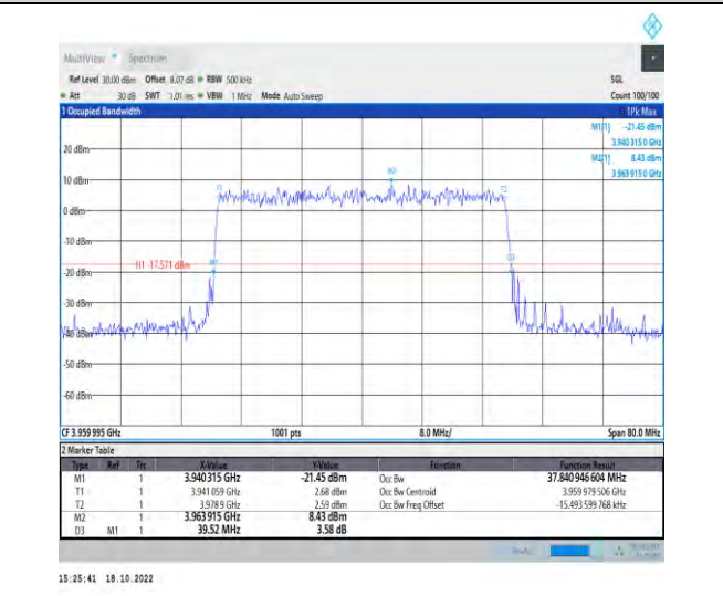
1-N77-3700-3980-PC2-30-40-H-9-CP-256QAM-Outer_Full-106@0-Ant1-37.841-39.520-≤40-PASS
