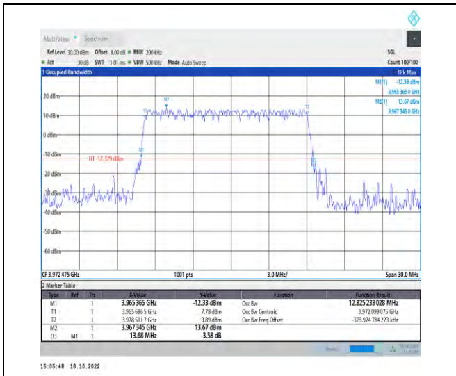
1-N77-3700-3980-PC2-30-15-H-1-DFT-QPSK-Outer_Full-36@0-Ant1-12.825-13.680-≤15-PASS
