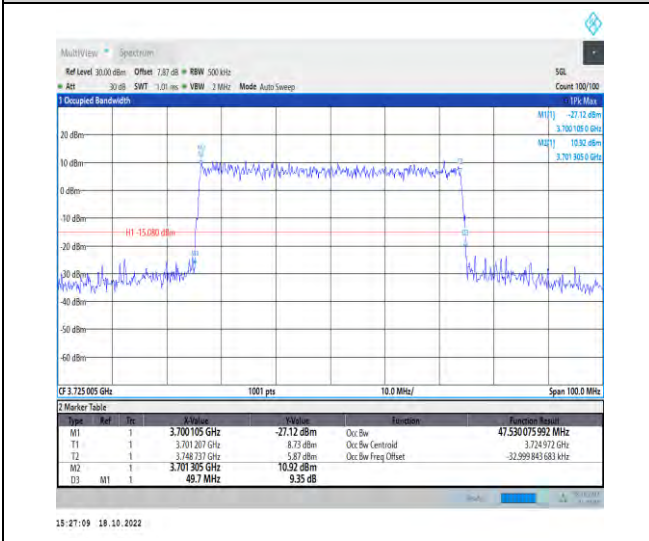
1-N77-3700-3980-PC2-30-50-L-8-CP-64QAM-Outer _Full-133@0-Ant1-47.53-49.700-≤50-PASS
