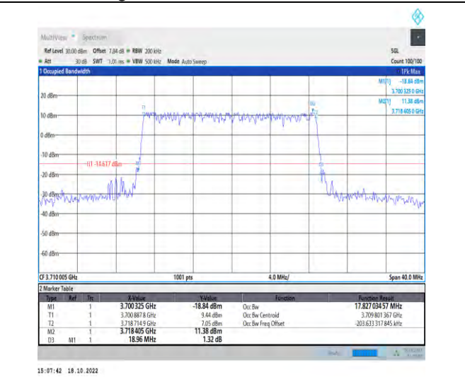
1-N77-3700-3980-PC2-30-20-L-3-DFT-16QAM-Outer_Full-50@0-Ant1-17.827-18.960-≤20-PASS
