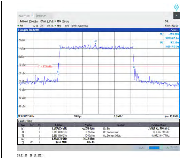
1-N77-3700-3980-PC2-30-40-M-1-DFT-QPSK-Outer_Full-100@0-Ant1-35.832-37.680-≤40-PASS
