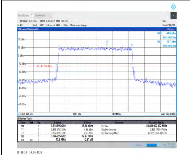
1-N77-3700-3980-PC2-30-50-M-4-DFT-64QAM-Outer_Full-128@0-Ant1-45.801-47.900-≤50-PASS
