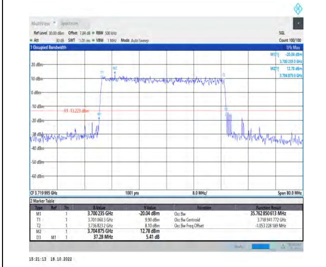
1-N77-3700-3980-PC2-30-40-L-4-DFT-64QAM-Outer_Full-100@0-Ant1-35.763-37.280-≤40-PASS
