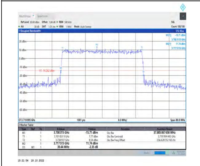
1-N77-3700-3980-PC2-30-40-L-8-CP-64QAM-Outer_Full-106@0-Ant1-37.885-39.440-≤40-PASS
