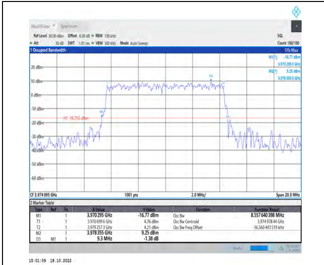
1-N77-3700-3980-PC2-30-10-H-6-CP-QPSK-Outer_Full-24@0-Ant1-8.558-9.300-≤10-PASS
