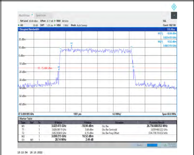
1-N77-3700-3980-PC2-30-30-M-5-DFT-256QAM-Outer_Full-75@0-Ant1-26.757-28.140-≤30-PASS
