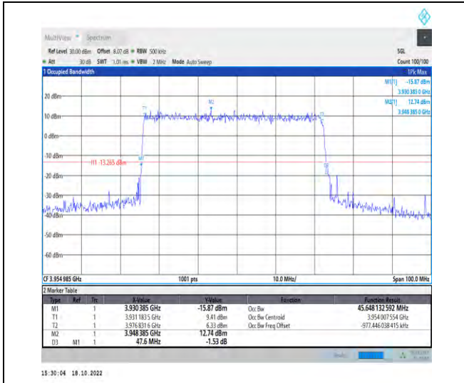
1-N77-3700-3980-PC2-30-50-H-1-DFT-QPSK-Outer_Full-128@0-Ant1-45.648-47.600-≤50-PASS
