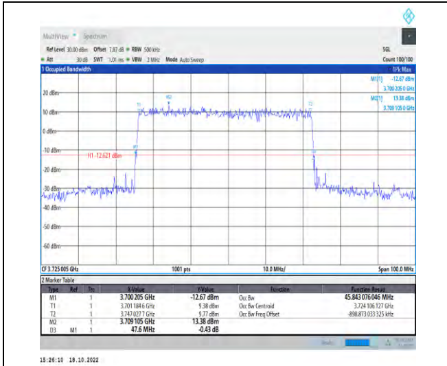
1-N77-3700-3980-PC2-30-50-L-1-DFT-QPSK-Outer_Full-128@0-Ant1-45.843-47.600-≤50-PASS
