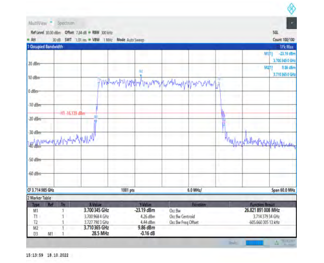
1-N77-3700-3980-PC2-30-30-L-5-DFT-256QAM-Outer_Full-75@0-Ant1-26.822-28.500-≤30-PASS
