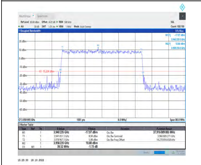
1-N77-3700-3980-PC2-30-40-H-8-CP-64QAM-Outer_Full-106@0-Ant1-37.916-39.520-≤40-PASS
