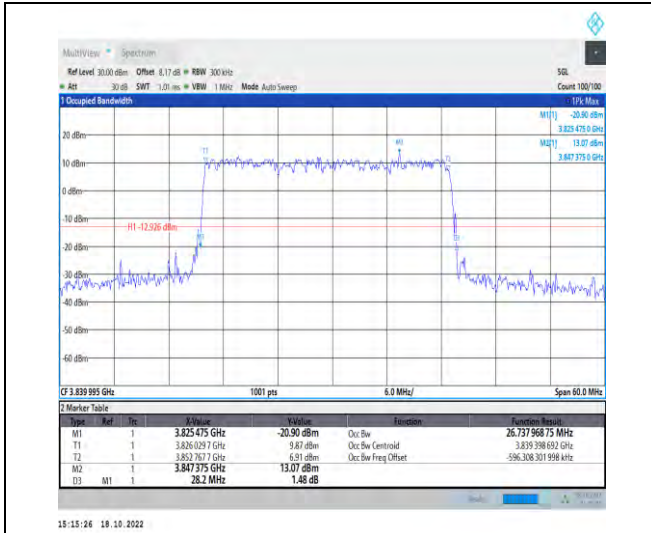
1-N77-3700-3980-PC2-30-30-M-1-DFT-QPSK-Outer_Full-75@0-Ant1-26.738-28.200-≤30-PASS
