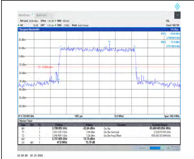
1-N77-3700-3980-PC2-30-50-L-4-DFT-64QAM-Outer_Full-128@0-Ant1-45.669-47.800-≤50-PASS
