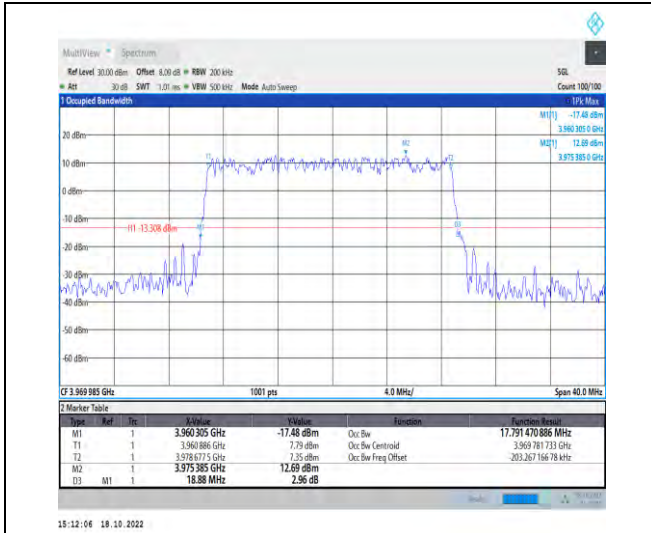
1-N77-3700-3980-PC2-30-20-H-1-DFT-QPSK-Outer_Full-50@0-Ant1-17.791-18.880-≤20-PASS
