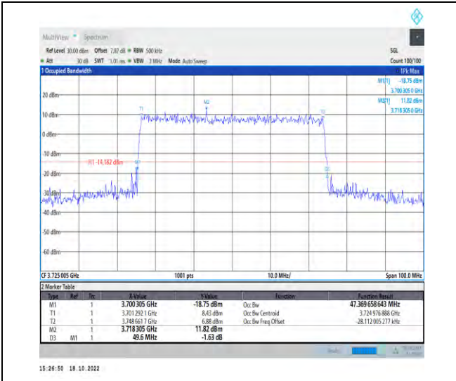
1-N77-3700-3980-PC2-30-50-L-6-CP-QPSK-Outer _Full-133@0-Ant1-47.37-49.600-≤50-PASS
