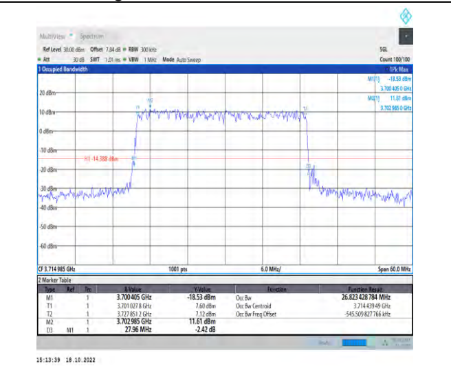
1-N77-3700-3980-PC2-30-30-L-3-DFT-16QAM-Outer_Full-75@0-Ant1-26.823-27.960-≤30-PASS
