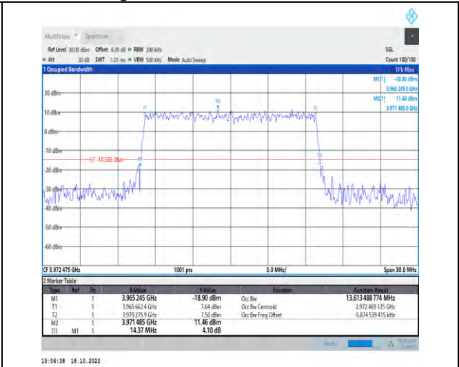
1-N77-3700-3980-PC2-30-15-H-7-CP-16QAM-Outer_Full-38@0-Ant1-13.613-14.370-≤15-PASS
