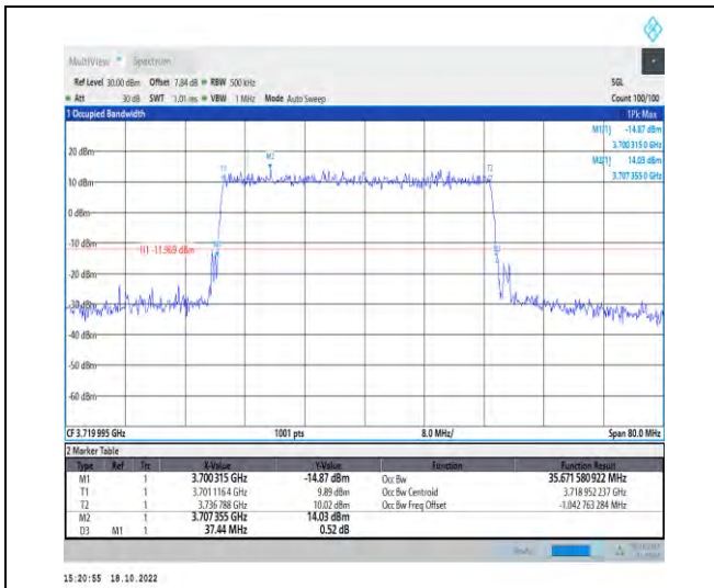
1-N77-3700-3980-PC2-30-40-L-1-DFT-QPSK-Outer_Full-100@0-Ant1-35.672-37.440-≤40-PASS
