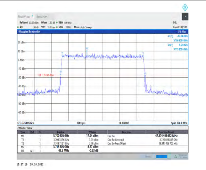
1-N77-3700-3980-PC2-30-50-L-9-CP-256QAM-Outer _Full-133@0-Ant1-47.374-49.500-≤50-PASS
