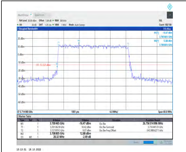
1-N77-3700-3980-PC2-30-30-L-1-DFT-QPSK-Outer_Full-75@0-Ant1-26.757-28.320-≤30-PASS
