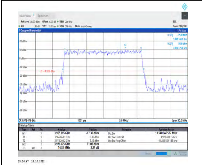
1-N77-3700-3980-PC2-30-15-H-8-CP-64QAM-Outer_Full-38@0-Ant1-13.54-14.310-≤15-PASS
