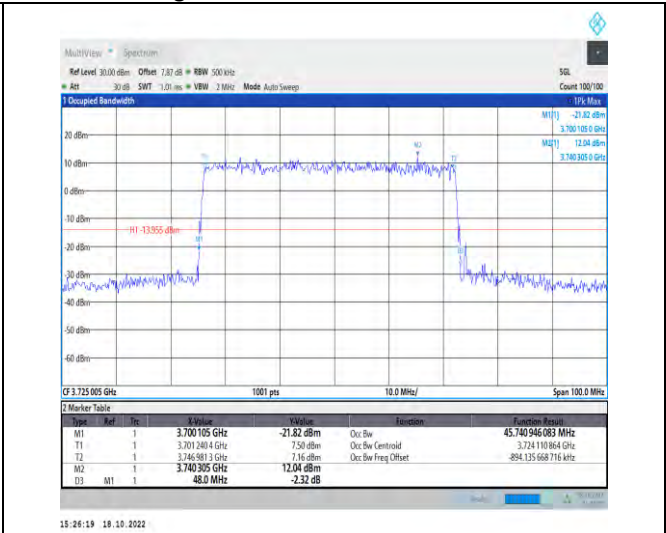
1-N77-3700-3980-PC2-30-50-L-3-DFT-16QAM-Outer_Full-128@0-Ant1-45.741-48.000-≤50-PASS
