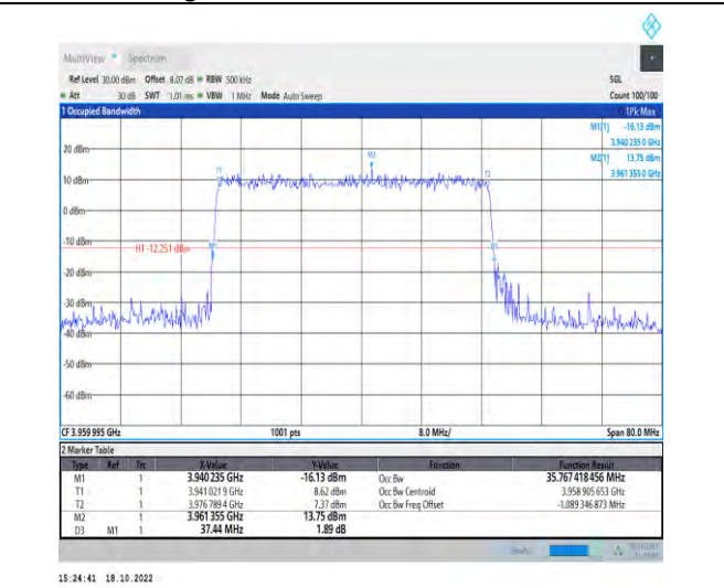
1-N77-3700-3980-PC2-30-40-H-3-DFT-16QAM-Outer_Full-100@0-Ant1-35.767-37.440-≤40-PASS
