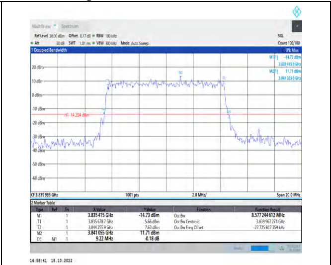
1-N77-3700-3980-PC2-30-10-M-3-DFT-16QAM-Outer_Full-24@0-Ant1-8.577-9.220-≤10-PASS
