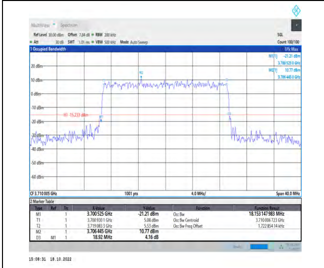
1-N77-3700-3980-PC2-30-20-L-8-CP-64QAM-Outer_Full-51@0-Ant1-18.153-18.920-≤20-PASS
