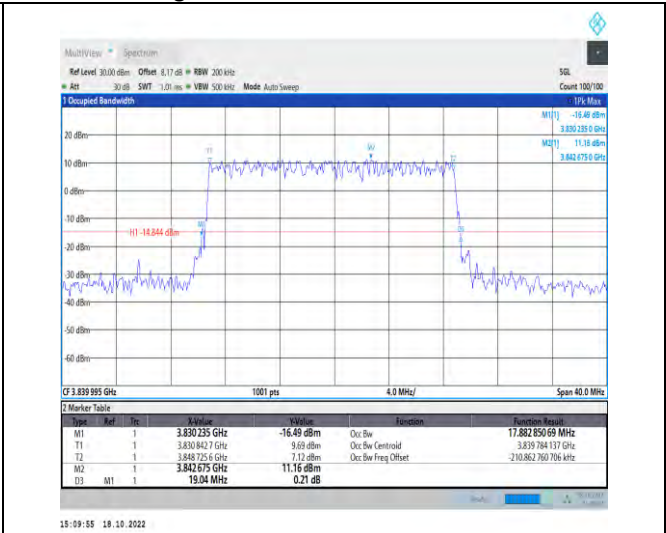
1-N77-3700-3980-PC2-30-20-M-3-DFT-16QAM-Outer_Full-50@0-Ant1-17.883-19.040-≤20-PASS
