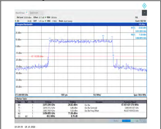
1-N77-3700-3980-PC2-30-50-M-7-CP-16QAM-Outer_Full-133@0-Ant1-47.452-49.300-≤50-PASS
