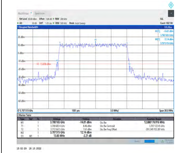
1-N77-3700-3980-PC2-30-15-L-4-DFT-64QAM-Outer_Full-36@0-Ant1-12.88-13.830-≤15-PASS
