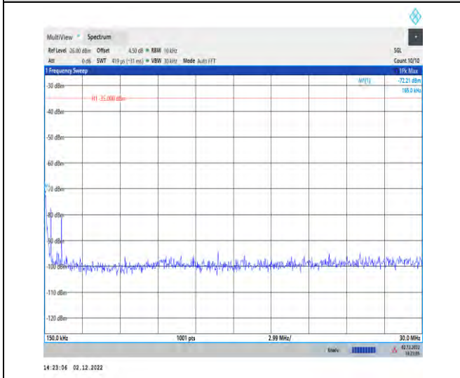
1-41-41-30-100-M-1-DFT-QPSK-Inner_1RB_Left-1 @1-0.15-30
