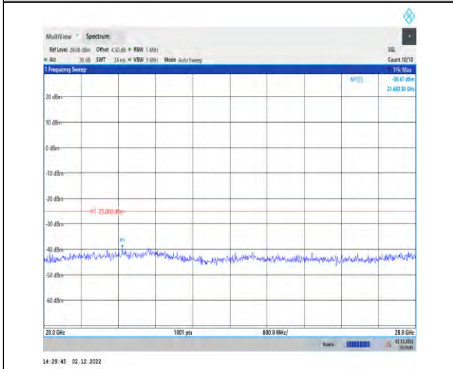
1-41-41-30-100-H-1-DFT-QPSK-Inner_1RB_Left-1@ 1-20000-28000
