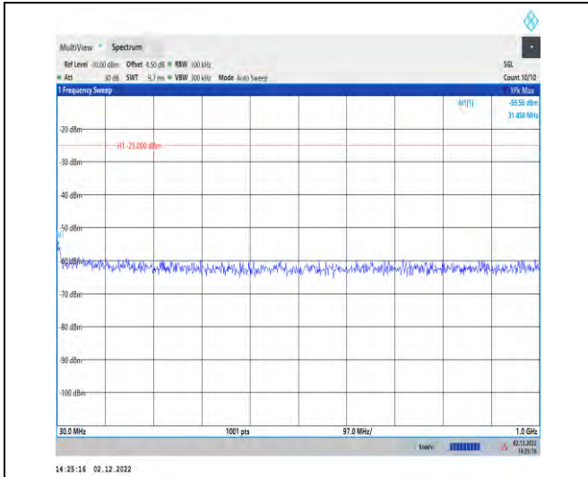
1-41-41-30-100-H-1-DFT-QPSK-Inner_1RB_Left-1@ 1-30-1000
