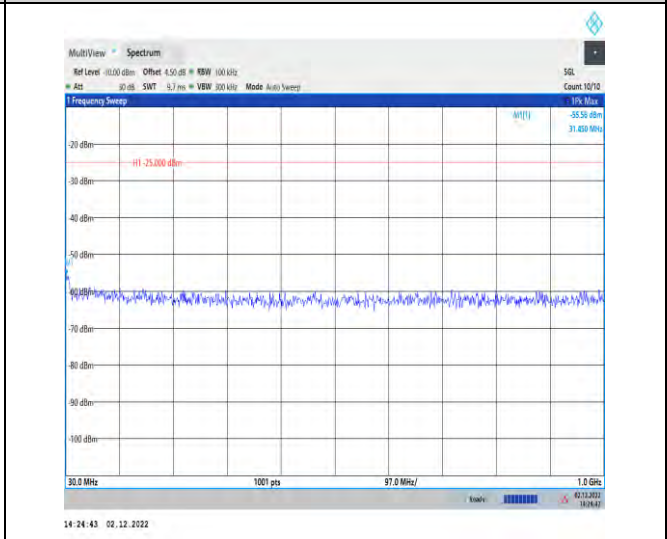
1-41-41-30-100-M-1-DFT-QPSK-Inner_1RB_Left-1@ 1-30-1000
