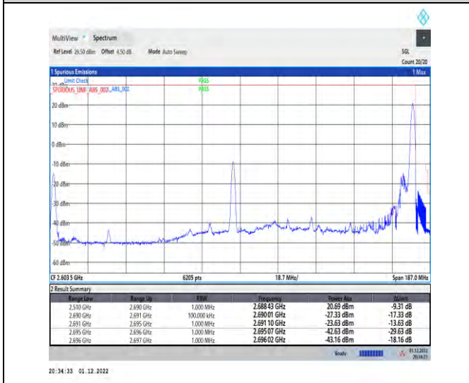
1-41-41-30-100+80-H-2-DFT-QPSK-Edge_1RB_Right
