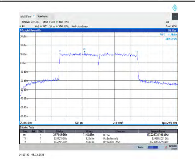
1-41-41-60+60-M-6-DFT-16QAM-Outer_Full
