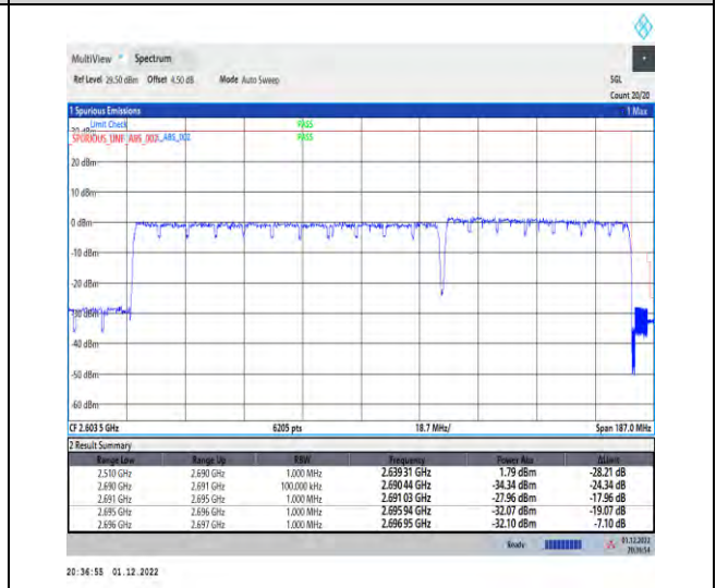
1-41-41-30-100+60-H-L-3-DFT-QPSK-Outer_Full
