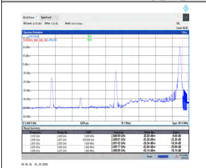
1-41-41-30-100+50-H-2-DFT-QPSK-Edge_1RB_Right
