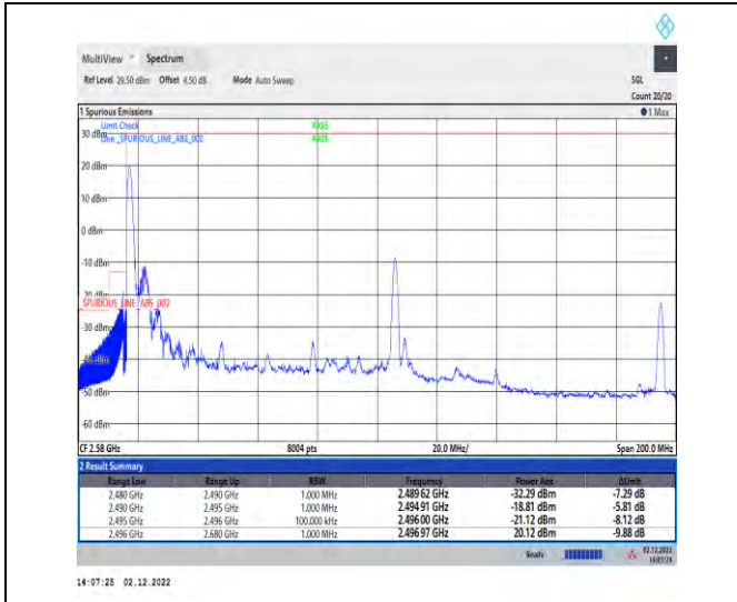
1-41-41-30-100+80-L-4-CP-QPSK-Edge_1RB_Left
