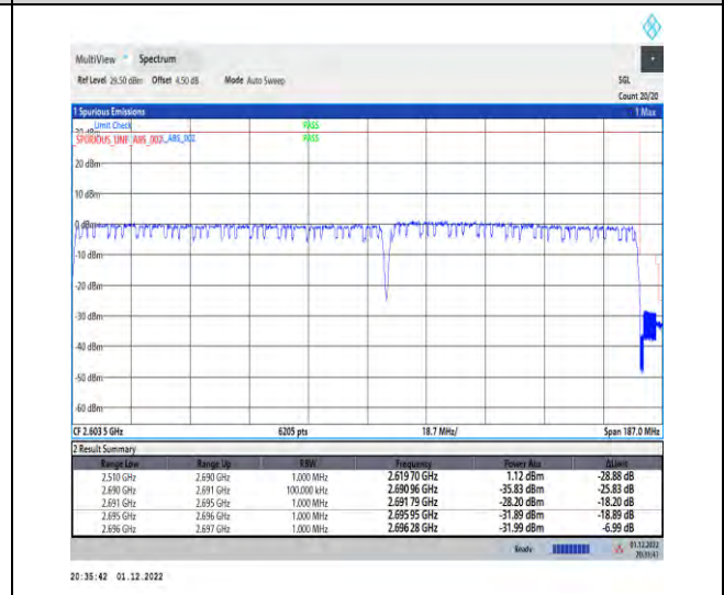
1-41-41-30-100+80-H-3-DFT-QPSK-Outer_Full
