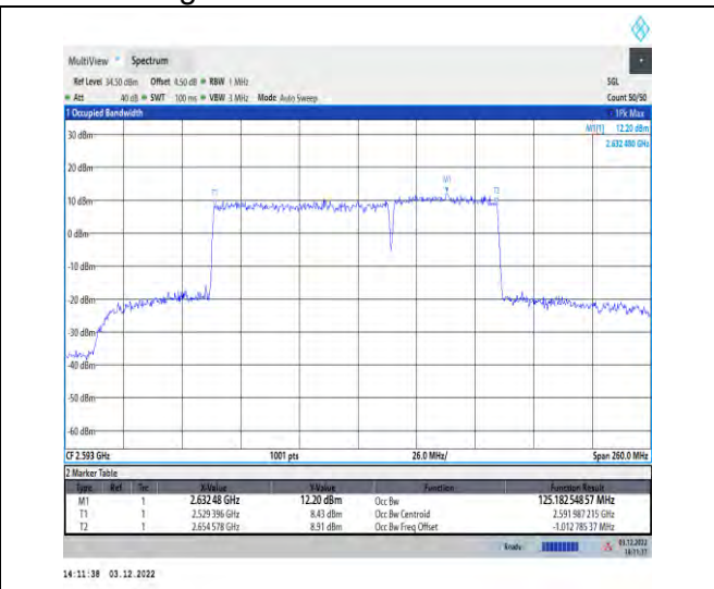
1-41-41-80+50-M-4-DFT-16QAM-Outer_Full
