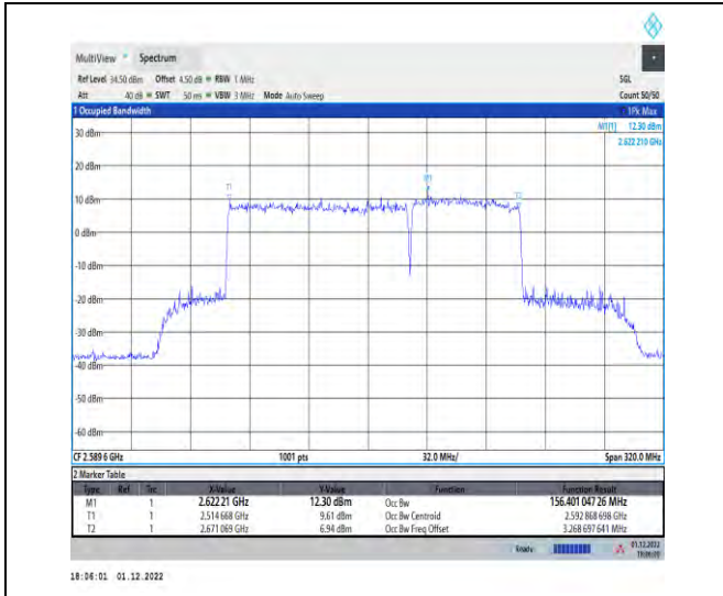
1-41-41-100+60-M-3-DFT-QPSK-Outer_Full
