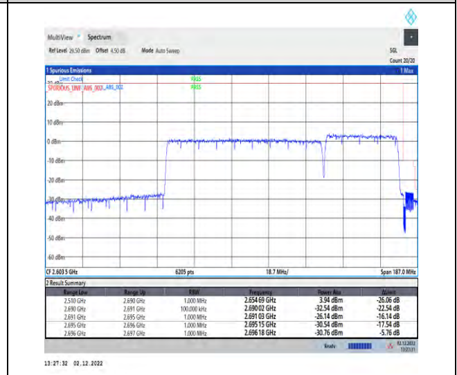
1-41-41-30-80+40-H-6-CP-QPSK-Outer_Full
