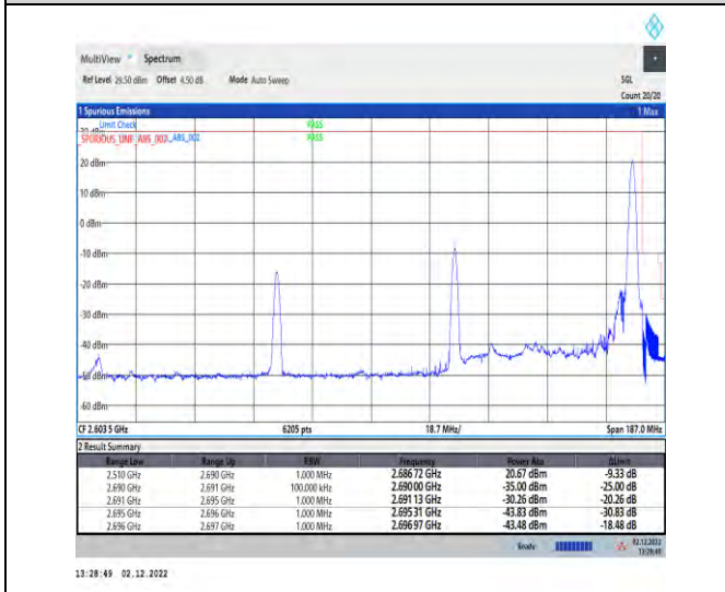
1-41-41-30-80+40-H-4-CP-QPSK-Edge_1RB_Right
