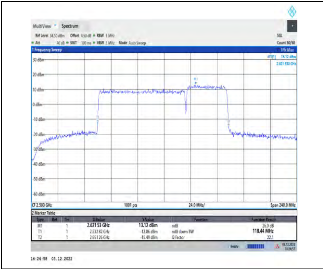
1-41-41-80+40-M-9-DFT-16QAM-Outer_Full
