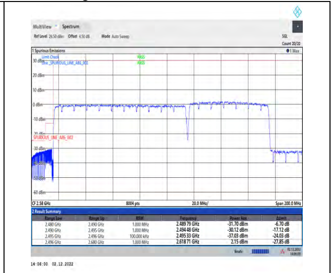
1-41-41-30-100+60-L-6-CP-QPSK-Outer_Full
