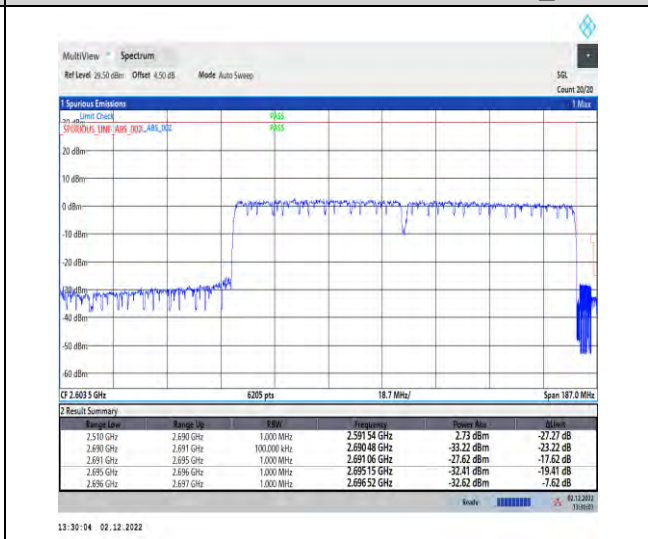
1-41-41-60+60-H-6-CP-QPSK-Outer_Full
