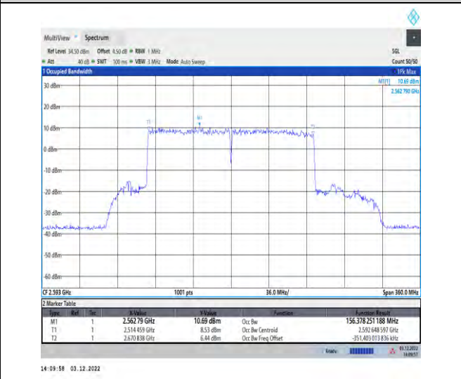
1-41-41-80+80-M-1-DFT-16QAM-Outer_Full
