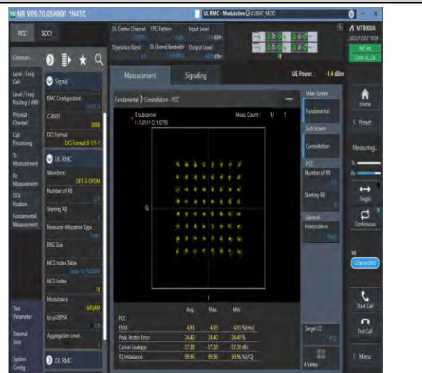
1-41-41-30-100-M-4-DFT-64QAM-Outer_Full-270@ 0-Ant1-see graph-PASS
