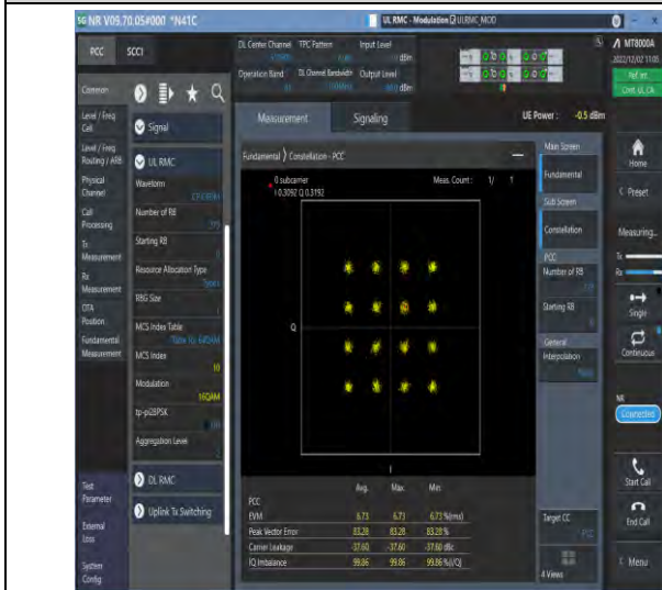
1-41-41-30-100-M-7-CP-16QAM-Outer_Full-273@0-Ant1-see graph-PASS
