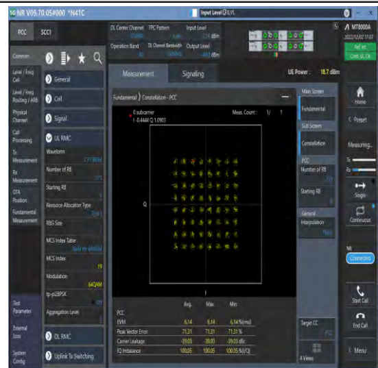
1-41-41-30-100-M-8-CP-64QAM-Outer_Full-273@0-Ant1-see graph-PASS
