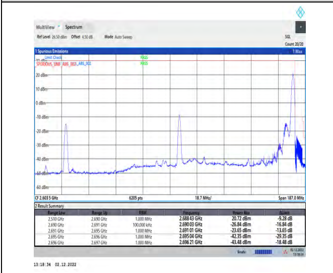
1-41-41-30-80+80-H-2-DFT-QPSK-Edge_1RB_Right
