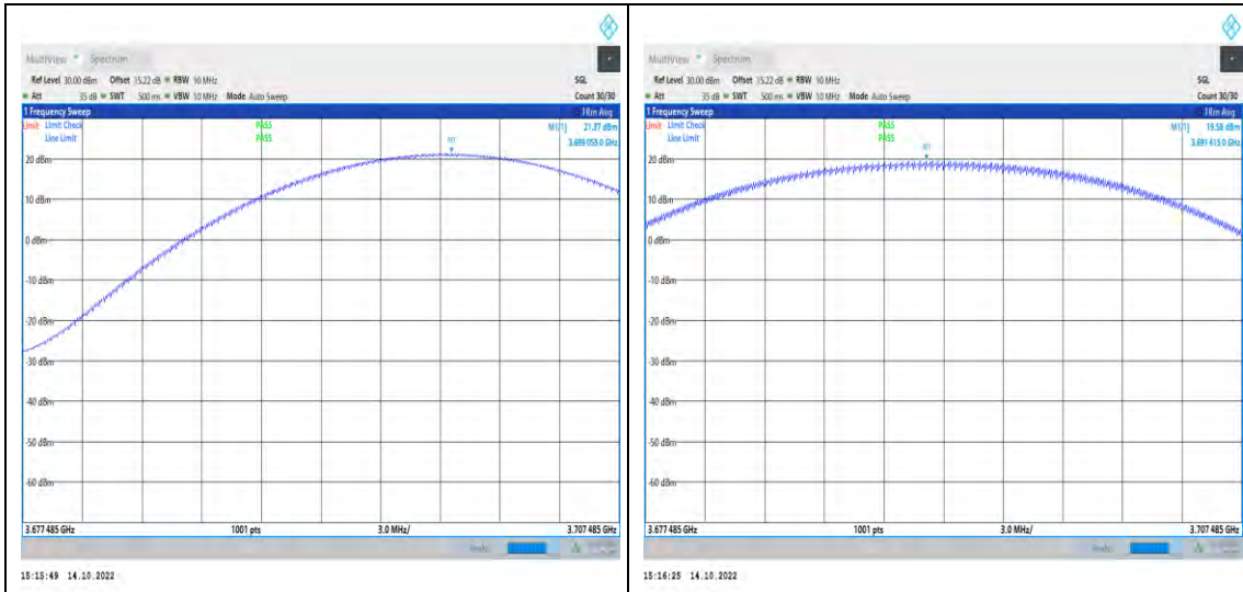
1-N48-PC3-30-15-H-5-DFT-QPSK-Inner_1RB_Right-1@ 36-3677.485-3707.485-Ant1-3690.69-21.37-99-PASS
