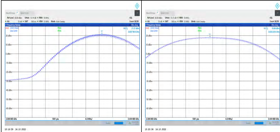
1-N48-PC3-30-20-M-5-DFT-QPSK-Inner_1RB_Right-1@ 49-3604.985-3644.985-Ant1-3630.71-21.57-99-PASS
