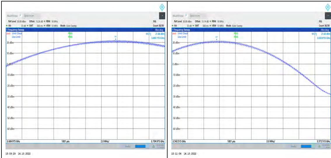
1-N48-PC3-30-10-H-5-DFT-QPSK-Inner_1RB_Right-1@ 22-3684.975-3704.975-Ant1-3703.74-21.98-99-PASS
