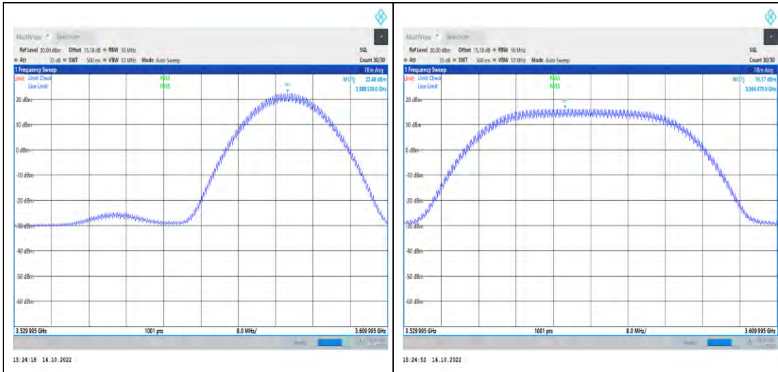
1-N48-PC3-30-40-L-5-DFT-QPSK-Inner_1RB_Right-1@ 104-3529.995-3609.995-Ant1-3588.72-22.48-99-PASS
