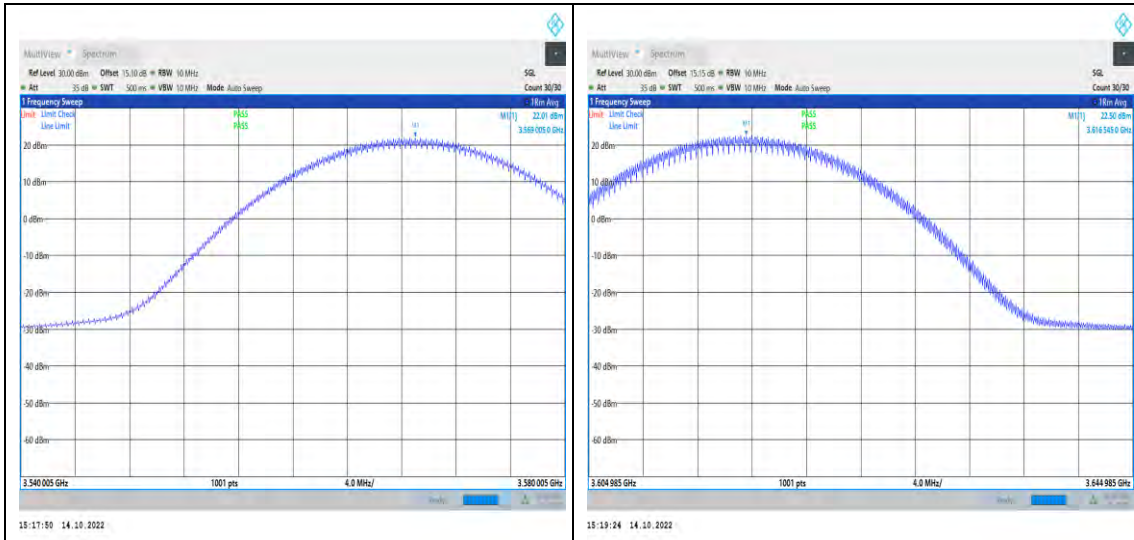
1-N48-PC3-30-20-L-5-DFT-QPSK-Inner_1RB_Right-1@ 49-3540.005-3580.005-Ant1-3566.53-22.01-99-PASS
