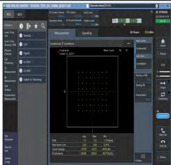
1-N48-PC3-30-40-M-4-DFT-64QAM-Outer_Full-100@0- Ant1-see graph-PASS
