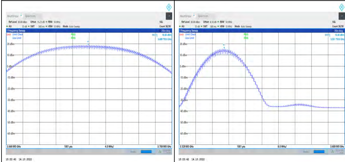
1-N48-PC3-30-20-H-6-DFT-QPSK-Outer_Full-50@0-366 9.995-3709.995-Ant1-3682.28-18.65-99-PASS
