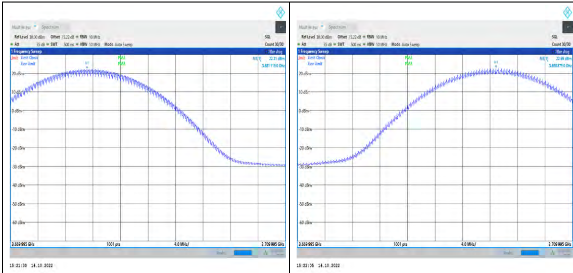
1-N48-PC3-30-20-H-4-DFT-QPSK-Inner_1RB_Left-1@1 -3669.995-3709.995-Ant1-3680.16-22.21-99-PASS
