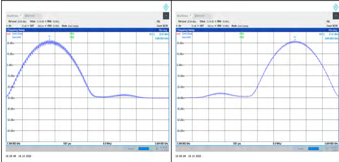
1-N48-PC3-30-40-M-4-DFT-QPSK-Inner_1RB_Left-1@1 -3584.985-3664.985-Ant1-3606.51-22.47-99-PASS
