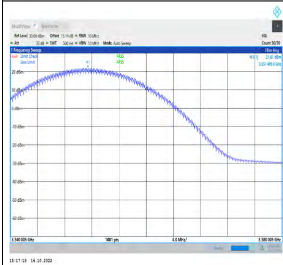
1-N48-PC3-30-20-L-4-DFT-QPSK-Inner_1RB_Left-1@1- 3540.005-3580.005-Ant1-3551.81-21.81-99-PASS
