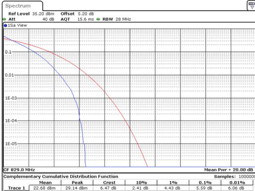
Band5-10MHz-QPSK-20450-50RB#0
