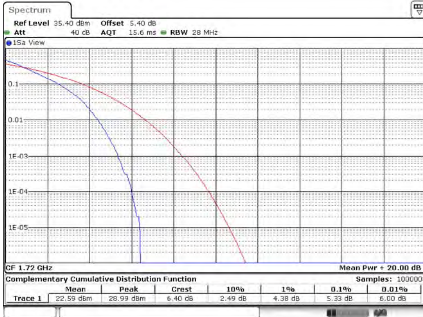
Band66-20MHz-QPSK-132072-100RB#0
