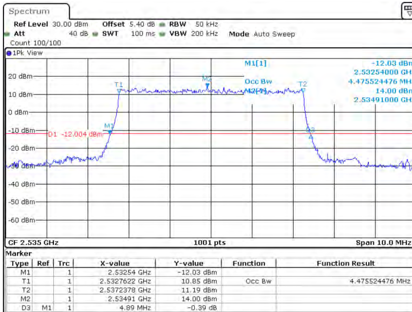
Band7-5MHz-QPSK-21100-25RB#0-4.476
