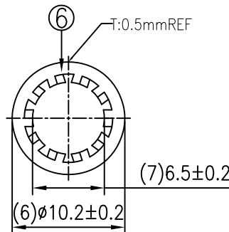
WASHER
