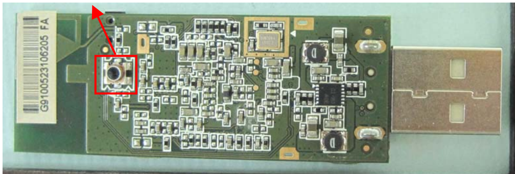
Ant. 1: TX/RX
