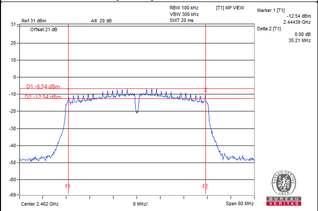
802.11n (HT40): Chain 0 / CH11
