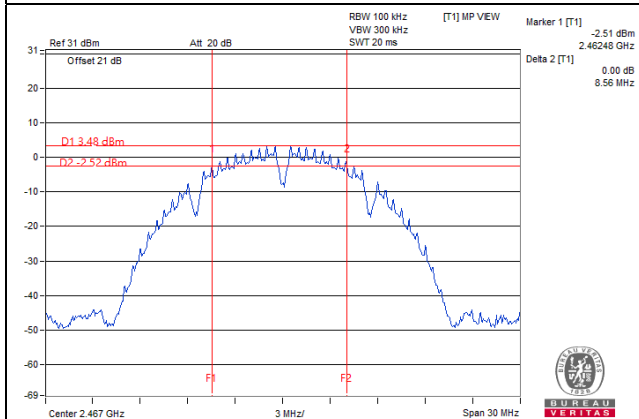
802.11n (HT20): Chain 0 / CH12
