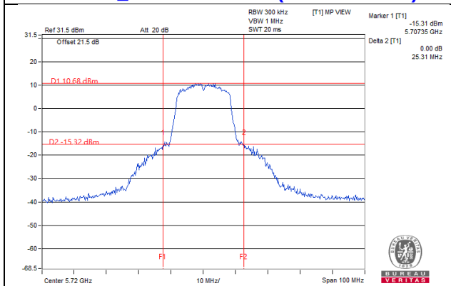
802.11a_Chain 1 / CH144 (U-NII-2C Band)
