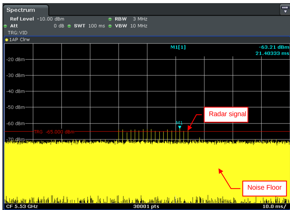
Radar Signal 0
