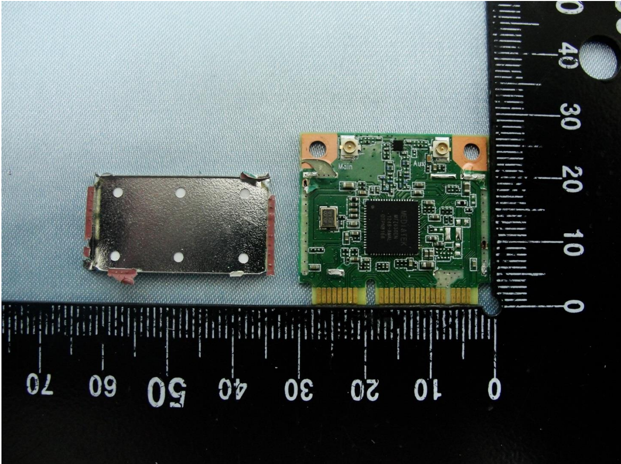
EUT: WLAN module (Brand Name: MediaTek / Model Name: MT7630E)
