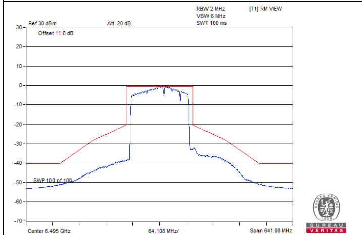
802.11be (EHT160) 996+484+242-tone MRU 1S1T / Chain 0 : CH 111
