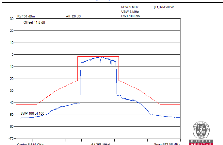
802.11be (EHT160) 996+484+242-tone MRU 1S1T / Chain 0 : CH 175
