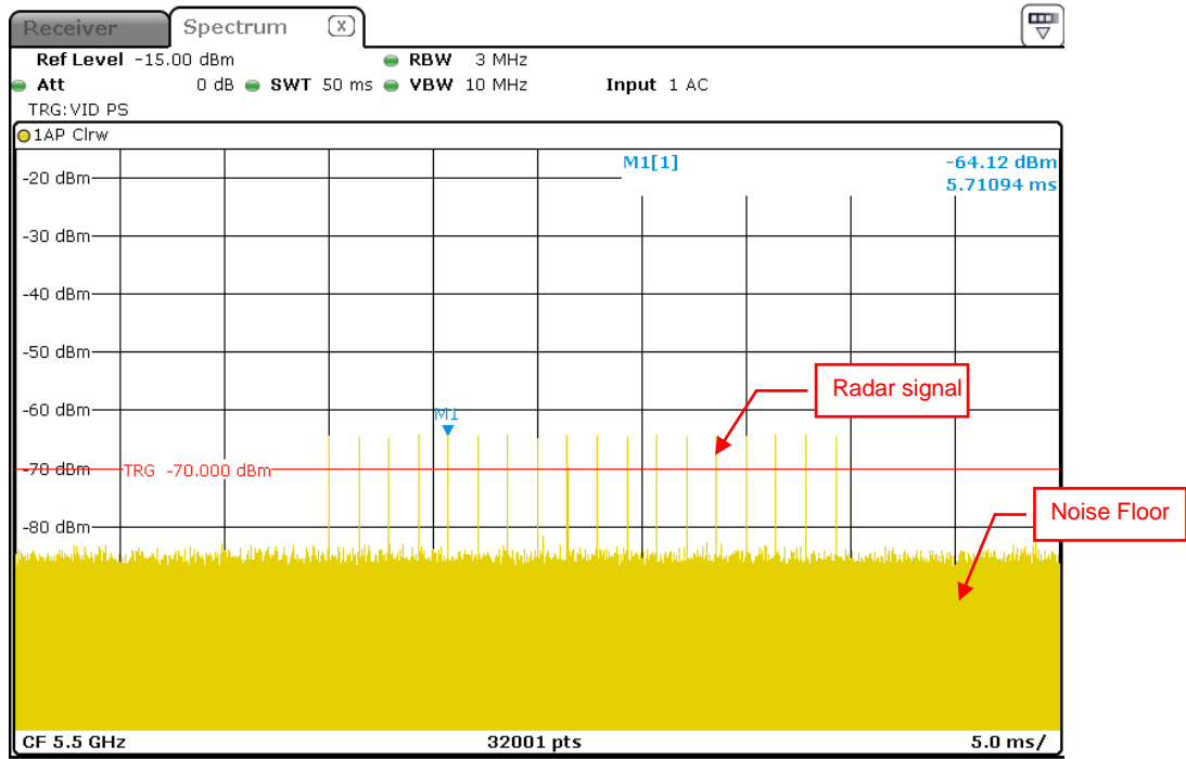
Radar Signal 0
