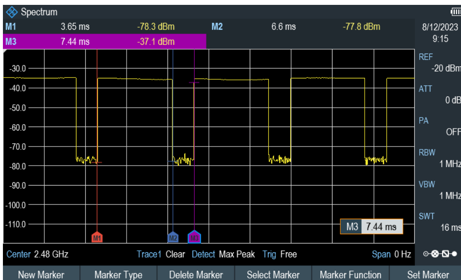
Time-domain plot for Bluetooth transmission signal
