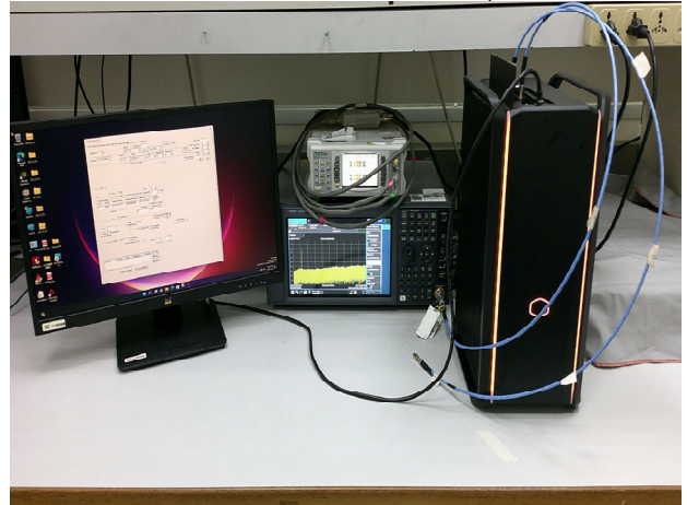
FCC_15_407_6E_Conducted_setup
