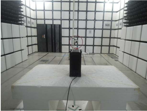
FCC_15_407_6E_Radiated_Setup
