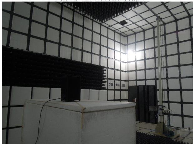
FCC_15_407_Radiated_Setup
