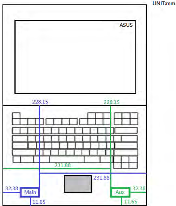
Photograph 7. Antenna position of EUT
