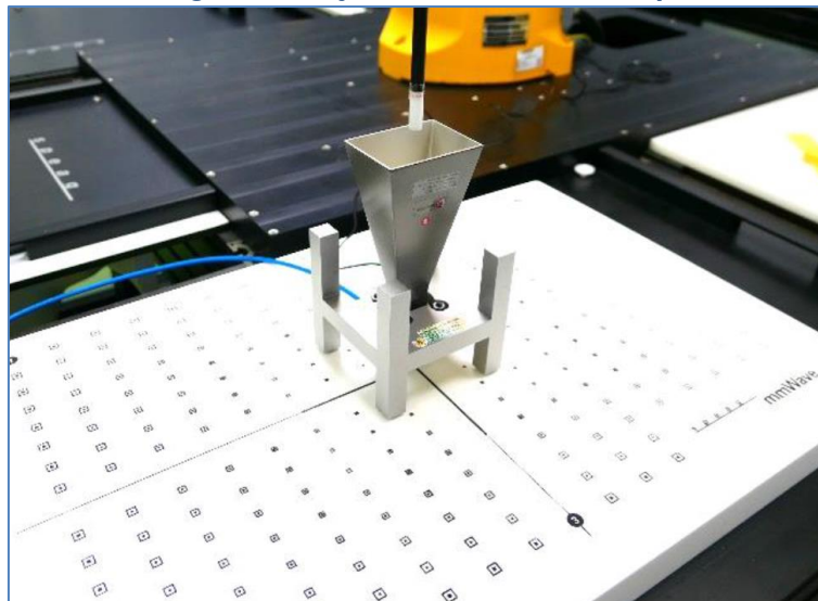
Figure 9-1: System Verification Setup
