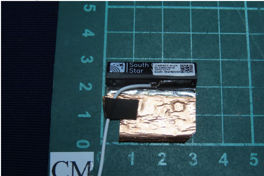
(42) EUT Photo_South Star Aux Antenna
