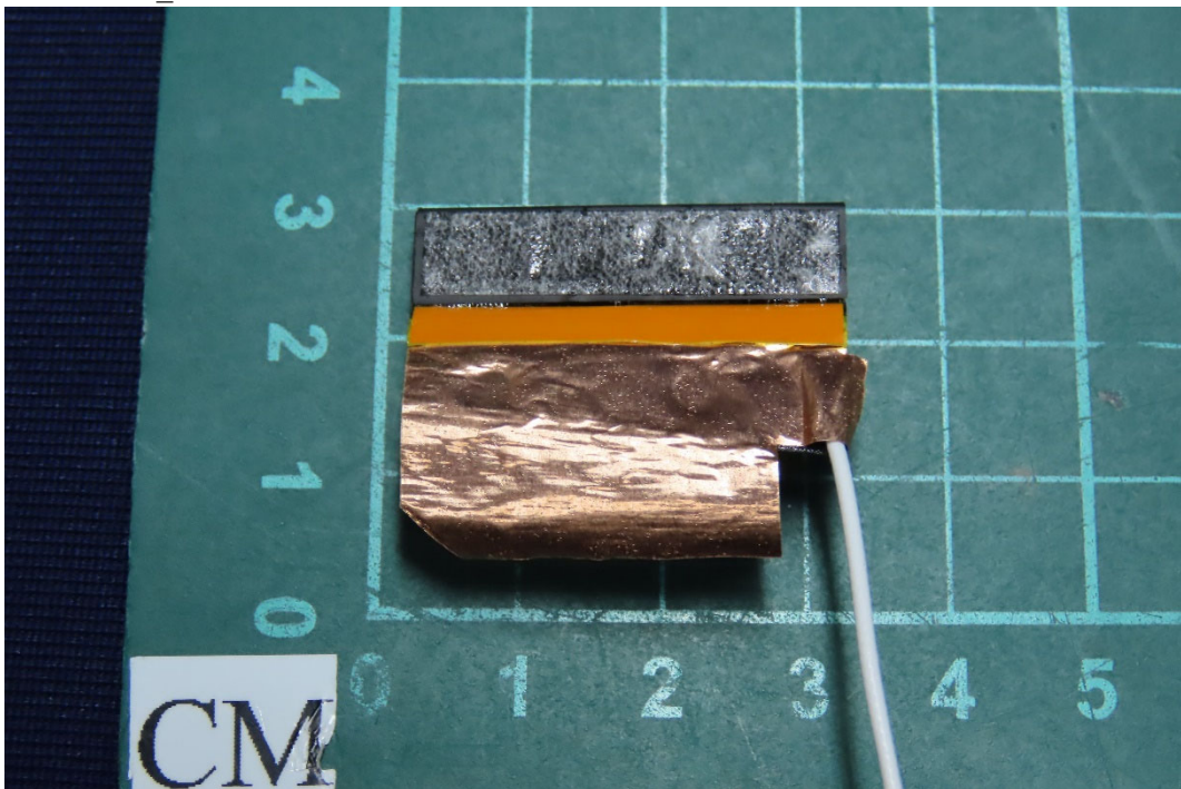
(43) EUT Photo_South Star Aux Antenna
