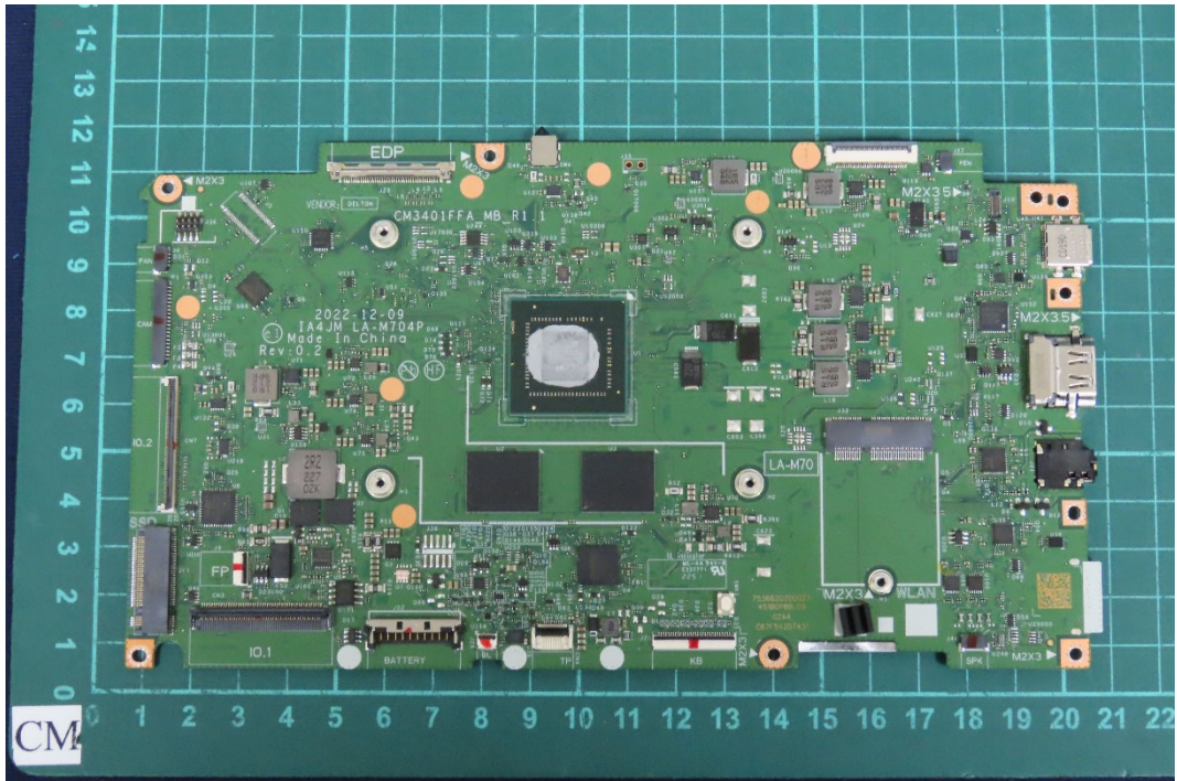
(34) EUT Photo
