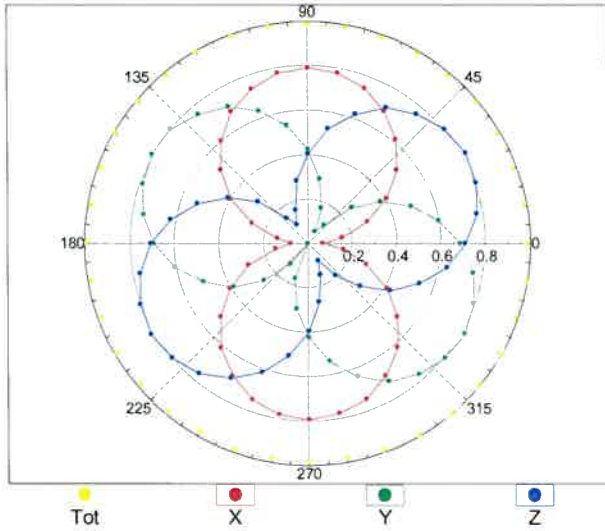
f=600 MHz,TEM
