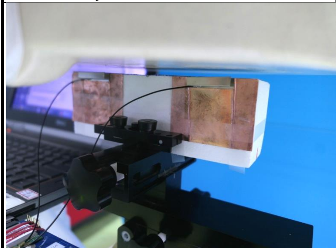
Body - Top Side of EUT at 5 mm
