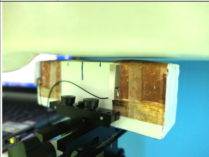
Body - Right Side of EUT at 5 mm
