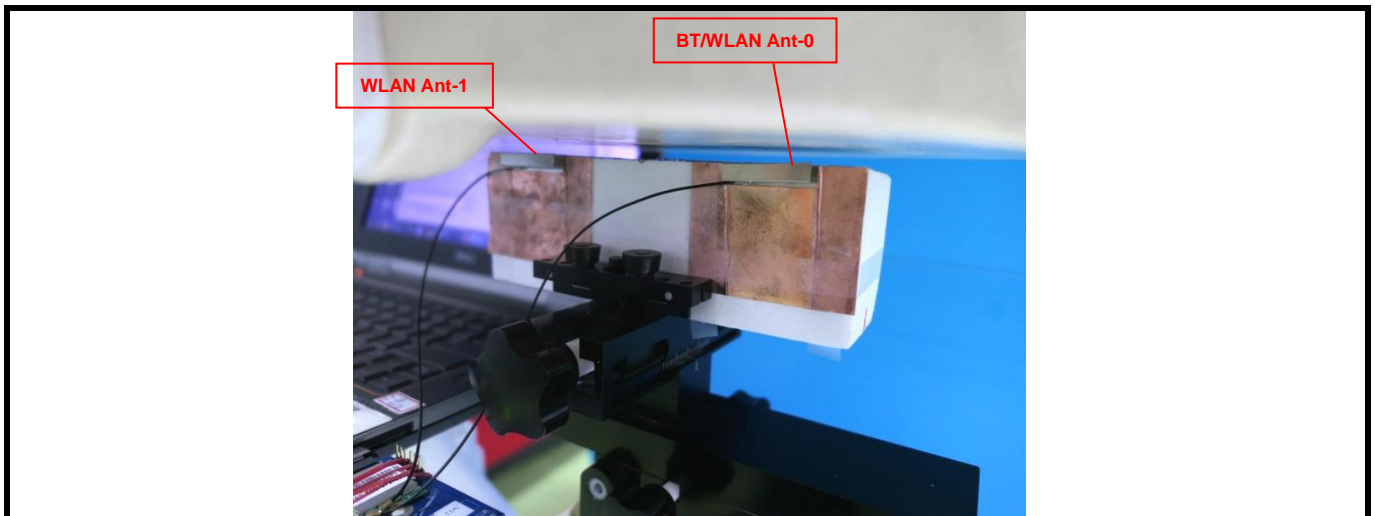
Antenna for Module Port
