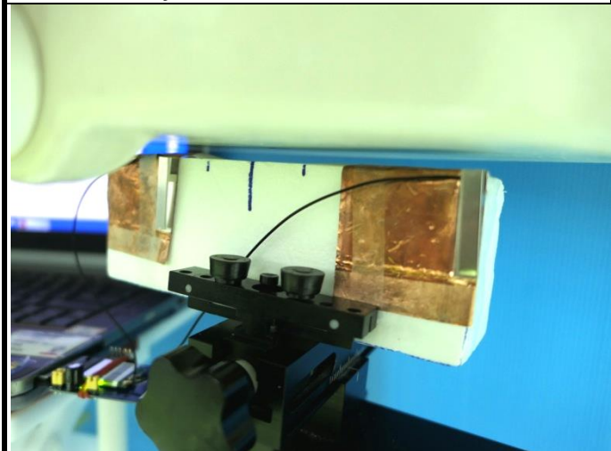
Body - Left Side of EUT at 5 mm
