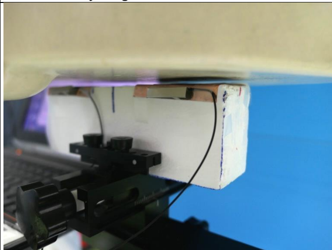
Body - Bottom Side of EUT at 5 mm
