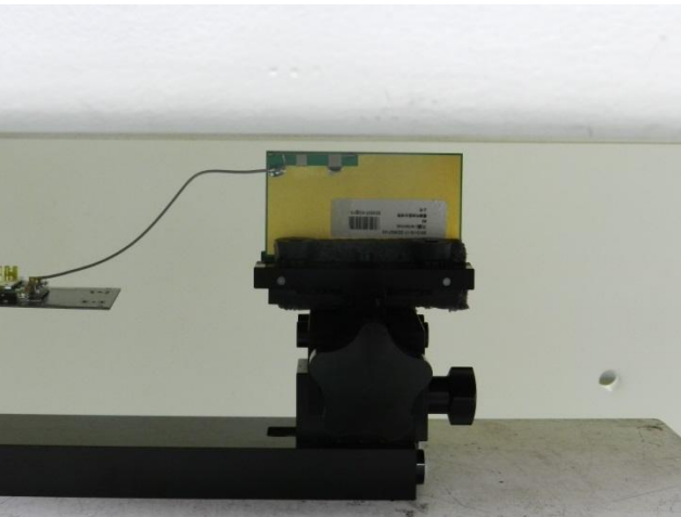
Right Side, Test Separation 0.5 cm Gap
