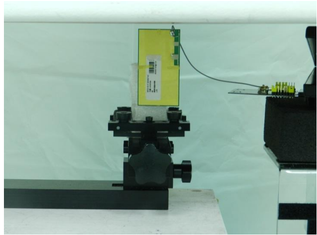
Bottom Side, Test Separation 0.5 cm Gap
