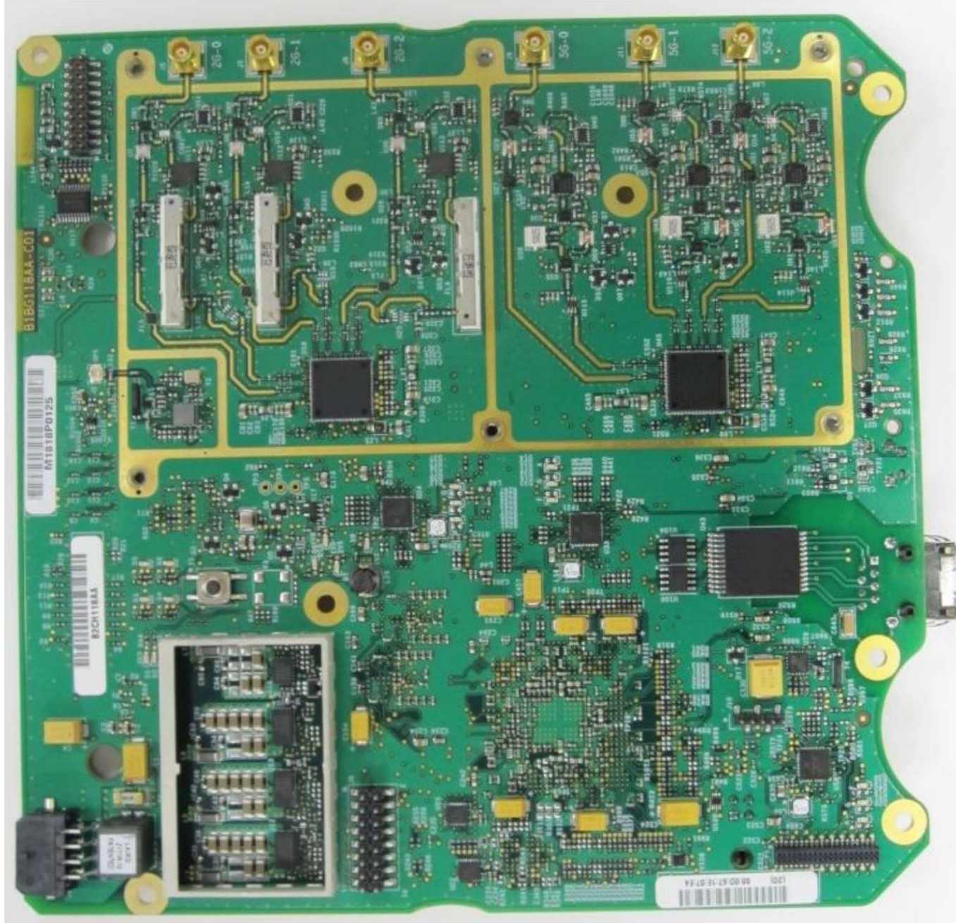
B2CH118AA Primary Side with No Shields
