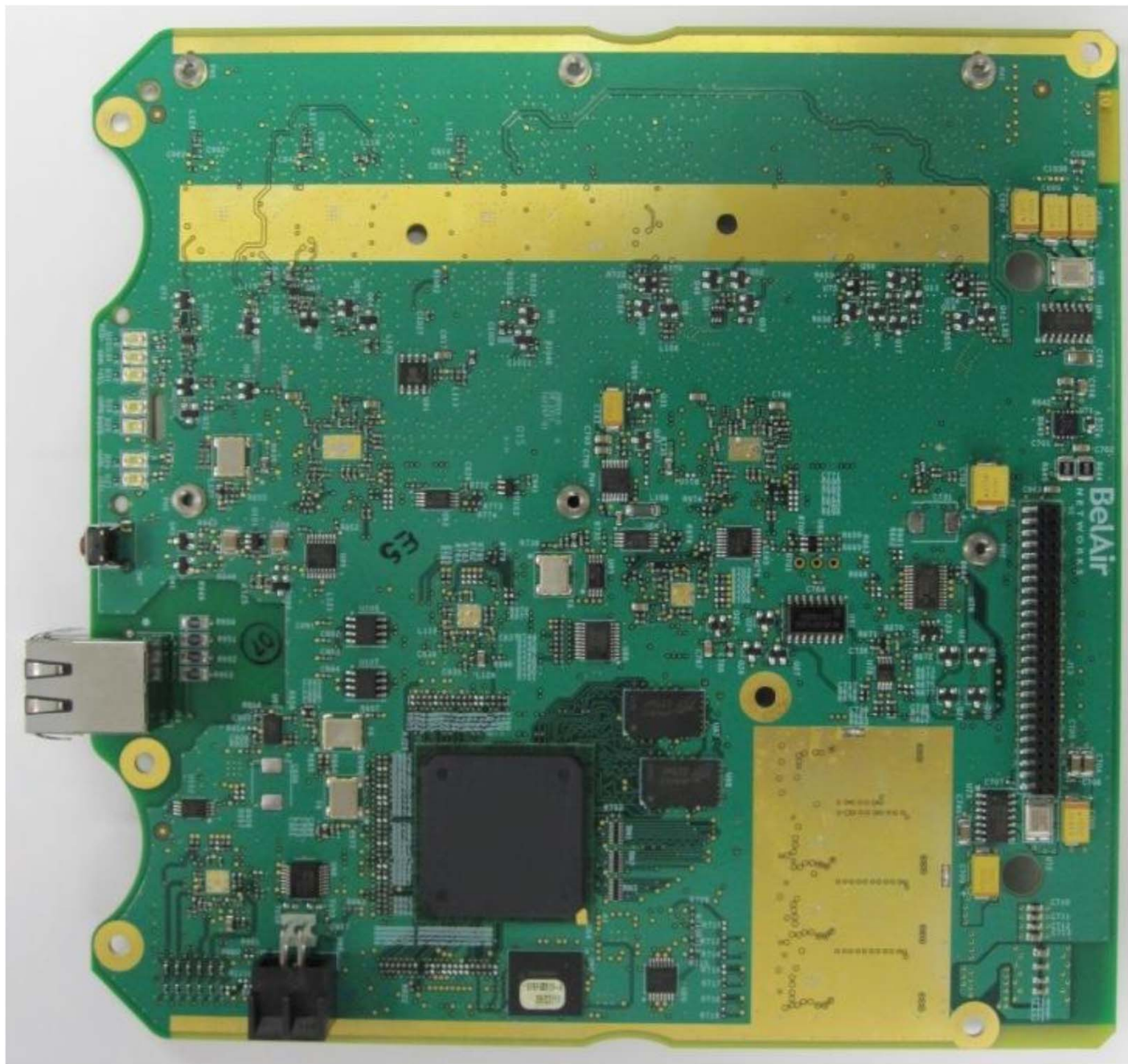
B2CH118AA Secondary Side
