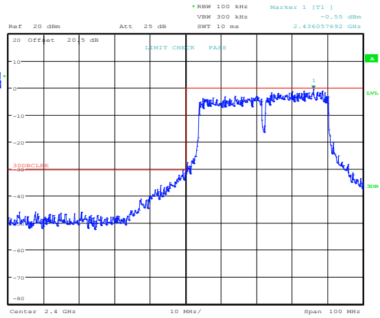
Figure 8.5-30: Conducted lower band edge for 802.11g, ch1
