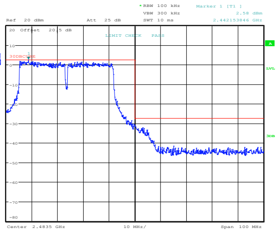
Figure 8.5-34: Conducted upper band edge for 802.11g, cho
