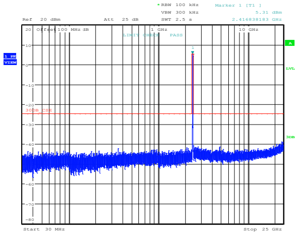
Figure 8.5-1: Conducted spurious emissions for 802.11b, ch0, low channel
