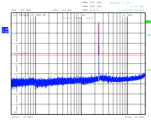
Figure 8.5-5: Conducted spurious emissions for 802.11b, ch0, mid channel
