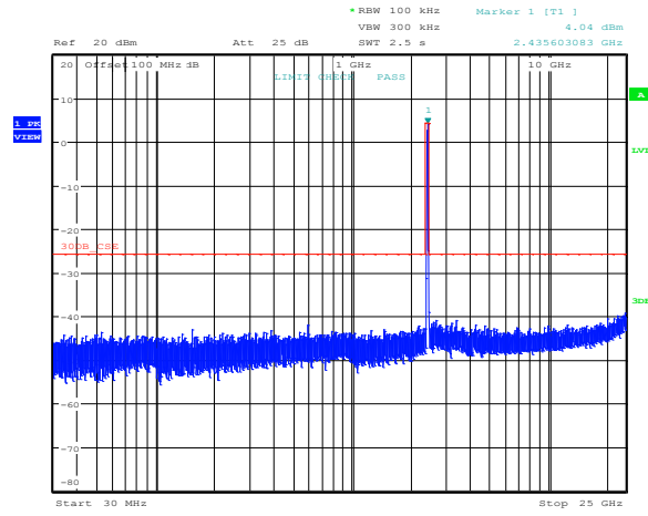
Figure 8.5-2: Conducted spurious emissions for 802.11g, ch0, low channel
