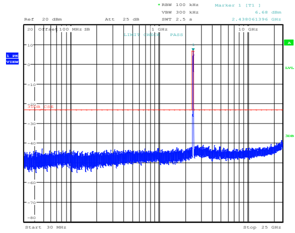
Figure 8.5-6: Conducted spurious emissions for 802.11g, ch0, mid channel
