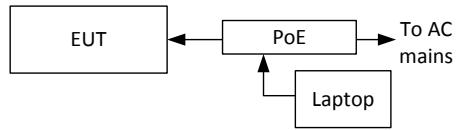
Figure 3.6-1: Setup diagram
