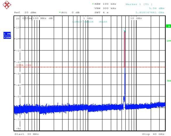
Figure 8.5-24: Conducted spurious emissions outside restricted bands for 802.11n HT40, cho, mid channel
