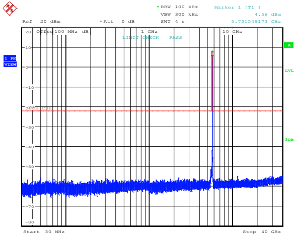
Figure 8.5-27: Conducted spurious emissions outside restricted bands for 802.11n HT40, cho, high channel
