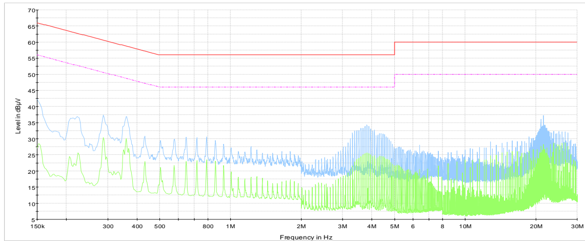
Conducted emissions on neutral line — CISPR 22 Mains QP Class B - - - CISPR 22 Mains AV Class B — Preview Result 1-PK+ — Preview Result 2-AVG
