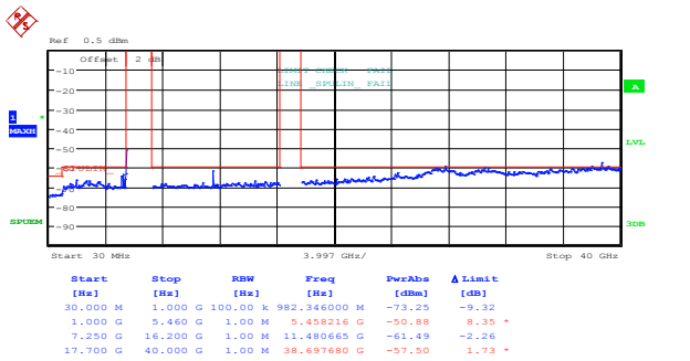
Figure 8.5-1: Conducted peak spurious emissions within restricted bands for 802.11a, cho, low channel
