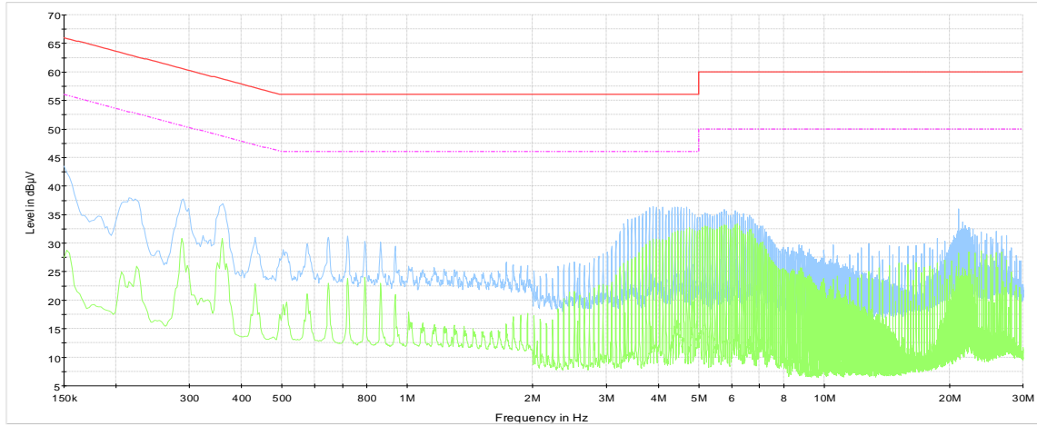
Conducted emissions on phase line — CISPR 22 Mains QP Class B - - - CISPR 22 Mains AV Class B — Preview Result 1-PK+ — Preview Result 2-AVG
