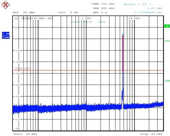
Figure 8.5-31: Conducted spurious emissions outside restricted bands for 802.11a, ch1, mid channel
