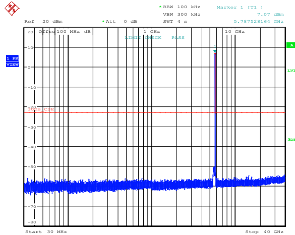
Figure 8.5-20: Conducted spurious emissions outside restricted bands for 802.11n HT20, cho, low channel
