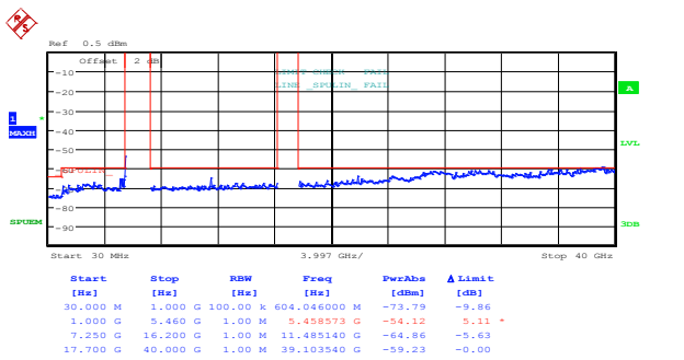
Figure 8.5-3: Conducted peak spurious emissions within restricted bands for 802.11n HT40, cho, low channel
