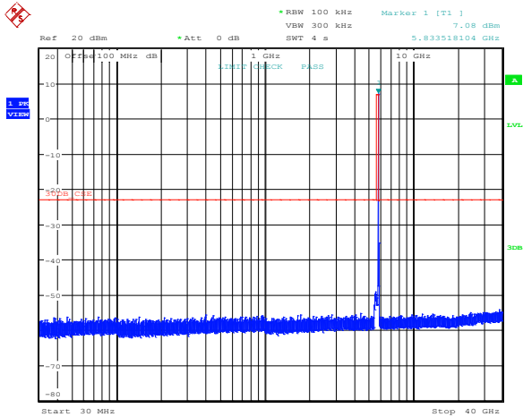
Figure 8.5-23: Conducted spurious emissions outside restricted bands for 802.11n HT20, cho, mid channel
