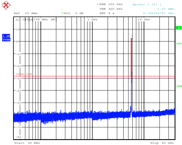
Figure 8.5-19: Conducted spurious emissions outside restricted bands for 802.11a, cho, low channel
