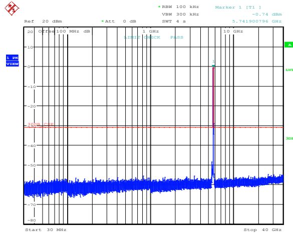
Figure 8.5-28: Conducted spurious emissions outside restricted bands for 802.11a, ch1, low channel
