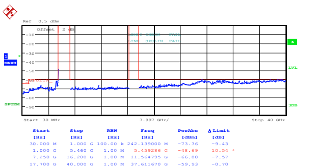
Figure 8.5-5: Conducted peak spurious emissions within restricted bands for 802.11n HT20, cho, mid channel
