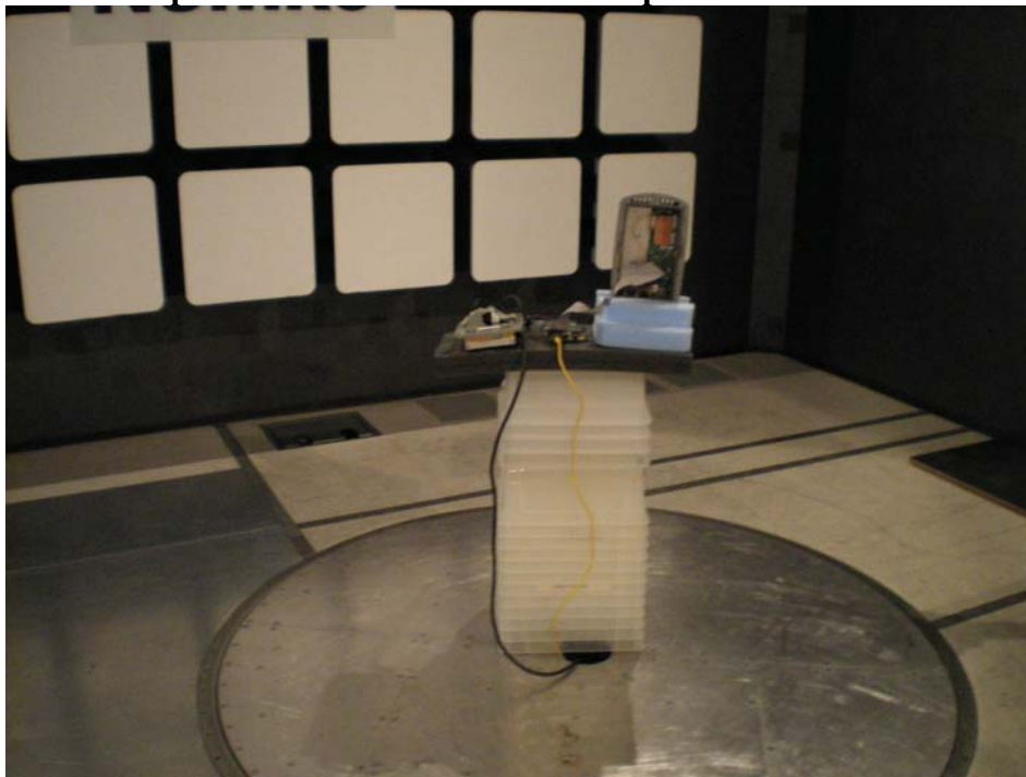
Radiated Spurious Emissions > 1GHz Setup:
