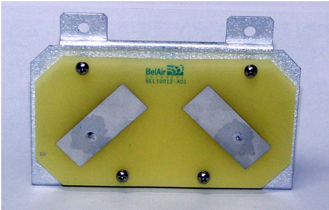
8dBI Access Antenna BEL10012-A01_Front_02
