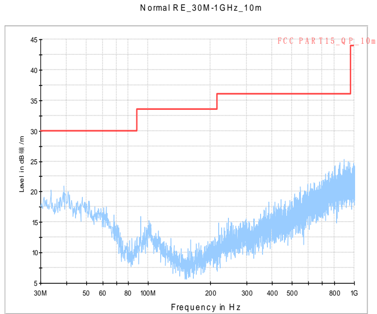
Fig.24. Radiated emission: GFSK, 2480MHz, 30 MHz - 1 GHz
