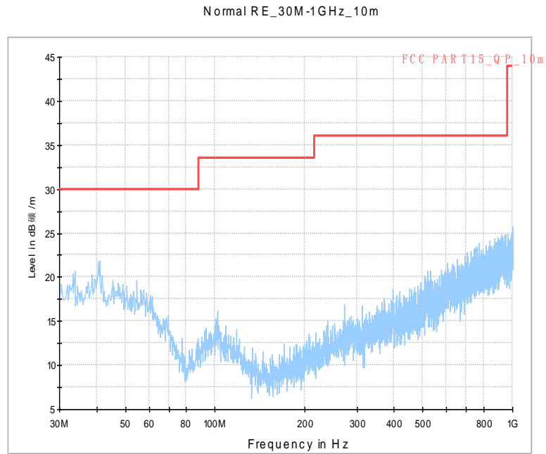
Fig.18. Radiated emission: GFSK, 2402MHz, 30 MHz - 1 GHz
