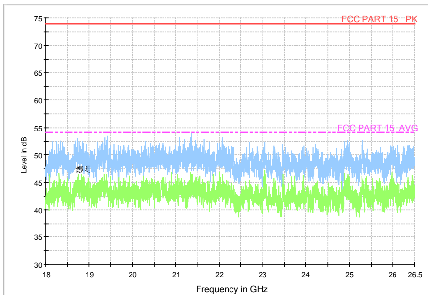
Normal RE_18G-26.5GHz
