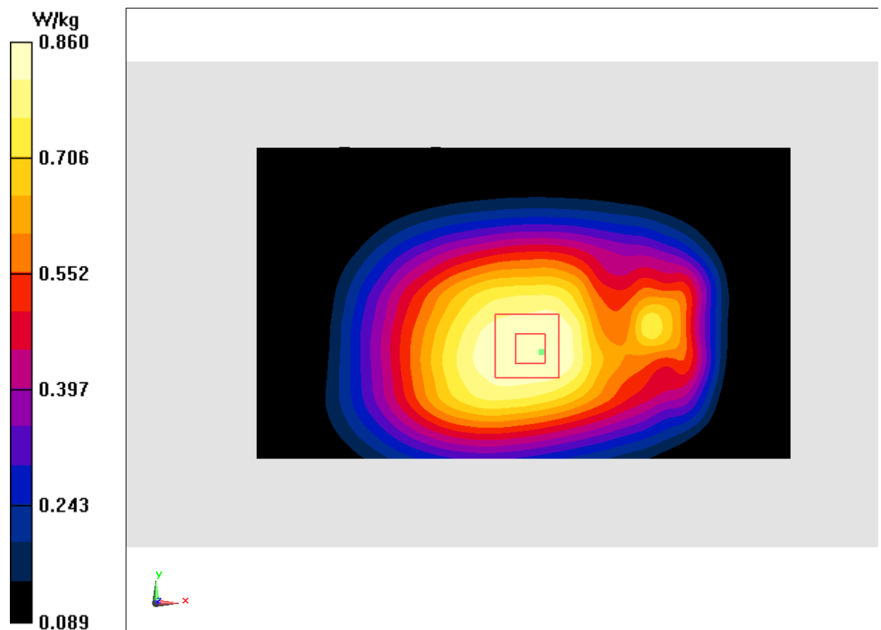
Fig.2 850 MHz
