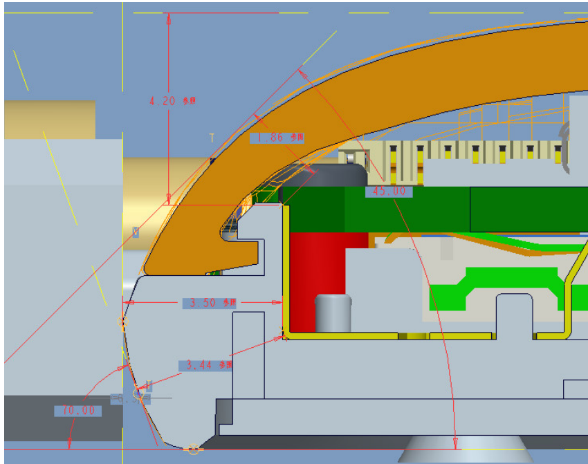
X =3.50mm, Y=4.20mm, Z=1.86mm for WWAN
