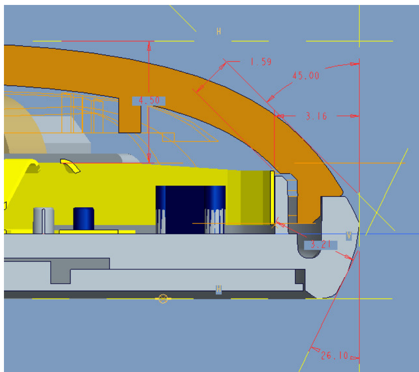
X =3.16mm, Y=4.50mm, Z=1.59mm for WLAN
