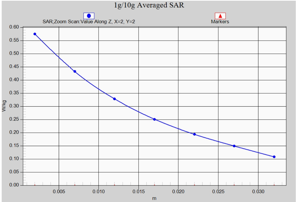
Fig. 14-1 Z-Scan at power reference point (LTE Band17)
