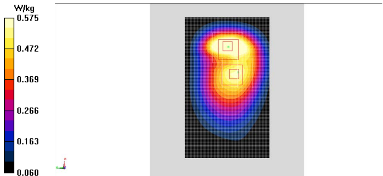
Fig.14 LTE Band17
