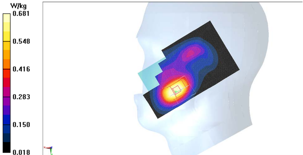
Fig.9 LTE Band4
