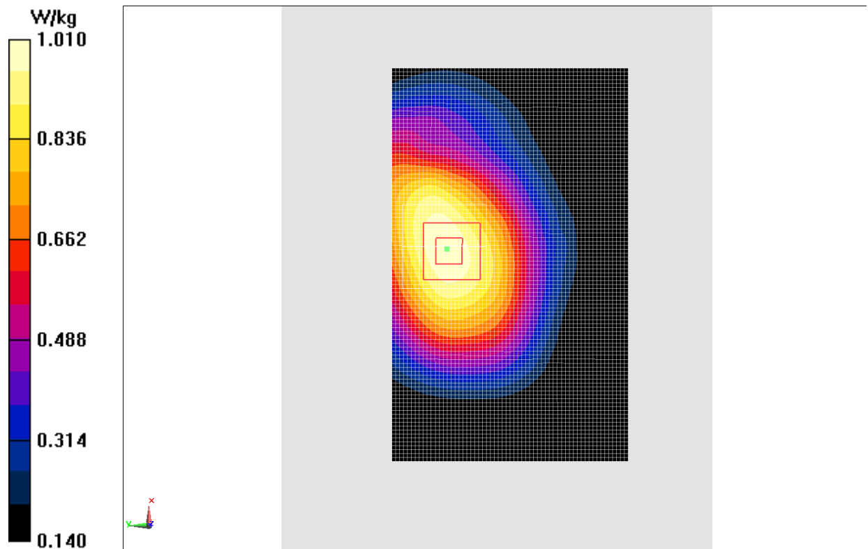
Fig.2 850 MHz
