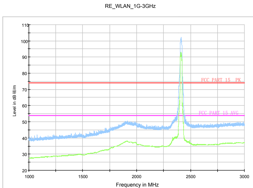
Fig.A.6.23 Transmitter Spurious Emission - Radiated (802.11n-HT20, Ch1, 1 GHz-3 GHz)
