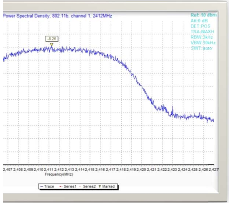
Fig.A.3.1 Power Spectral Density(802.11b,Ch1)
