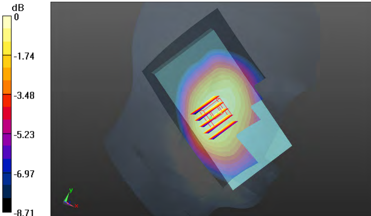
0 dB = 0.238 W/kg
