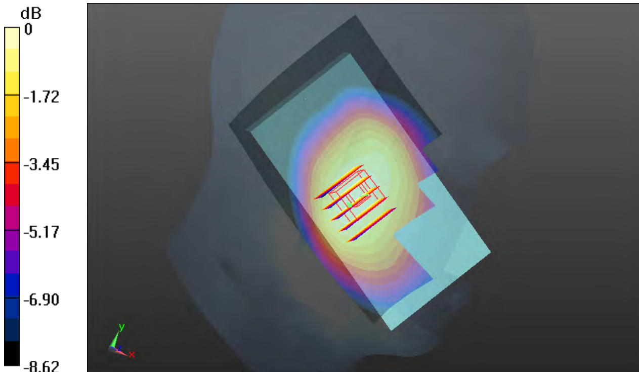
0 dB = 0.271 W/kg
