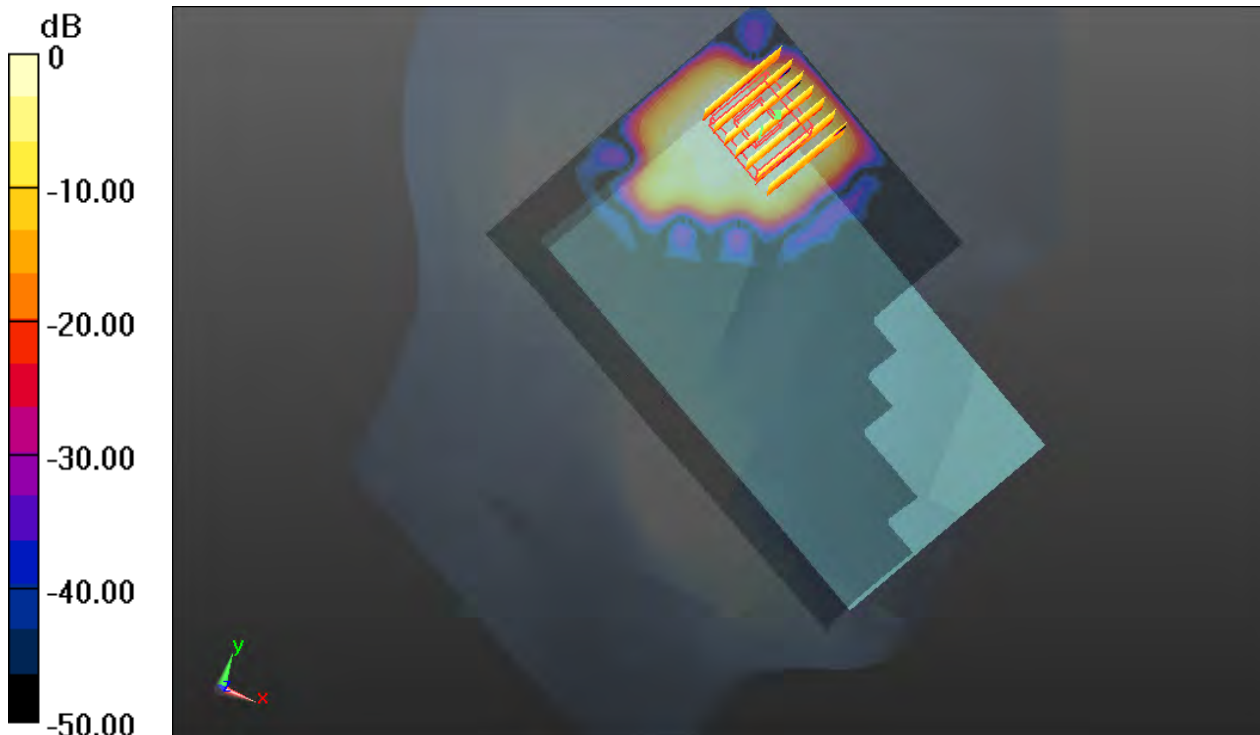
0 dB = 0.0822 W/kg
