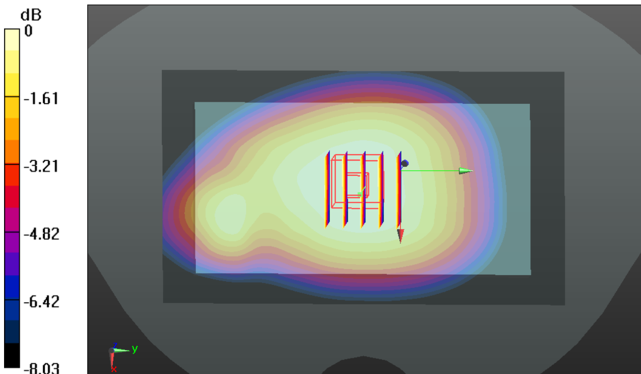
0 dB = 0.362 W/kg
