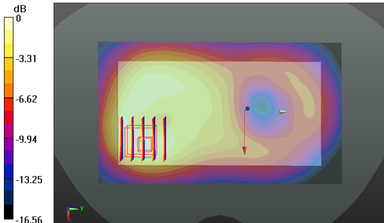
0 dB = 0.665 W/kg
