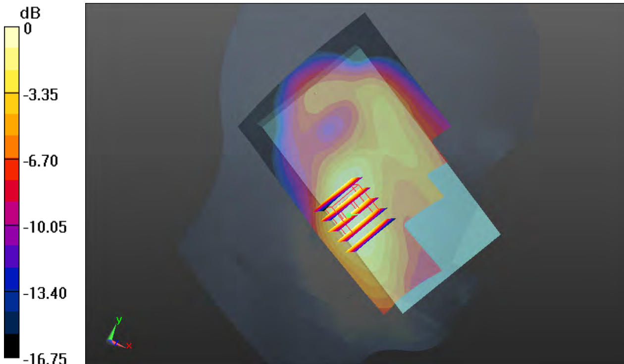
0 dB = 0.219 W/kg
