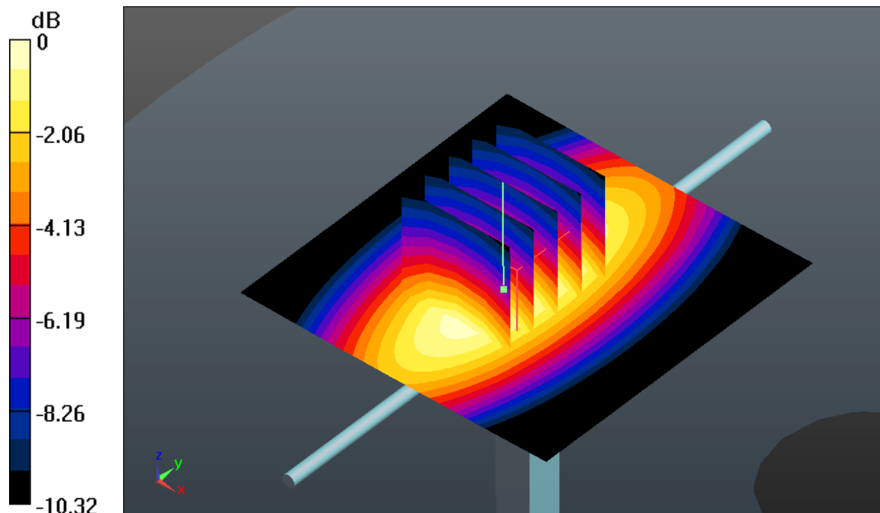
0 dB = 2.51 W/kg
