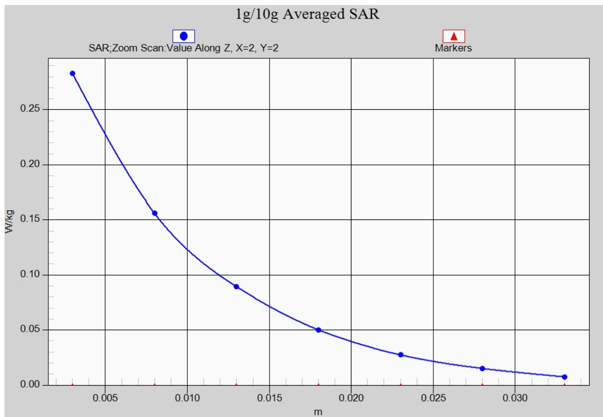
Fig. 12-1 Z-Scan at power reference point (2450 MHz)
