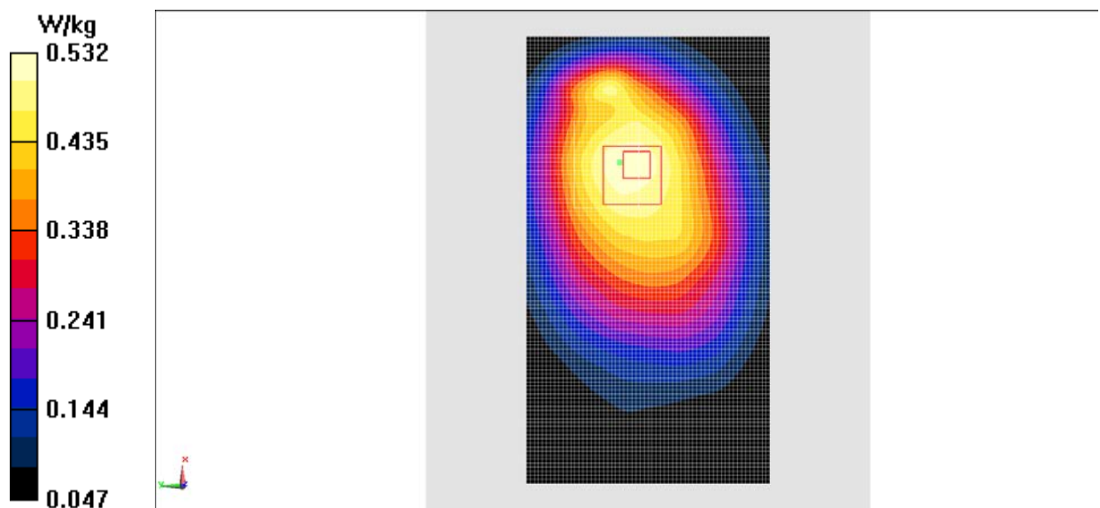
Fig.8 LTE Band5
