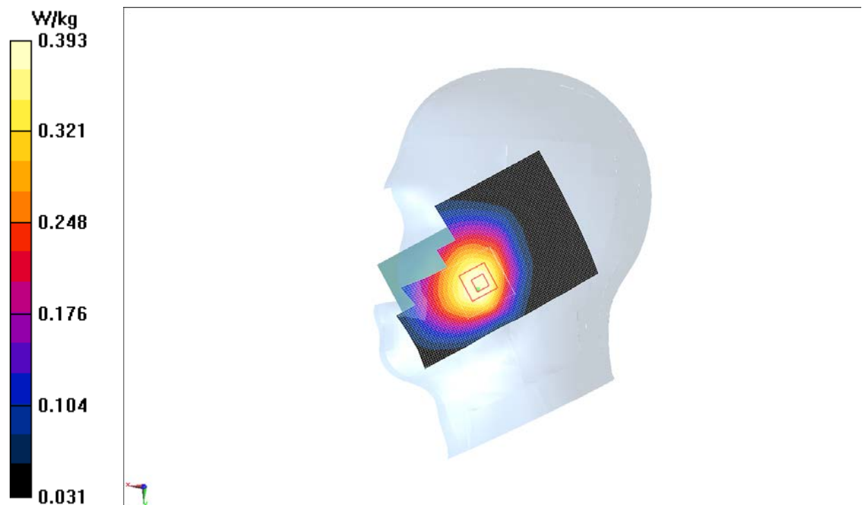
Fig.7 LTE Band5
