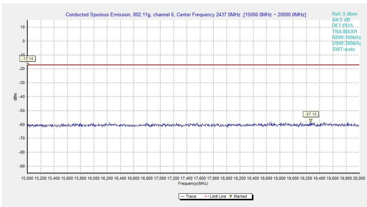
Fig.A.6.1.55 Transmitter Spurious Emission - Conducted (802.11g, Ch6, 15 GHz-20 GHz)
