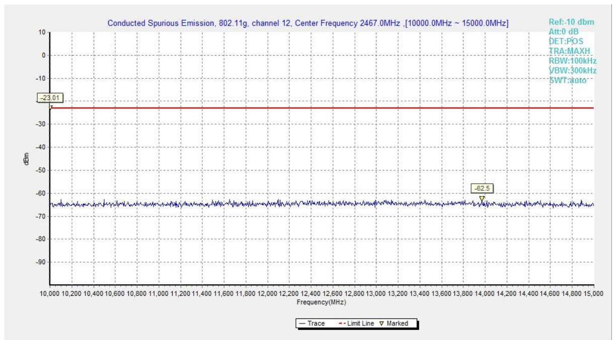
Fig.A.6.1.70 Transmitter Spurious Emission - Conducted (802.11g, Ch12, 10 GHz-15 GHz)
