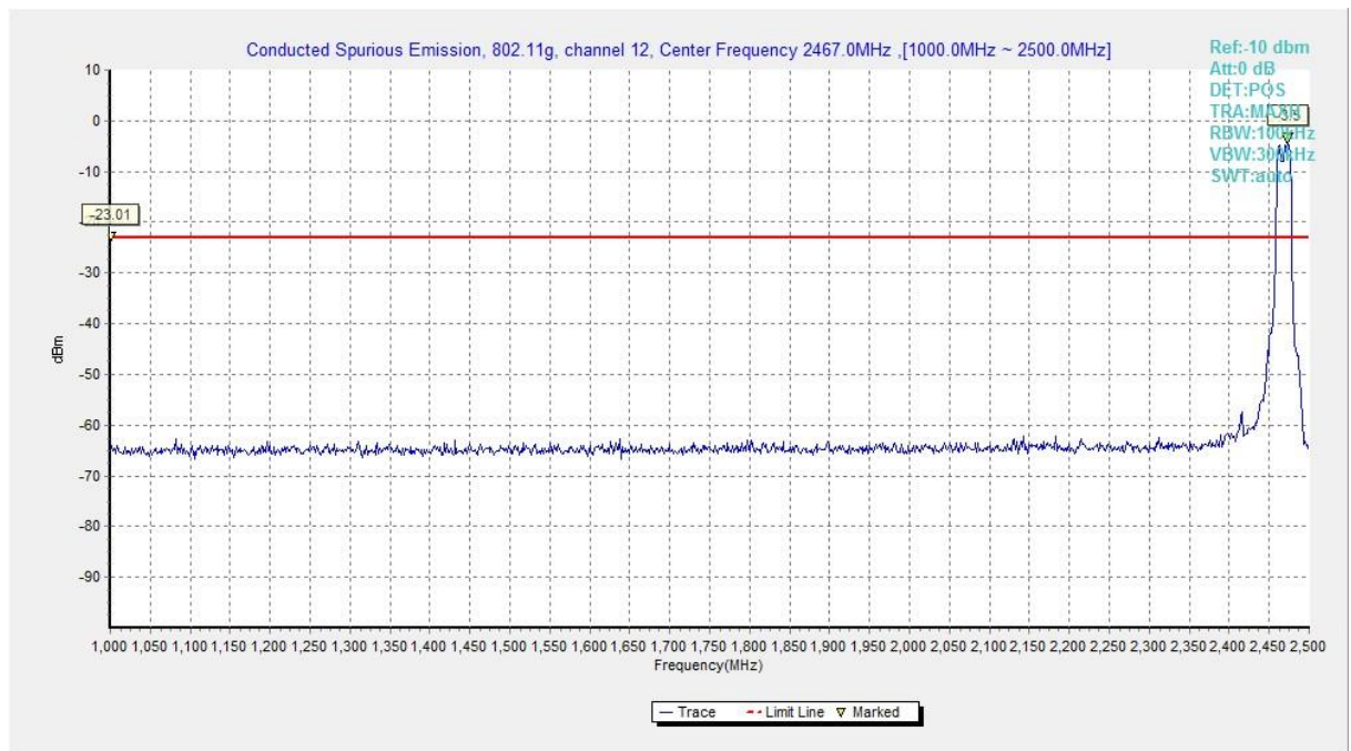
Fig.A.6.1.67 Transmitter Spurious Emission - Conducted (802.11g, Ch12, 1 GHz-2.5 GHz)
