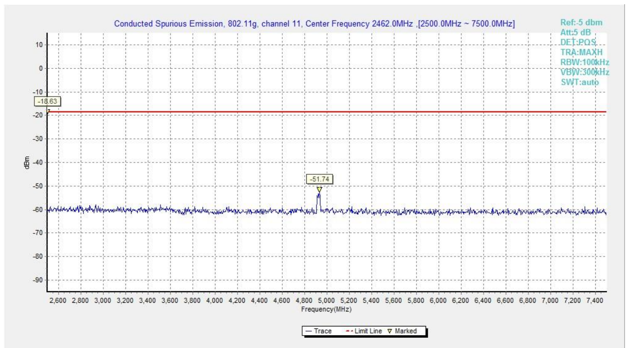
Fig.A.6.1.60 Transmitter Spurious Emission - Conducted (802.11g, Ch11, 2.5 GHz-7.5 GHz)
