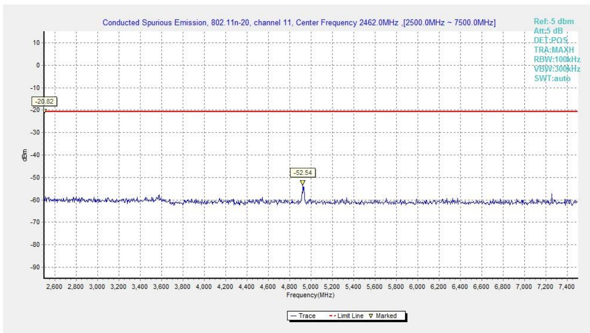
Fig.A.6.1.100 Transmitter Spurious Emission - Conducted (802.11n-HT20, Ch11, 2.5 GHz-7.5 GHz)
