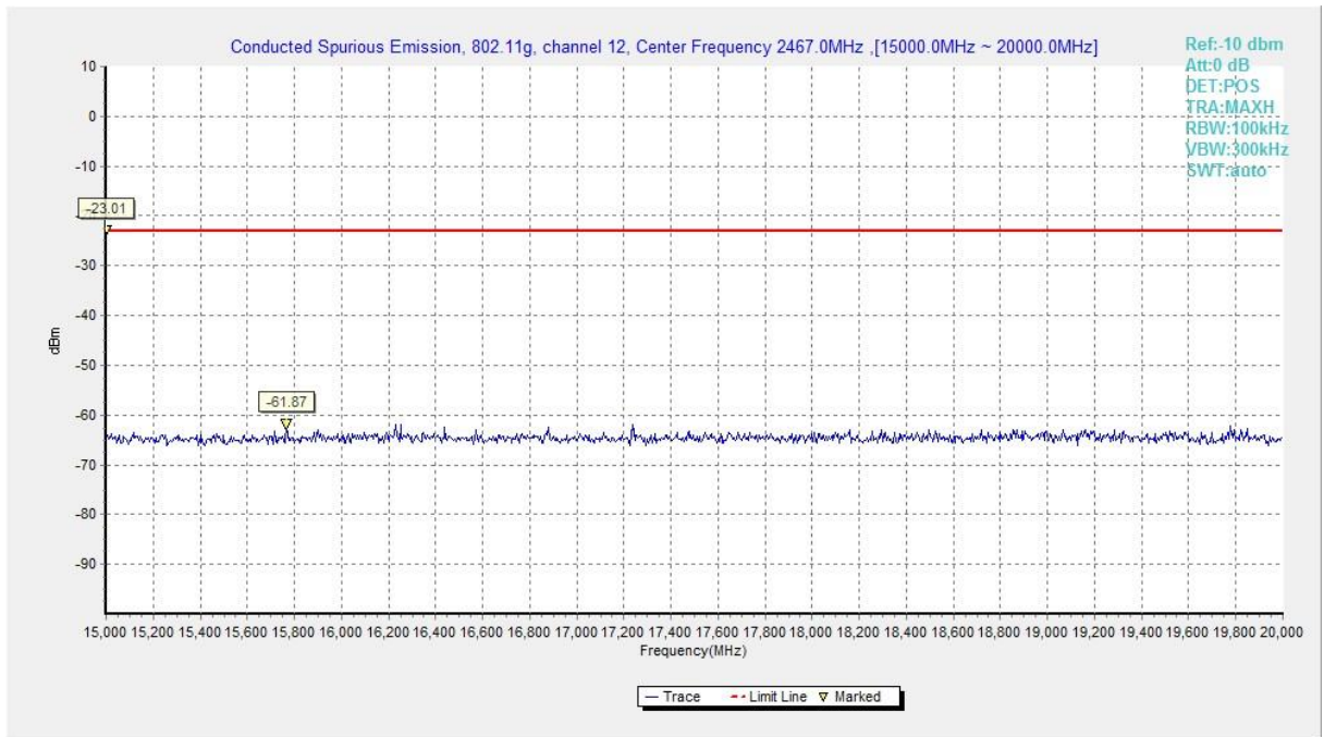
Fig.A.6.1.71 Transmitter Spurious Emission - Conducted (802.11g, Ch12, 15 GHz-20 GHz)
