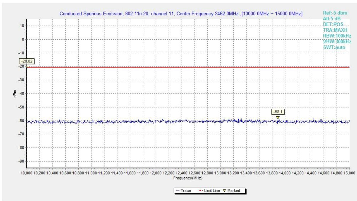
Fig.A.6.1.102 Transmitter Spurious Emission - Conducted (802.11n-HT20, Ch11, 10 GHz-15 GHz)
