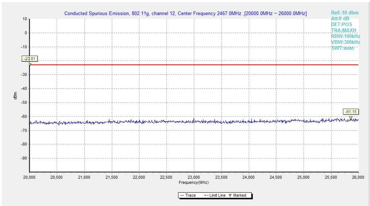
Fig.A.6.1.72 Transmitter Spurious Emission - Conducted (802.11g, Ch12, 20 GHz-26 GHz)
