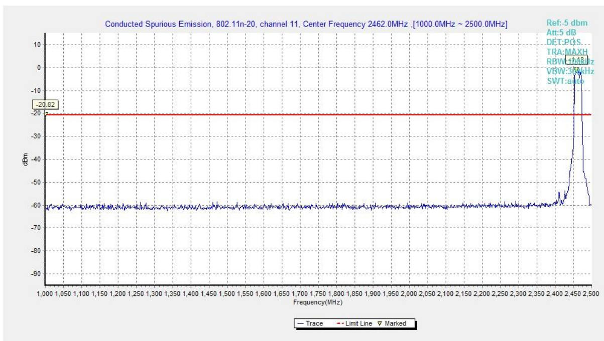
Fig.A.6.1.99 Transmitter Spurious Emission - Conducted (802.11n-HT20, Ch11, 1 GHz-2.5 GHz)
