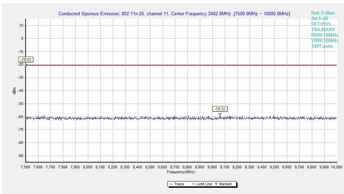
Fig.A.6.1.101 Transmitter Spurious Emission - Conducted (802.11n-HT20, Ch11, 7.5 GHz-10 GHz)
