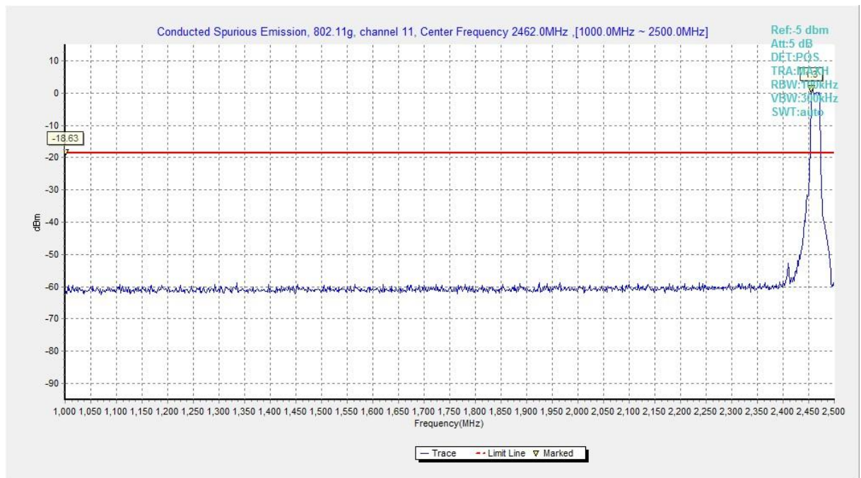
Fig.A.6.1.59 Transmitter Spurious Emission - Conducted (802.11g, Ch11, 1 GHz-2.5 GHz)
