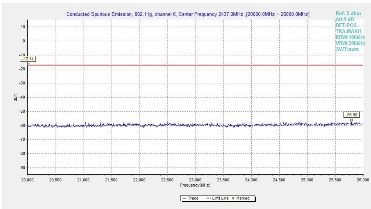
Fig.A.6.1.56 Transmitter Spurious Emission - Conducted (802.11g, Ch6, 20 GHz-26 GHz)
