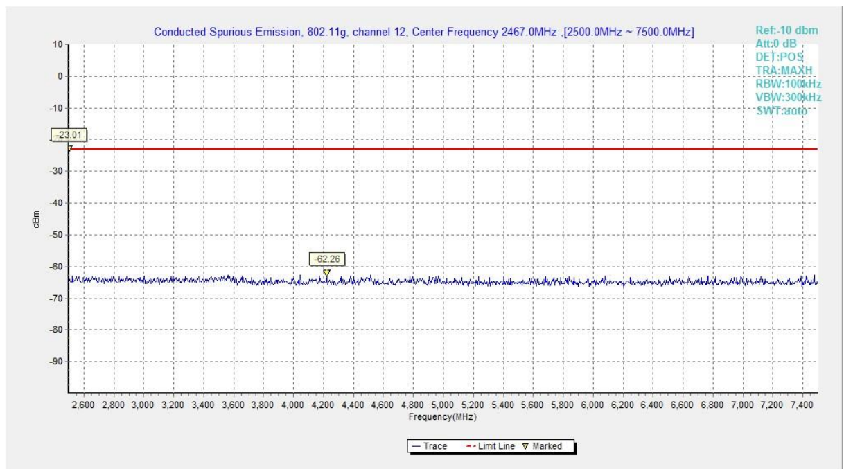
Fig.A.6.1.68 Transmitter Spurious Emission - Conducted (802.11g, Ch12, 2.5 GHz-7.5 GHz)
