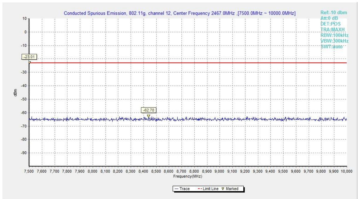
Fig.A.6.1.69 Transmitter Spurious Emission - Conducted (802.11g, Ch12, 7.5 GHz-10 GHz)
