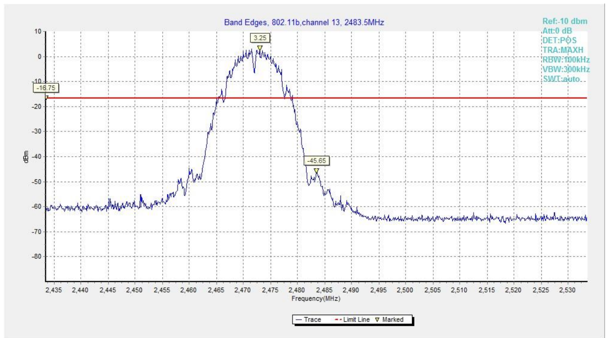
Fig.A.5.3 Band Edges (802.11b, Ch 13)
