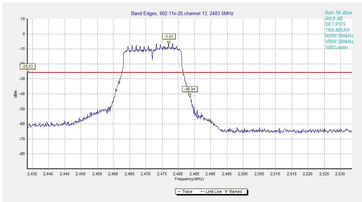
Fig.A.5.9 Band Edges (802.11n-HT20, Ch 13)
