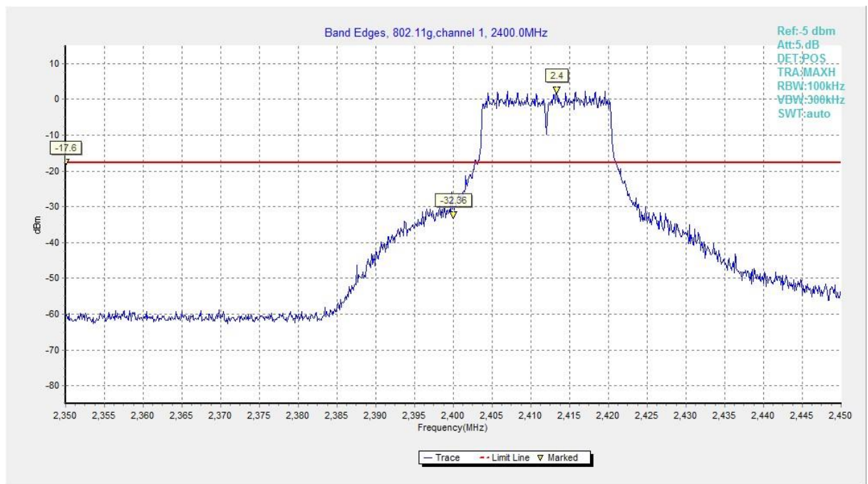
Fig.A.5.4 Band Edges (802.11g, Ch 1)
