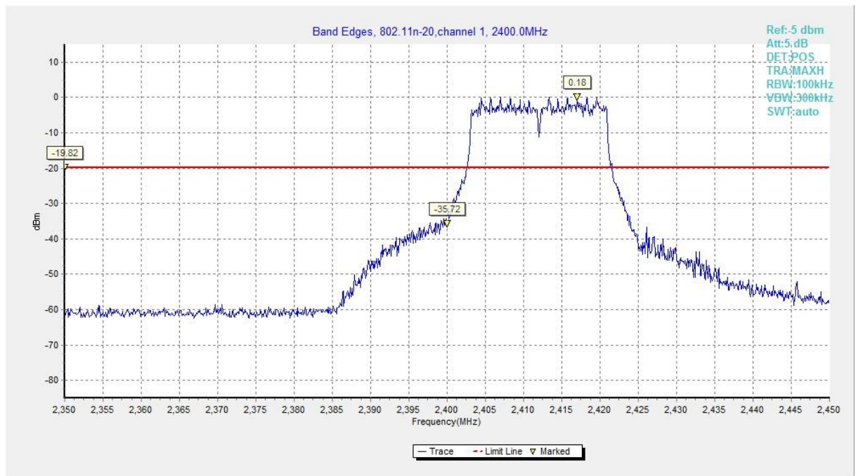
Fig.A.5.7 Band Edges (802.11n-HT20, Ch 1)
