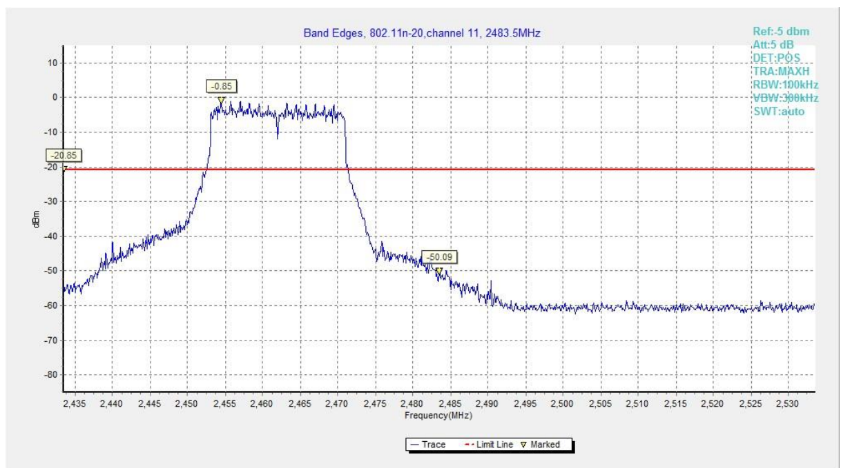
Fig.A.5.8 Band Edges (802.11n-HT20, Ch 11)
