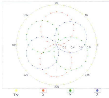
f=600 MHz,TEM
